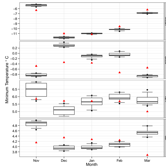
(c) Min temperature
