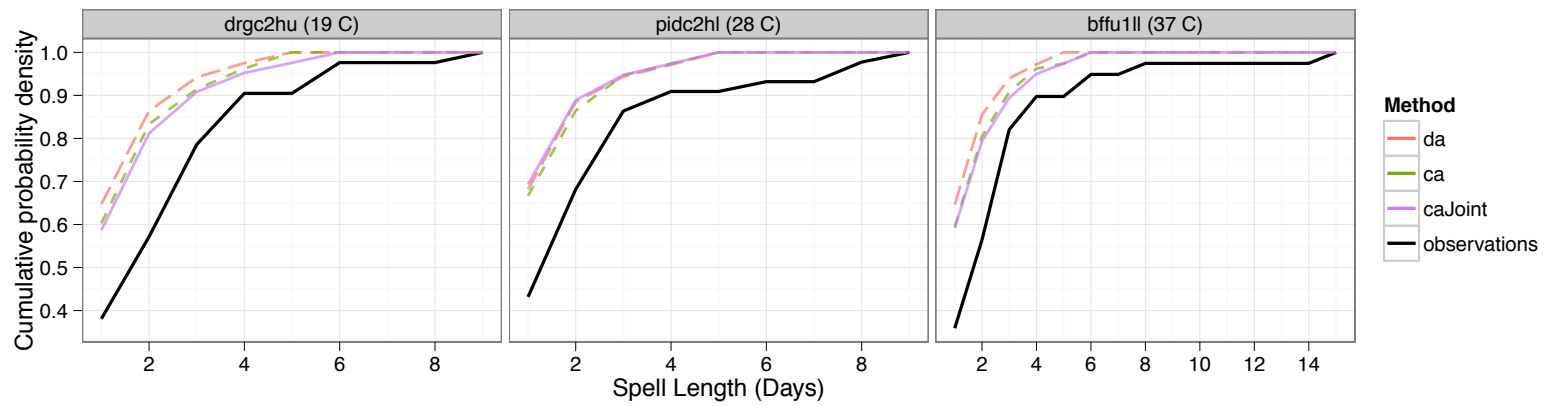
(b) JJA spells above 99th percentile
