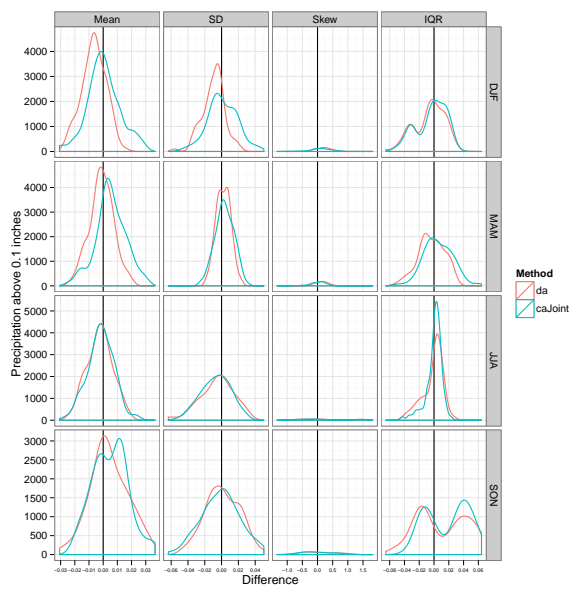
Figure 2.12: Distribution (over all simulations) of differences between observed and simulated statistics of precipitation
