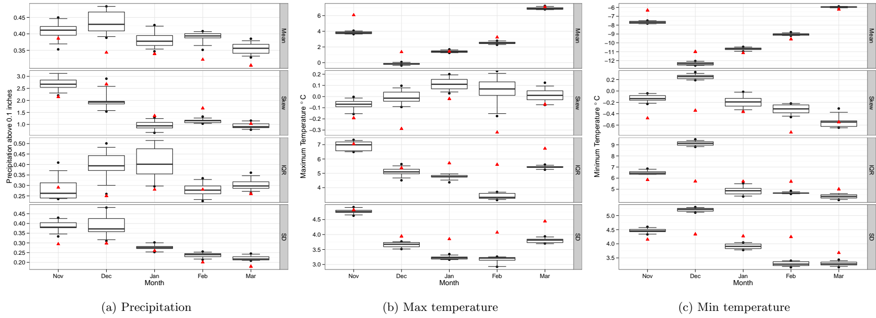
Figure B.3: Distributional statistics of daily weather variables for ANB of 40:35:25
