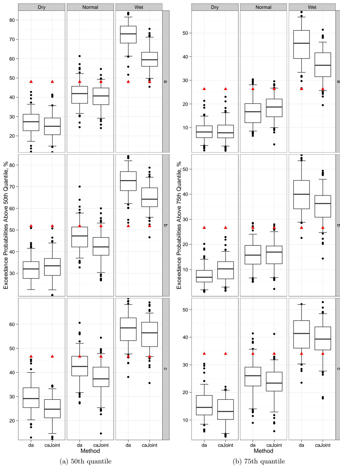
Figure 2.22: Same as Figure 2.21 for MAM
