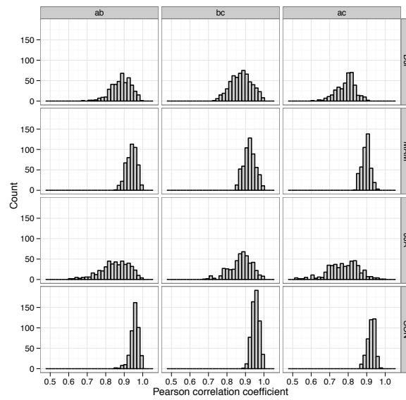
Figure 2.5: Histograms of between-cluster correlations in the observed data for all stations in each pair of clusters
