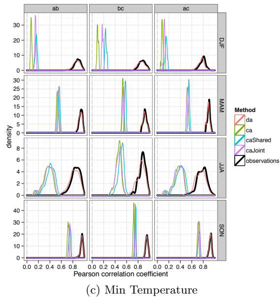
Figure 2.9: Simulated and observed distributions of between-cluster correlations
