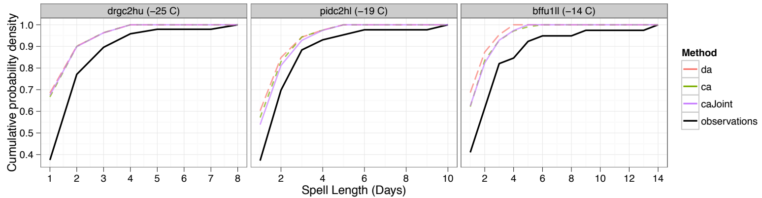
(b) DJF spells below 1st percentile
