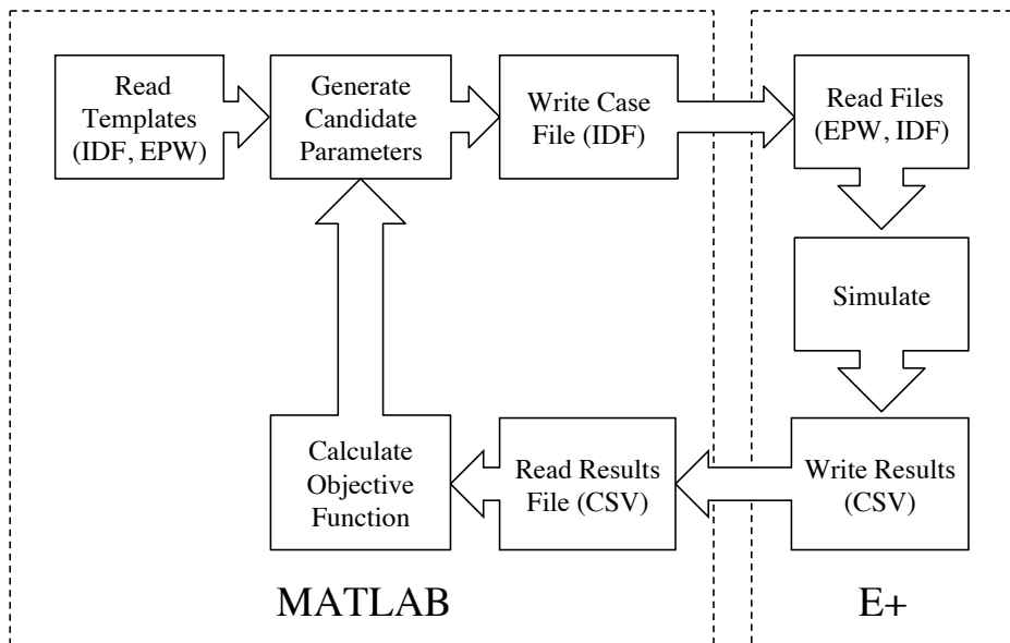
Figure 3.2: The ME+ environment, coupling Matlab and EnergyPlus.
