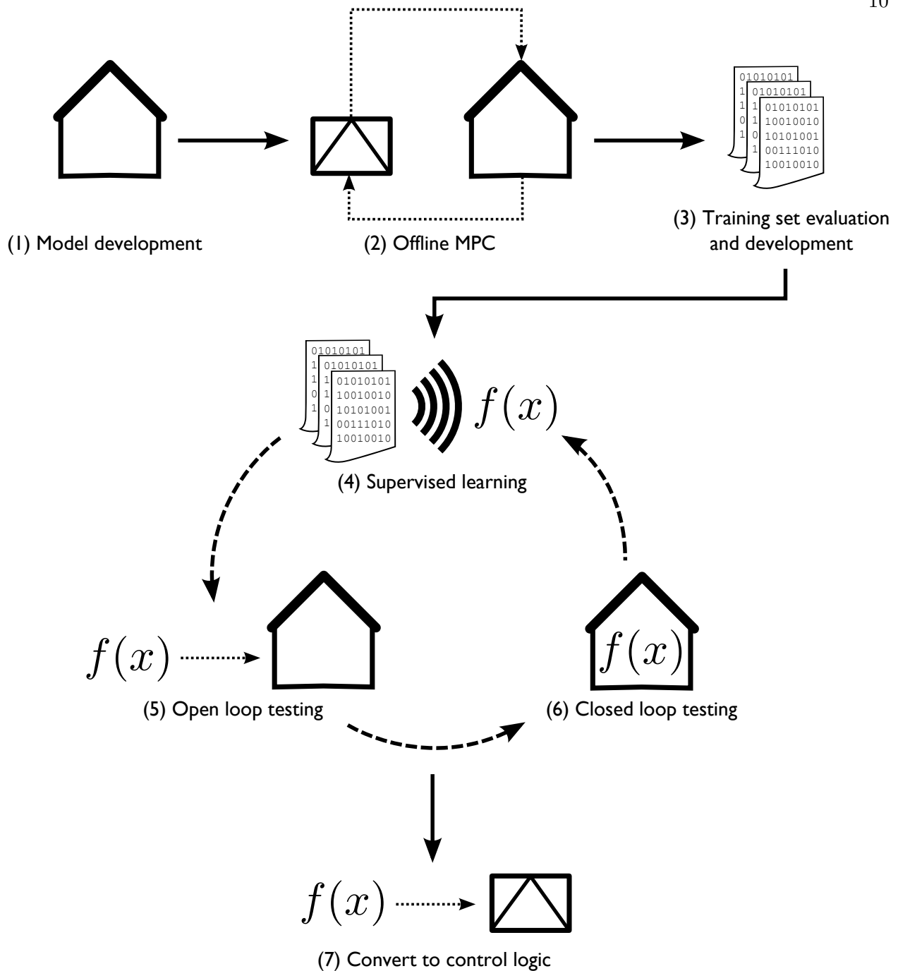
Figure 1.4: Rule extraction proceeds in a seven-step process. In steps 1 through 3, a building energy model is developed and offline MPC is used to develop a training set of optimal solutions and corresponding building states. Supervised learning techniques are used to directly generate the control rule in step 4. Once a rule is trained, performance is tested to examine the skill of the rule in reproducing optimal behavior, seen in steps 5 and 6. Steps 4 through 6 generally involve some iteration, since it is often necessary to introduce expert knowledge as the solution is better understood. Finally in step 7, the final rule is converted into control logic scripted in an applicable BAS language.
