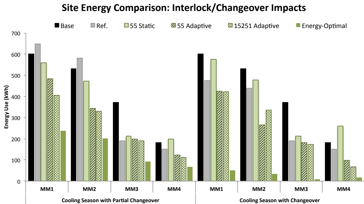
Figure 6.23: Comparison of partial and full changeover operation for buildings MM1–4 during the cooling season week.
