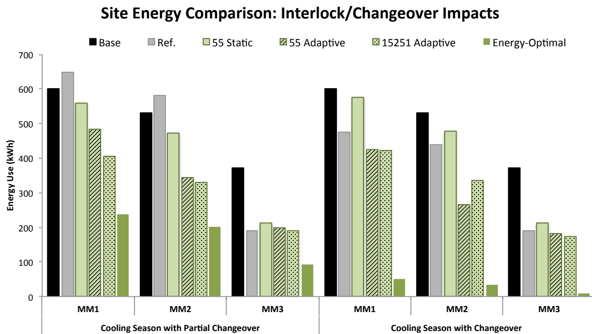
Figure 6.19: Weekly energy use comparison of partial changeover and changeover optimizations for models MM1 through 3. Note that the MM3 reference cases include interlock-enabled changeover by default.
