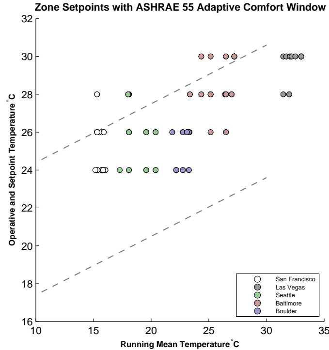
Figure 6.12: MPC-derived setpoints during occupied periods using the ASHRAE 55 adaptive comfort penalty. Setpoints broadly trend with the adaptive comfort window.
