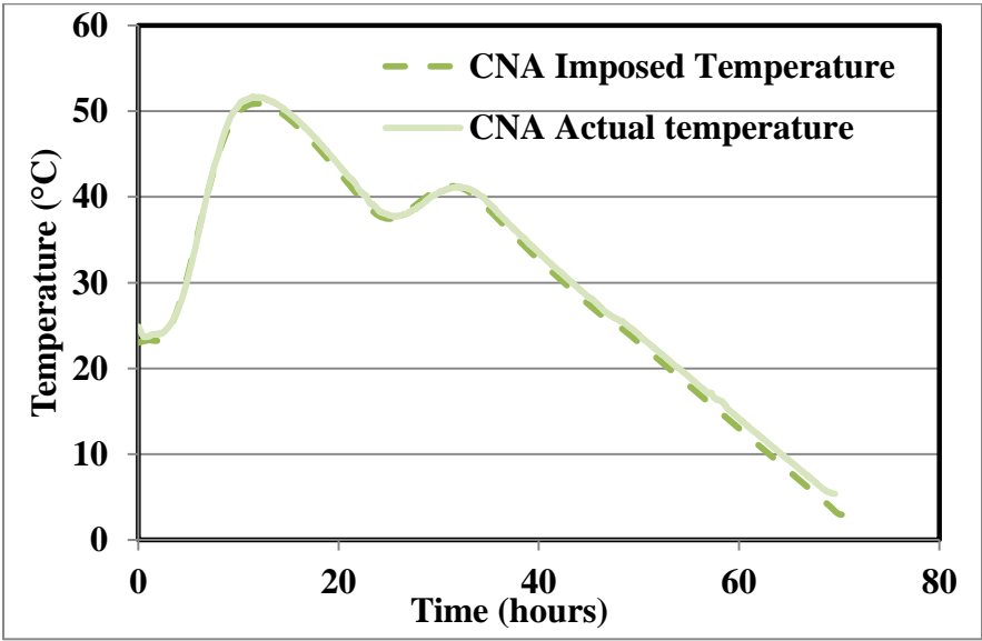
Figure 28 Plot of CNA imposed temperature and the actual recorded temperature in the cracking frame
