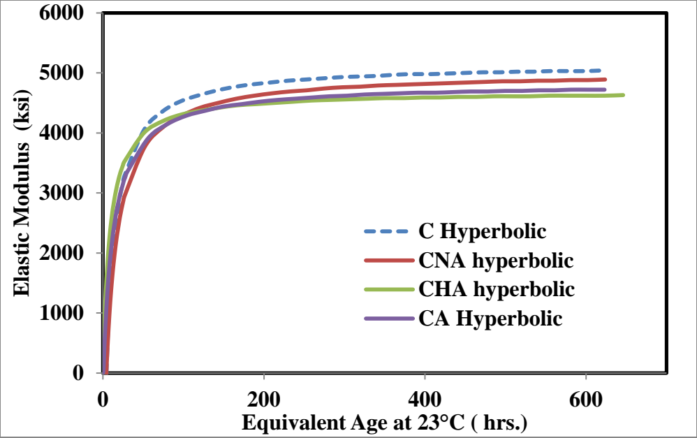
Figure 24 Elastic modulus versus equivalent age
