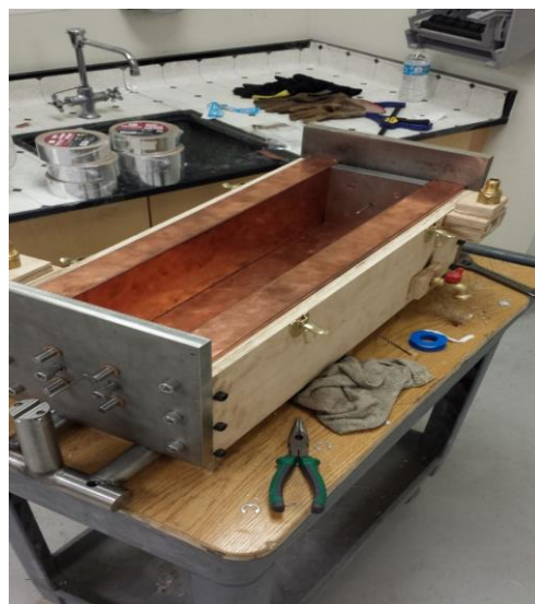
Figure A.9 Finishing touches of the construction of the free shrinkage frame. This includes a drain for easy emptying of the frame and latches for a good seal during operation
