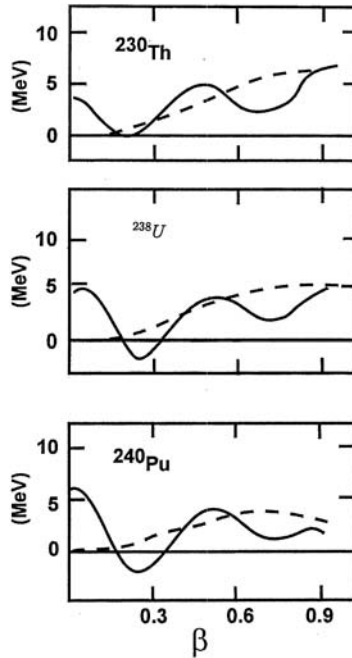
Fig. 8.1. The calculated shell corrected barrier, \Delta W given by (8.2) and the standard liquid drop barrier \Delta W(LDM) given by (8.4) are shown as solid and broken lines respectively, as a function of deformation \beta . This is taken from [8.9]
