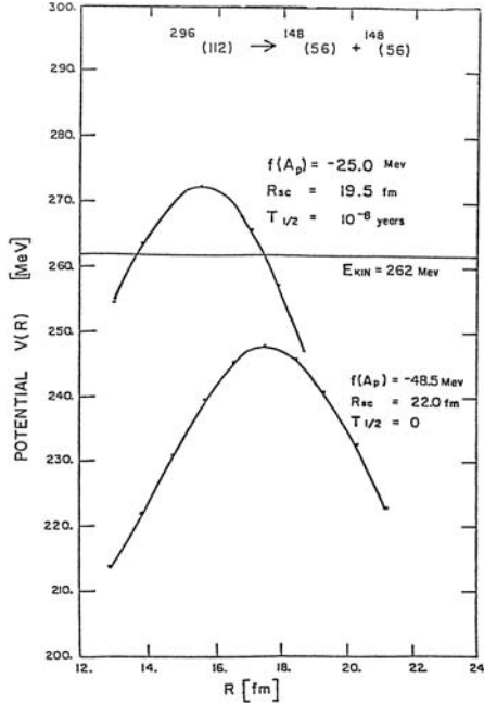
Fig. 4.2. Computed external barrier in the decay of ^{296}(112) to ^{148}(56) and ^{148}(56) for two different scission radii in the spheroid-spheroid model. E_{kin} , calculated from (4.2), is shown as a straight line. f(A_p) is calculated from 4.4 and 4.6 and T_{1/2} is the half-life for the corresponding barrier
