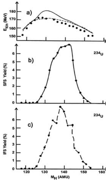
Fig. 8.5. The kinetic energy E_{kin} , and the percentage mass yields spectra for spontaneous fission, SFS yields (%), and isomer fission states, IFS yield (%), of ^{234}\text{U} are shown at the upper, middle and lower inserts, respectively. M_H is atomic mass of the heavy fragments. Solid lines are experimental data of [8.36]. Solid dots in (b) and (c) are calculated percentage mass yields using the kinetic energy spectra shown as broken line in (a). Solid line in (a) is the observed kinetic energy and solid dots in (a) are (Q-values calculated from [8.37] – 16 MeV)
