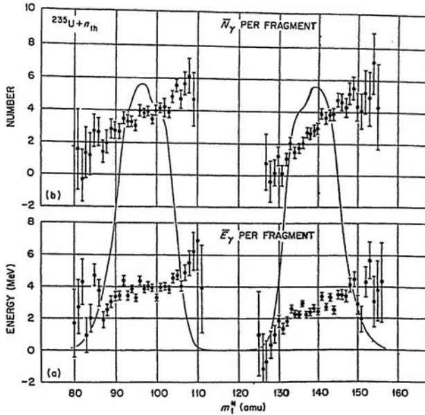
Fig. 1.13. Average number of gamma-rays emitted, N_\gamma and their total energy observed, \bar{E}_\gamma is plotted as a function of fragment atomic mass in the thermal neutron induced fission of ^{235}\text{U} [1.86]. The solid curve refers to observed mass spectrum
