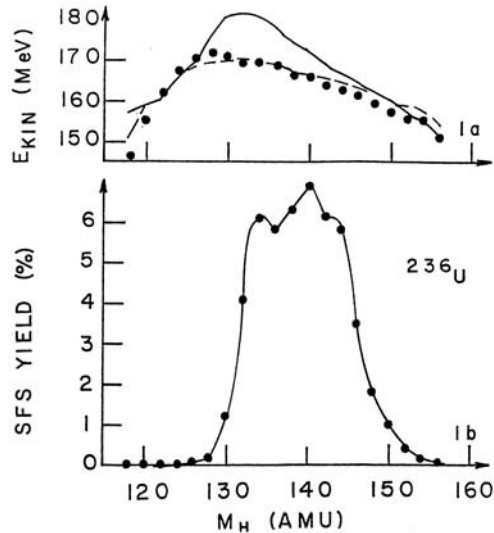
Fig. 5.4. The average kinetic energy, E_{\text{kin}} in MeV, and percentage mass yields spectra, SFS yield (%), associated with spontaneous fission of ^{236}\text{U} . The data taken from [5.34] are shown as solid lines. The broken line in the upper insert is the average kinetic energy used in calculating percentage mass yields shown as solid dots in the lower insert
