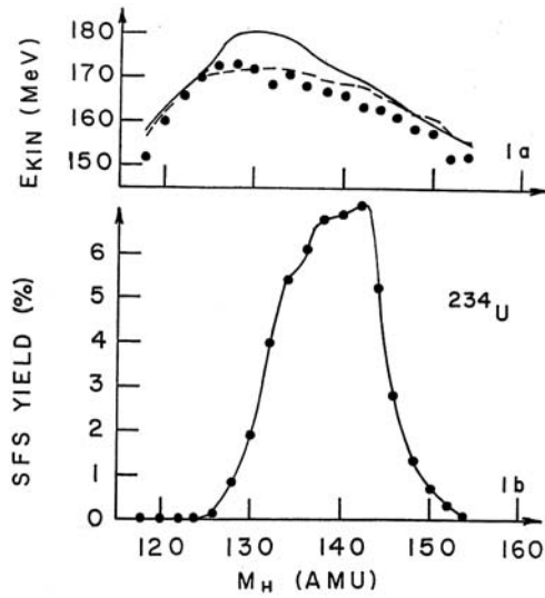
Fig. 5.3. The average kinetic energy E_{\text{kin}} in MeV, and percentage mass yields spectra, SFS yield (%) associated with spontaneous fission of ^{234}\text{U} . The data taken from [5.34] are shown as solid lines. The broken line in the upper insert is the average kinetic energy used in calculating percentage mass yields shown as solid dots in the lower insert
