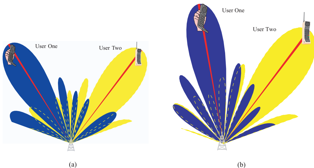
FIGURE 4.13: Fully adaptive spatial processing supporting two users on the same conventional channel simultaneously in the same cell [20].
