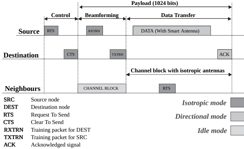
FIGURE 7.8: The proposed channel access protocol [24].
