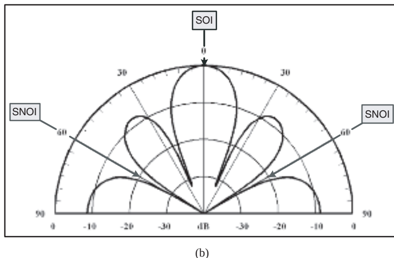
FIGURE 4.5: Adaptation procedure: (a) Calculation of the beamformer weights [20] and (b) Beam-formed antenna amplitude pattern to enhance SOI and suppress SNOIs.
