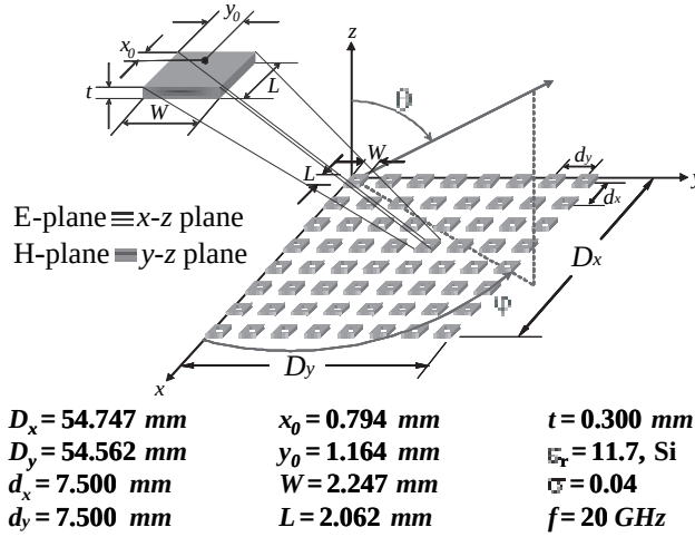
FIGURE 7.1: Planar-array configuration.
