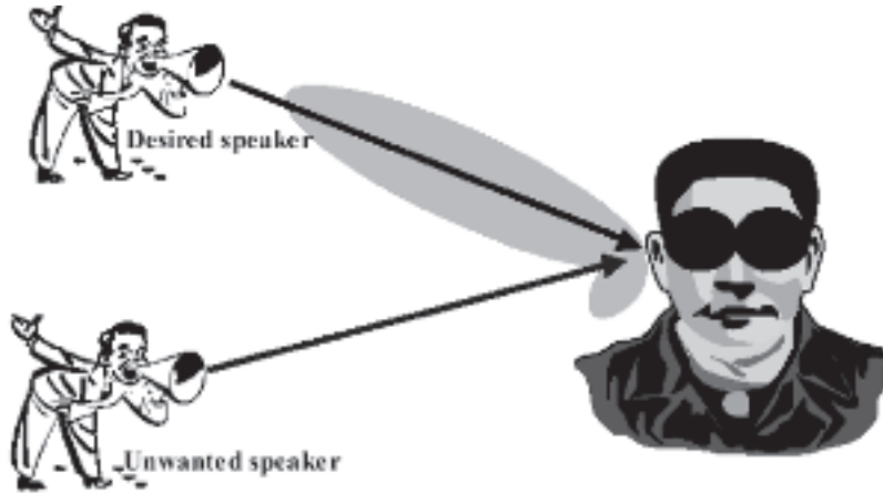
FIGURE 4.2: Human auditory function [17].
