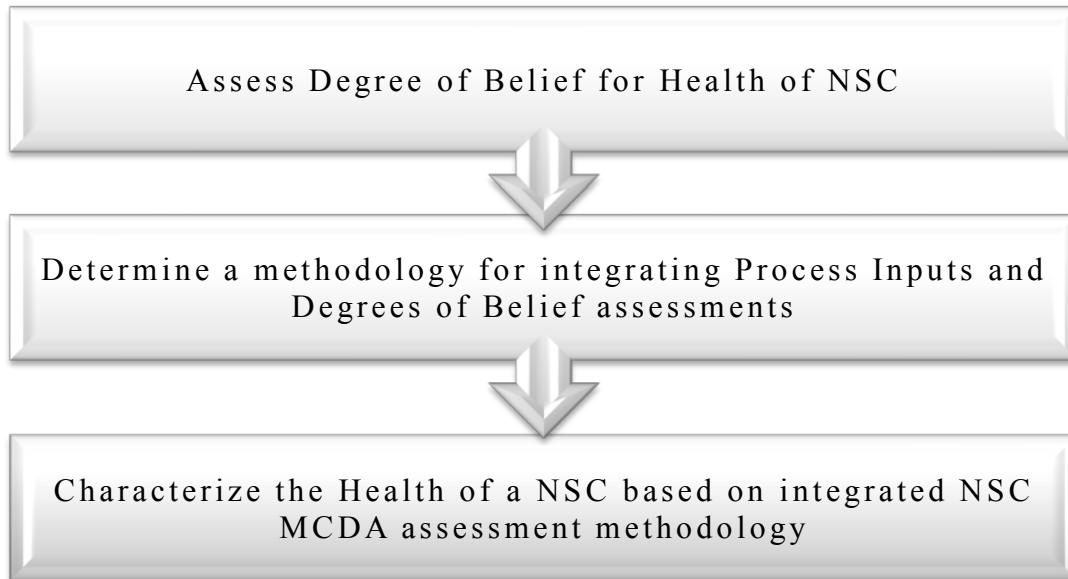
Figure 3. Research Purpose
