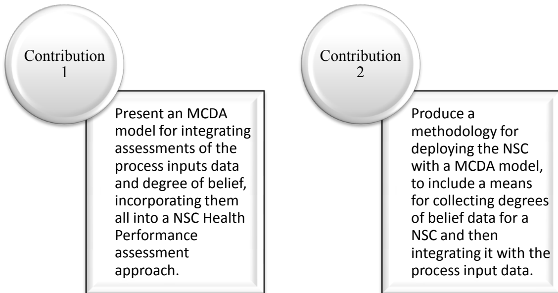
Figure 5. Research Contributions
