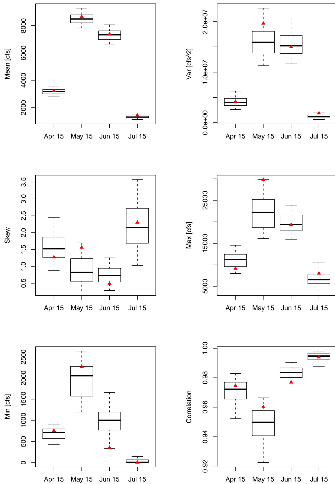
Figure 3.2: Daily statistics on the 15th of each month for 250 simulations of 88 years each of stream-flow. The boxes extend to the 25th and 75th percentiles while the whiskers represent the 5th and 95th percentiles. The historical value is shown as the red triangle.
