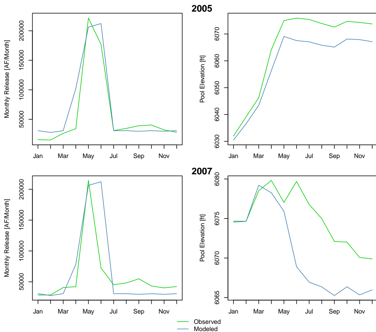
Figure 3.31: Comparison between modeled results and observed historical values for Navajo's release and end-of-month pool elevation. The top two figures are for 2005, while the bottom figures are for 2007.
