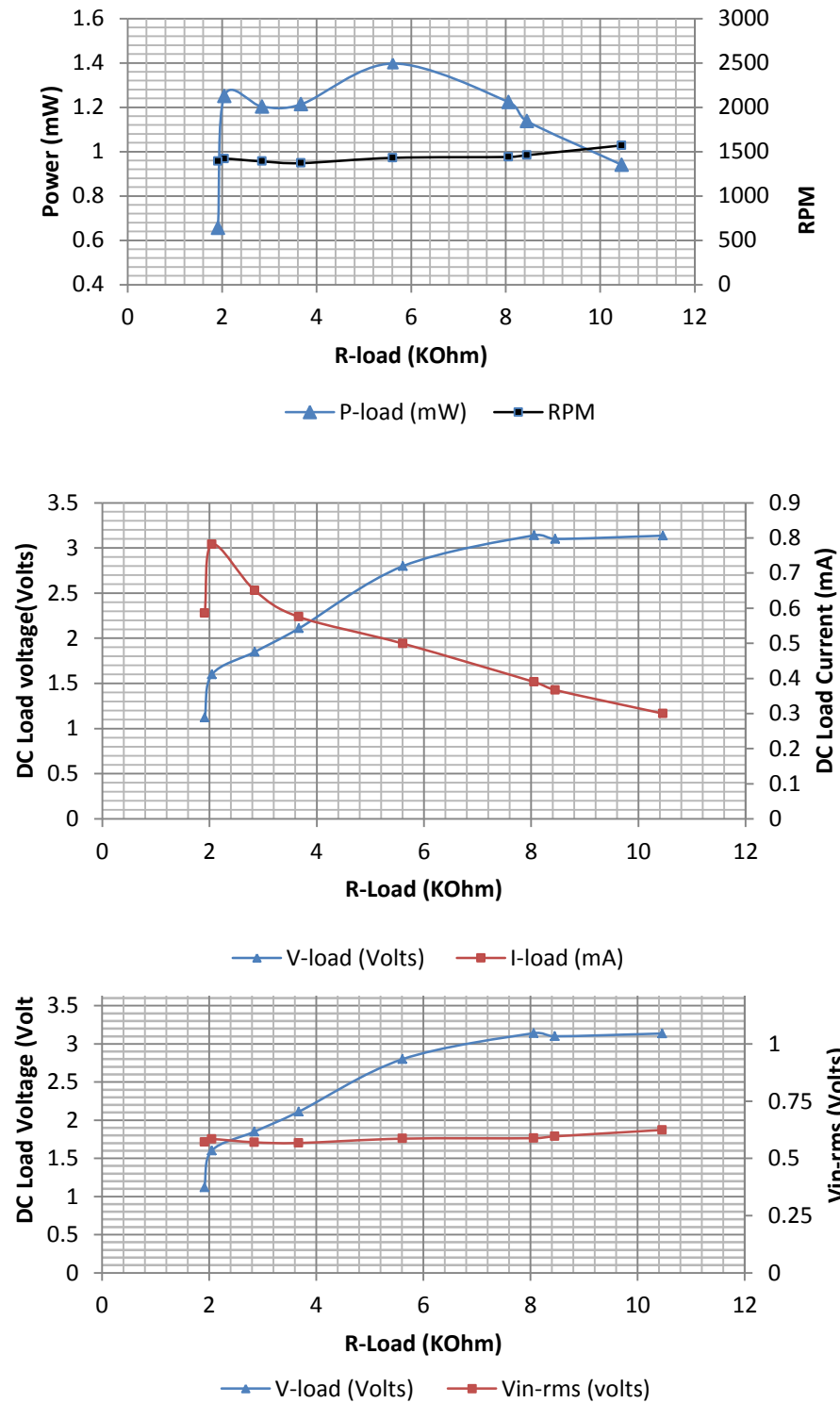
Figure 9.10 OTI-1 (N) DC power, DC load voltage/current, RPM and generator voltage against load resistance, using BQ25504 to boost the voltage sent to the load.
