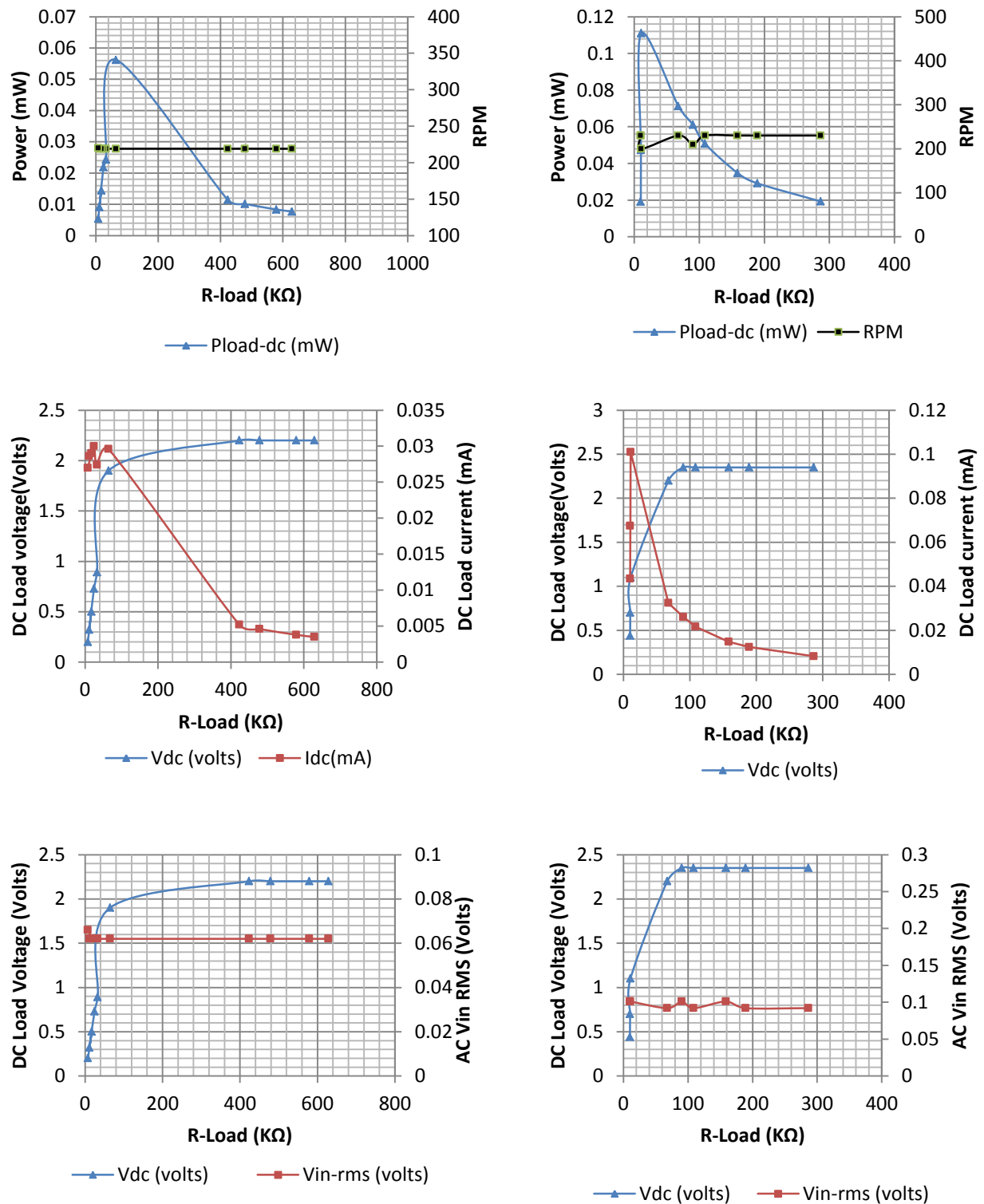
Figure 9.29 OTI-1 (SB) DC power, DC load voltage, DC load current, RPM and rms generator voltage against load resistance, using LTC 3108 Supercap (left) and LTC 3108 femto (right)
