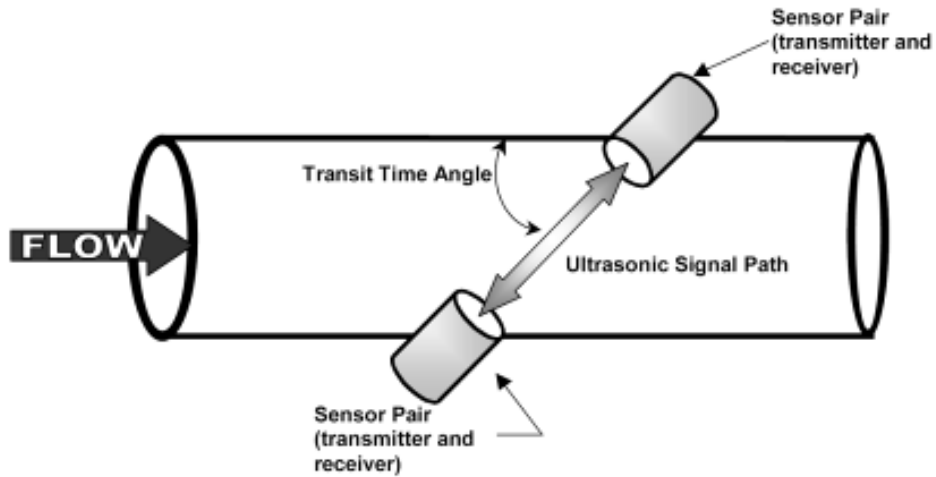
Figure 8.10 Principle of operation of ultrasonic flowmeter used in this work[89].
