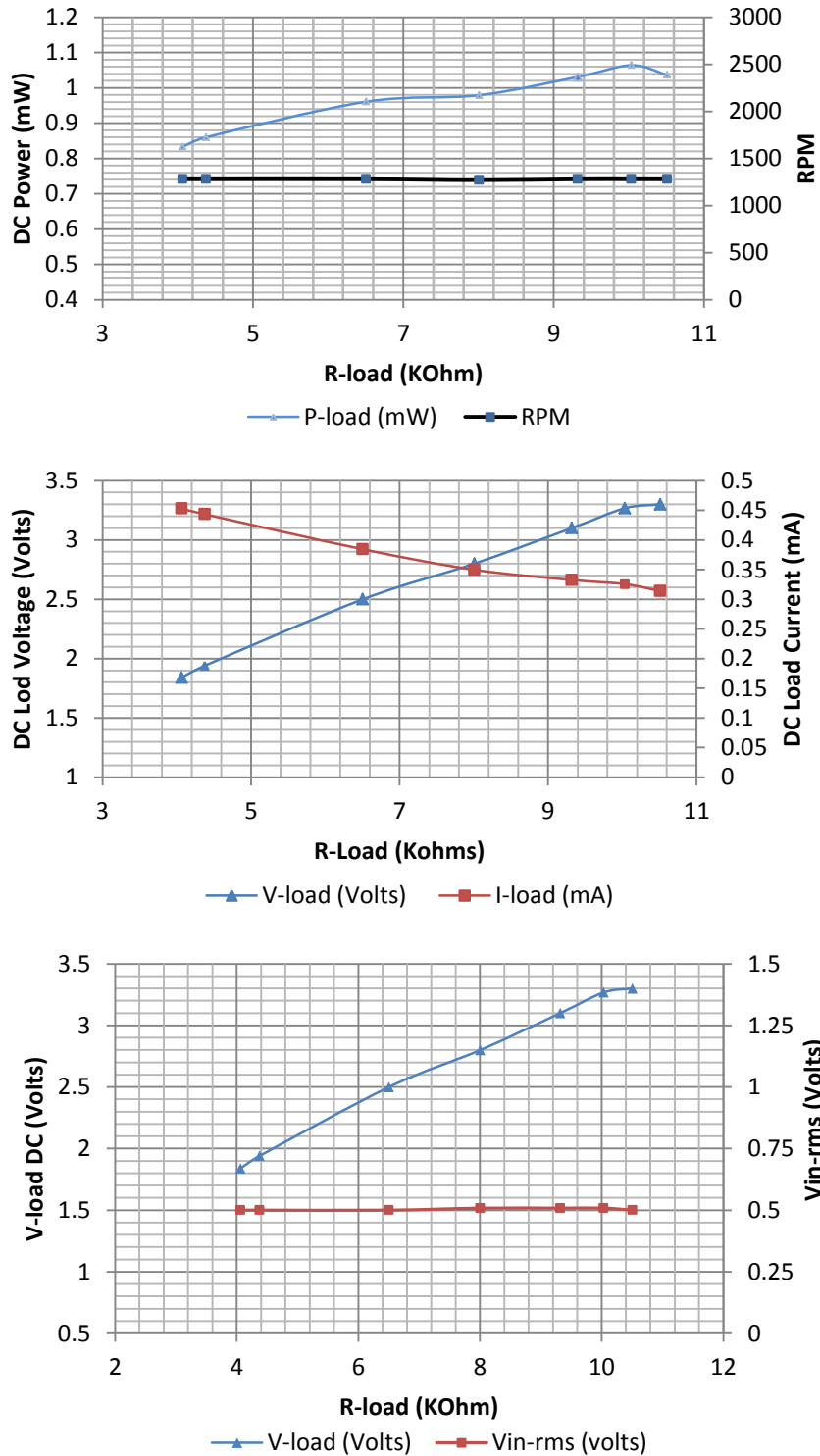
Figure 9.11 OTI-1 (N) DC power, DC load voltage/current, RPM and generator voltage against load resistance, using LTC 3105 to boost the voltage sent to the load.
