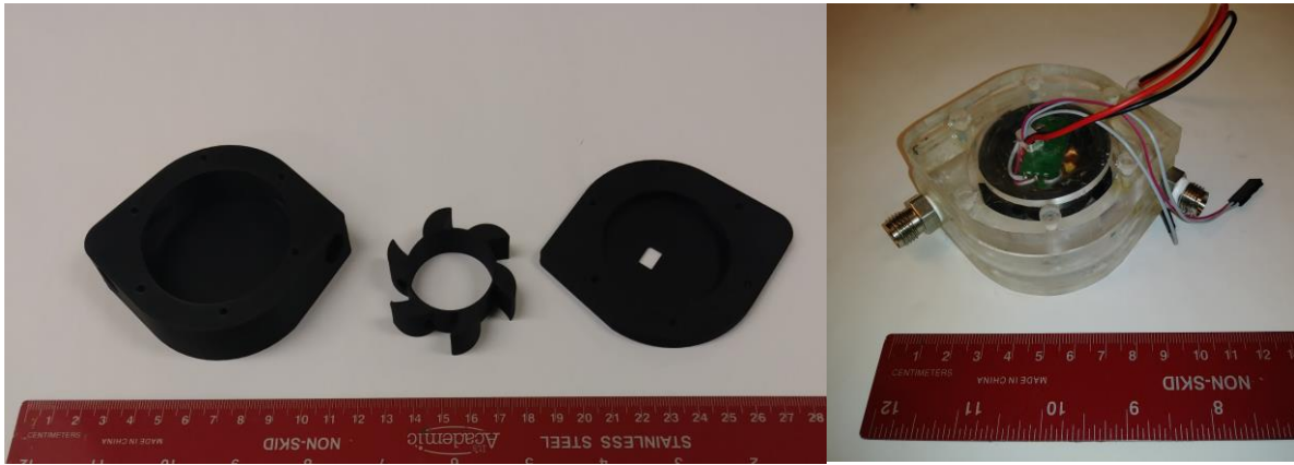
Figure 7.8 LST casing rotor and lid 3D printed in ABS on the left and CNC-machined LST assembled for testing on the right.
