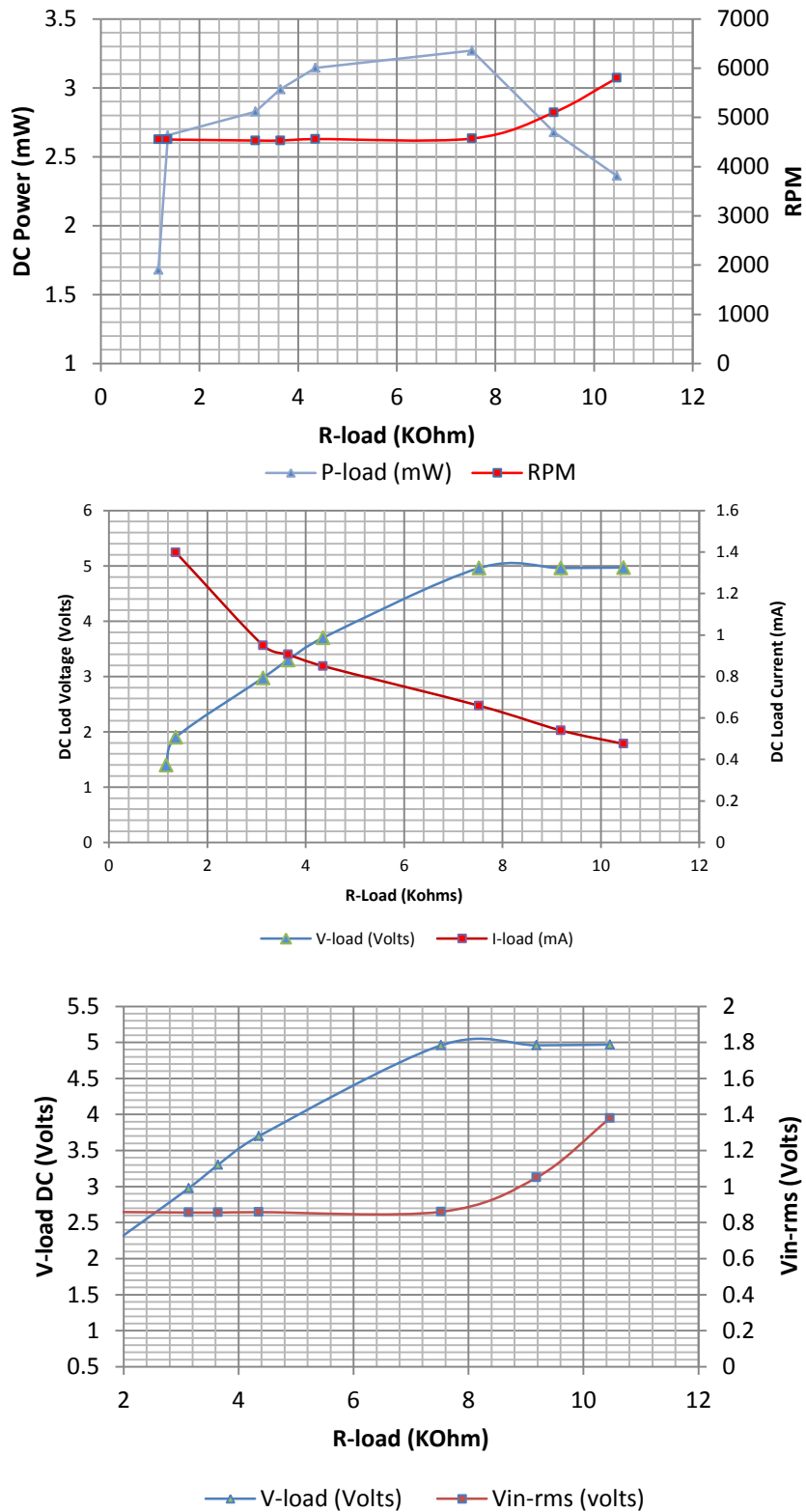
Figure 9.13 OTI-2 (N) DC power, DC load voltage/current, RPM and generator voltage against load resistance, using LTC3105 to boost the voltage sent to the load to 5 volts.
