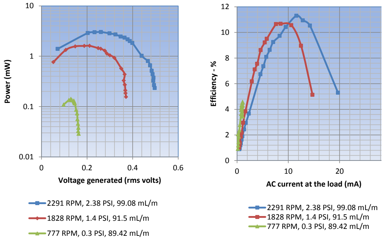
Figure 9.16 MST (W) AC power in mW vs generated rms voltage in volts for different RPM, pressure difference in PSI and flow Q in mL/m (left) and efficiency vs load current in mA (right)
