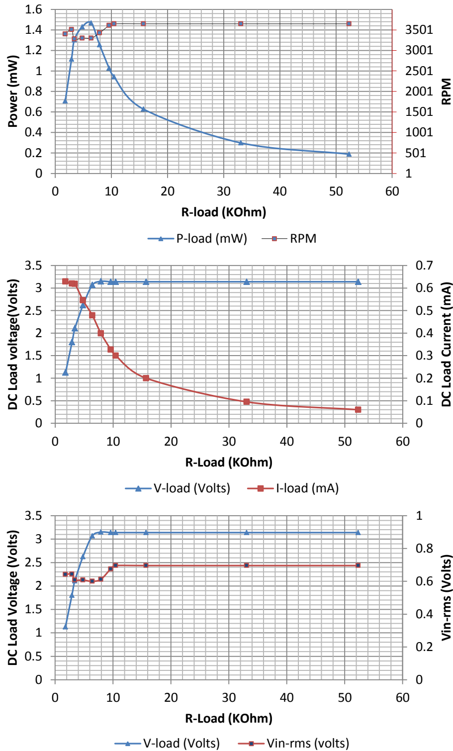
Figure 9.8 MST (N) DC power, DC load voltage/current, RPM and generator voltage against load resistance, using TI BQ 25504 to boost the voltage sent to the load.
