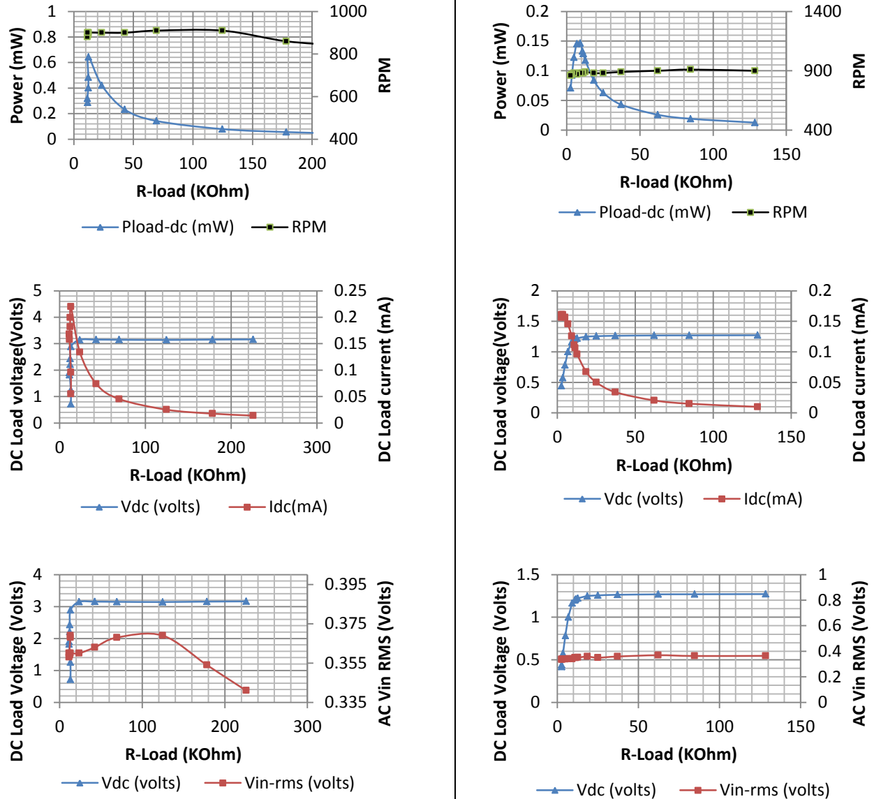
Figure 9.23 OTI-1 (W) DC power, DC load voltage, DC load current, RPM and RMS generator voltage against load resistance, using TI BQ 25504 (left) and LTC 3105 (right)
