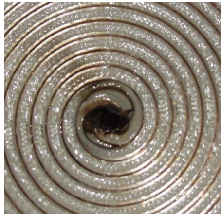
Figure 3.12. Damage incurred during thermal testing with 50 W incident power at 3 GHz.
