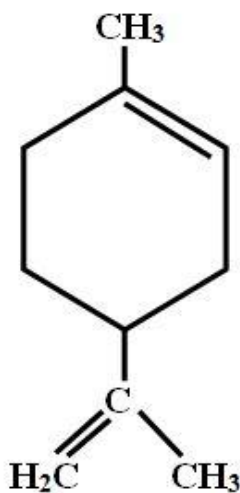
Figure 6: Structural representation of d-limonene
