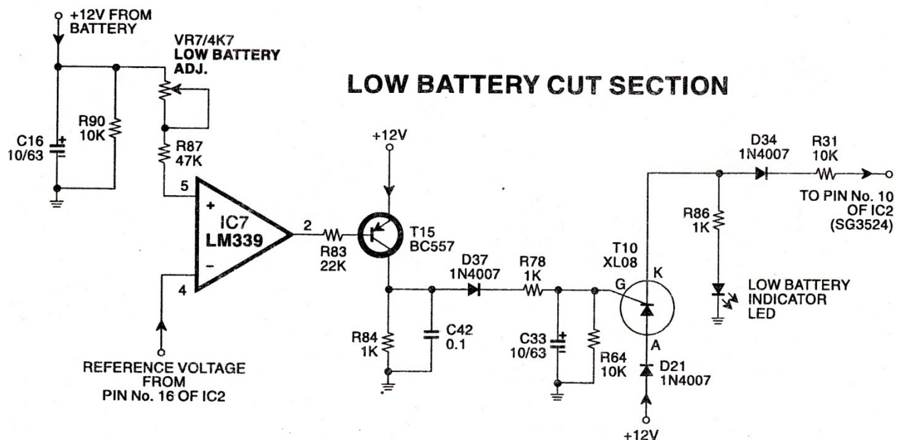
Fig: 2.5 low battery cut section
