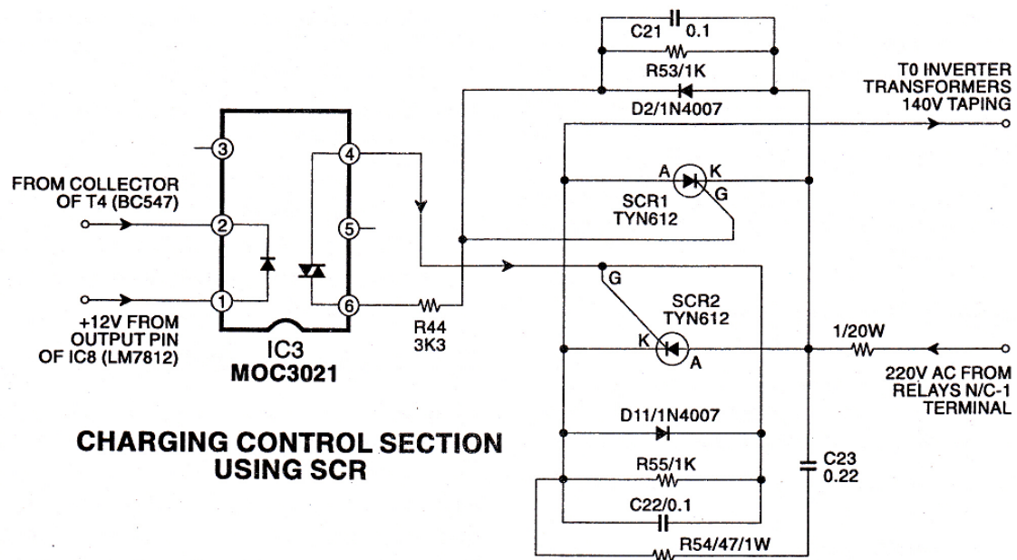
Fig: 2.9 Circuit diagram of charging control section using SCR
