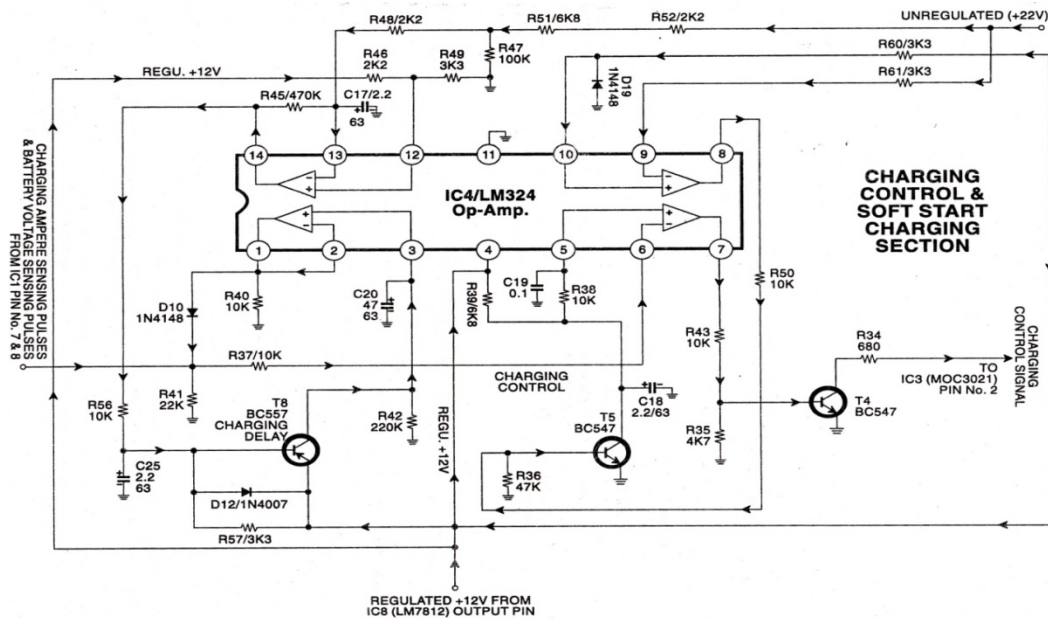
Fig: 2.7 charging control & soft start charging section
