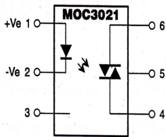
Fig 1.3.5 diagram of MOC3021
