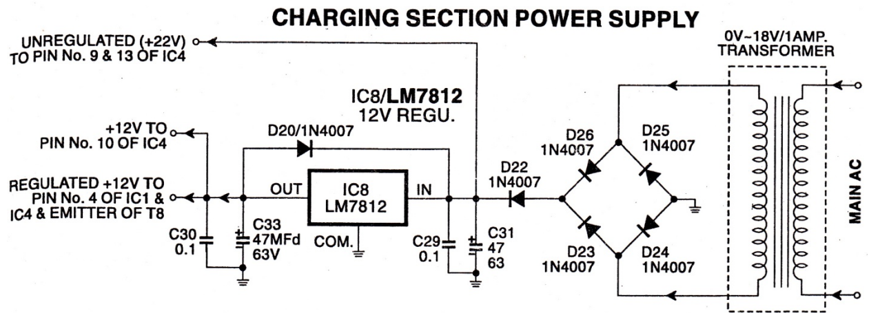
Fig: 2.6 charging section power supply
