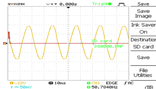
Fig: 4.7 Output of the sine wave inverter manufactured by SINGER
