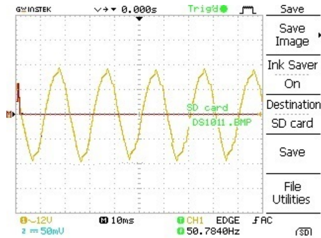
Fig: 5.8 Rahimafrooz manufactured inverter's output in Digital Oscilloscope after 30 days
