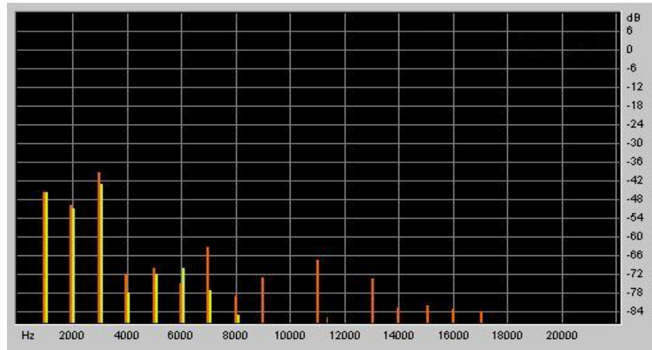
Fig: 4.4 THD in voltage for the output of Pure Sine Wave Inverter of BU project
