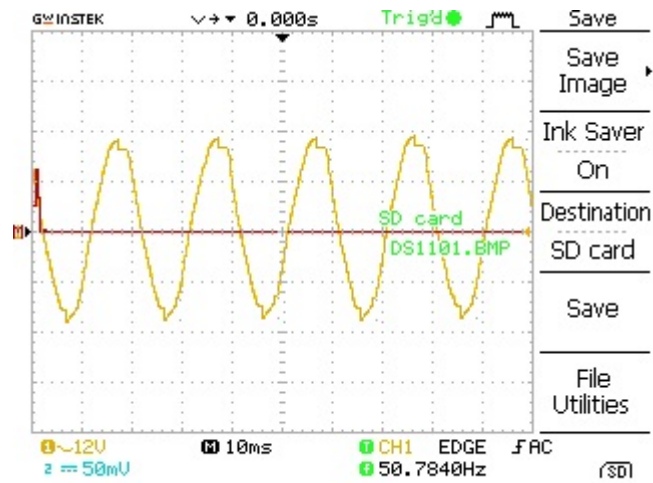
Fig: 5.5 BU project inverter's output in digital oscilloscope
