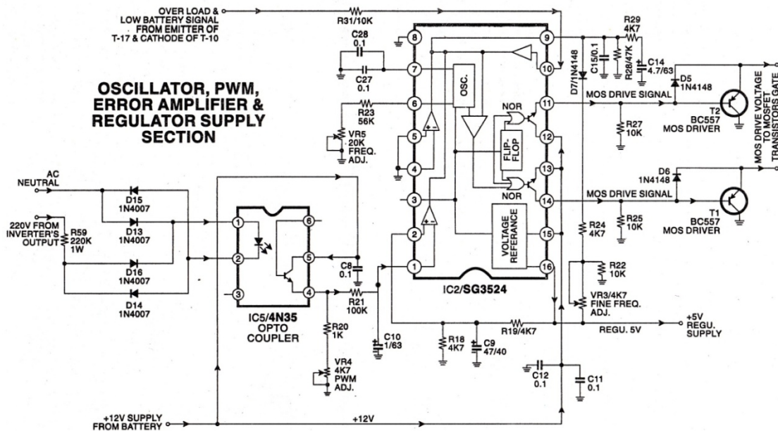
Fig: 2 Oscillator, PWM, error amplifier & regulator supply section
