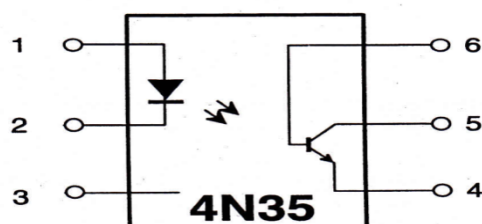
Fig: 1.3.4 Internal block diagram of IC 4N35
