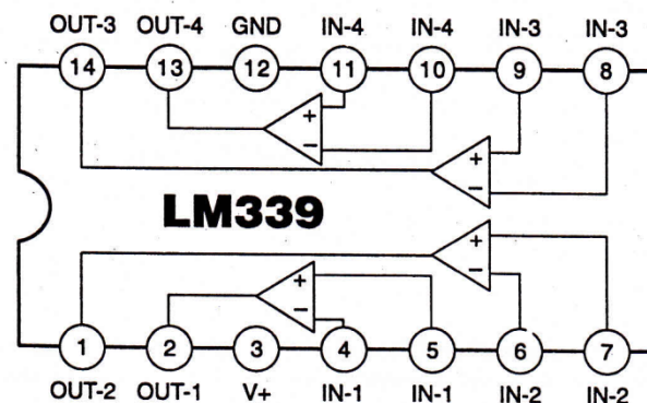
Fig: 1.3.1 Internal block diagram of ICLM339
