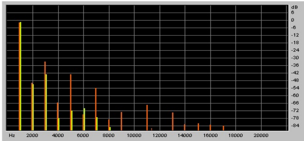
Fig: 4 THD in voltage for the output of Pure Sine Wave Inverter manufactured by Rahimafrooz
