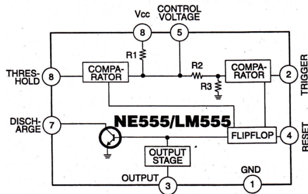
Fig: 1.3.3 Internal Block diagram of IC NE555-timer
