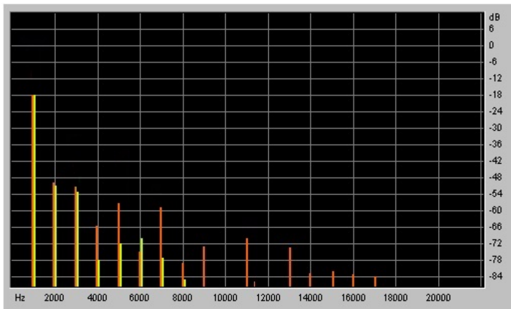
Fig: 4.1 THD in voltage for the output of Pure Sine Wave Inverter manufactured by SINGER
