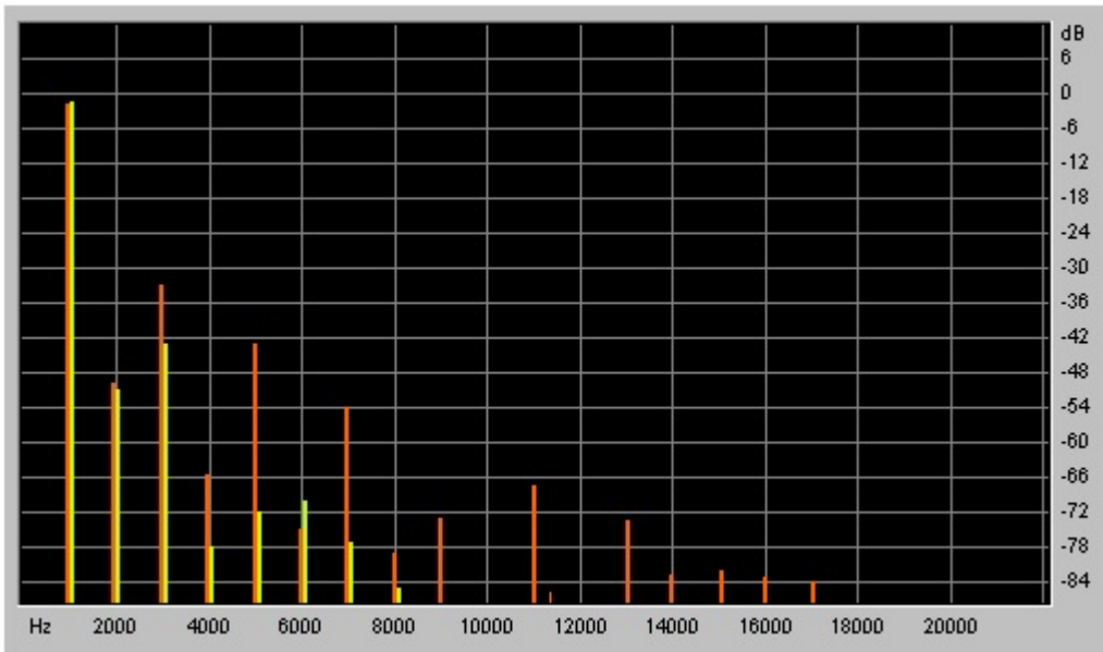
Fig: 5.3 Rahimafrooz manufactured inverter's THD of voltage in Spectrum Analyzer
