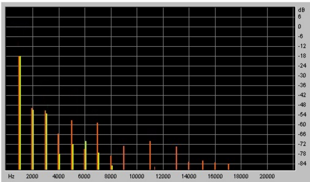
Fig: 5.4 Rahimafrooz inverter's THD of voltage in Spectrum Analyzer after 30 days
