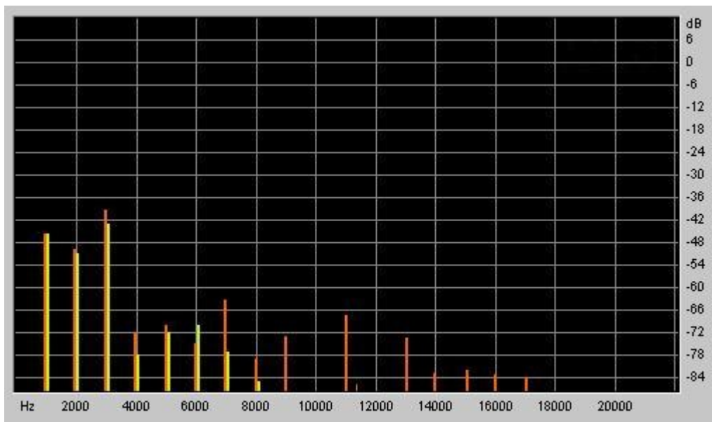
Fig: 5.2 BU project inverter's THD of voltage in Spectrum Analyzer after 30 days
