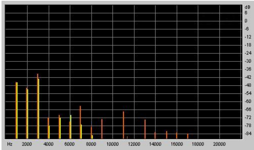
Fig: 5.1 BU Project inverter's THD of voltage in Spectrum Analyzer
