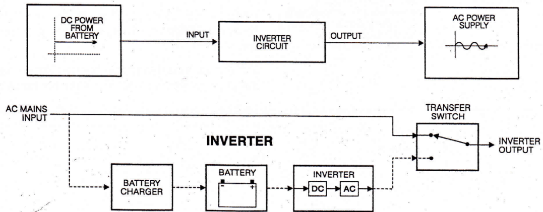
Fig: 1: block diagram of inverter
