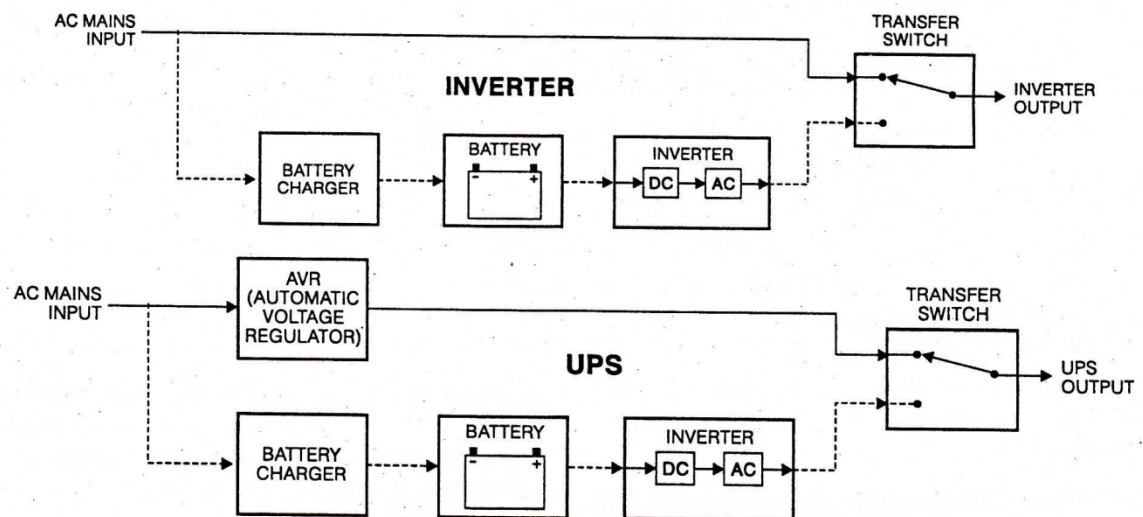
Fig: 1.1 block diagram of IPS and Inverter
