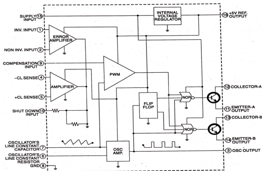
Fig: 1.3.2 internal block diagram of IC SG3524
