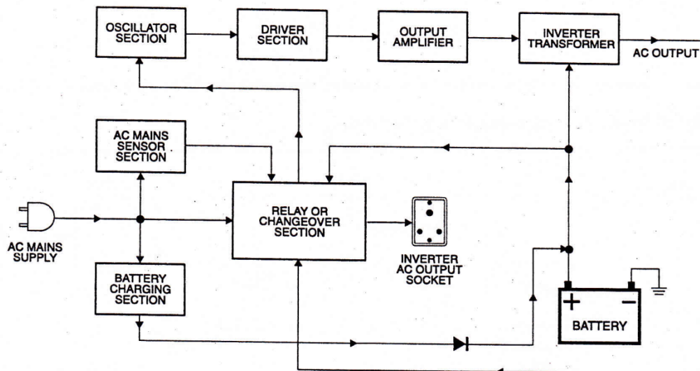
Fig: 1.2 Basic diagram of an inverter
