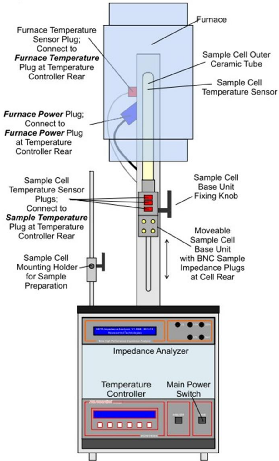
Figure 4.4. Novocontrol™ system.
