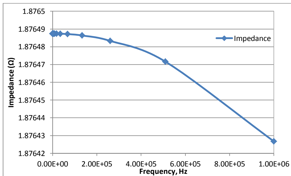
Figure 5.19. Impedance response of the 60%GDC-40%CF0 membrane generated using COMSOL™.
