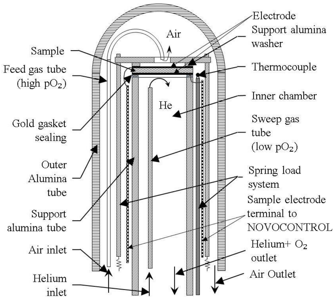
Figure 3.2. Probostat TM sample stage schematic.
