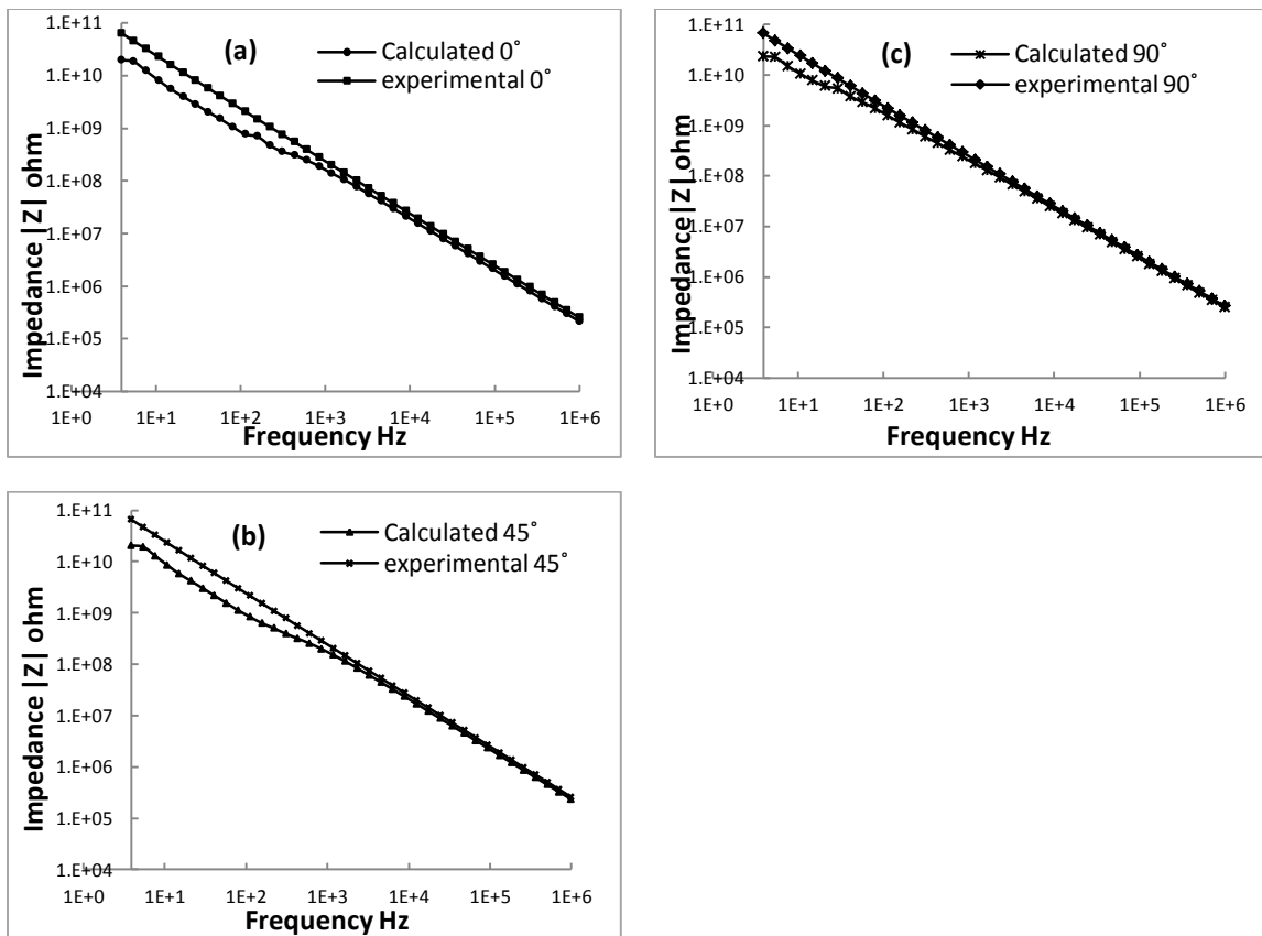
Figure 5.8. Measured impedance response vs computed impedance response of the epoxy-tin composite material (a) 0^\circ orientation of the lenticular tin inclusion with the applied field, (b) 45^\circ orientation of the lenticular tin inclusion with the applied field and (c) 90^\circ orientation of the lenticular tin inclusion with the applied field.
