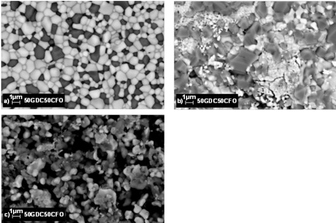
Figure 3.11. Scanning electron micrographs showing microstructure of the 50%GDC-50% CFO perovskite membrane: a) Fresh polished membrane surface as fabricated, b) Air Side surface and c) permeate side surface.
