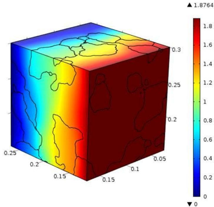
Figure 5.18. Voltage distribution in the 60%GDC-40%CF0 membrane generated using COMSOL™.
