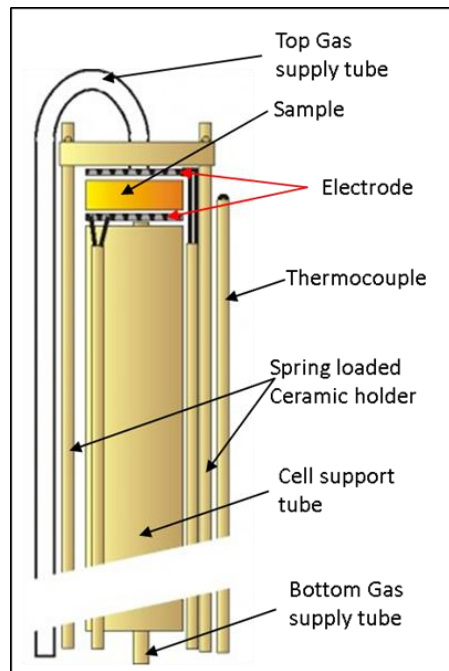
Figure 4.8. Spring loads and regular 2-electrode 4-wire setup with dual gas supplies and thermocouple in a Probostat™.
