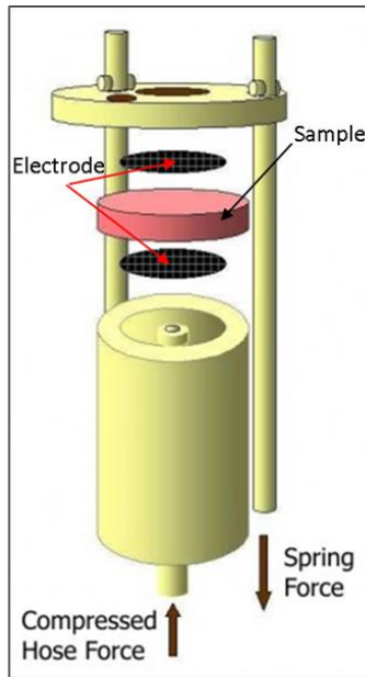
Figure 4.7. Sample inside the Probostat™ connected with two platinum wire mesh electrodes.
