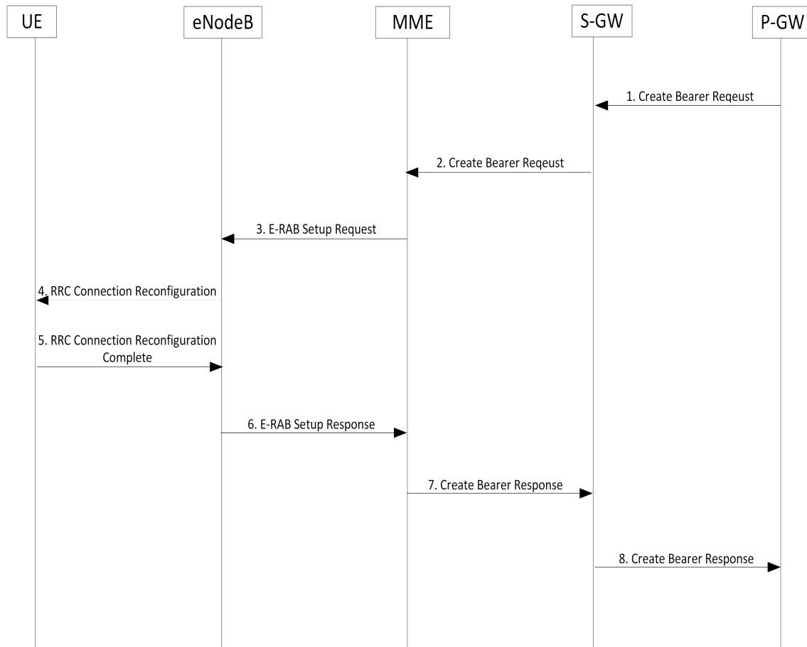
Figure 5.4 EPS bearer establishment procedures
