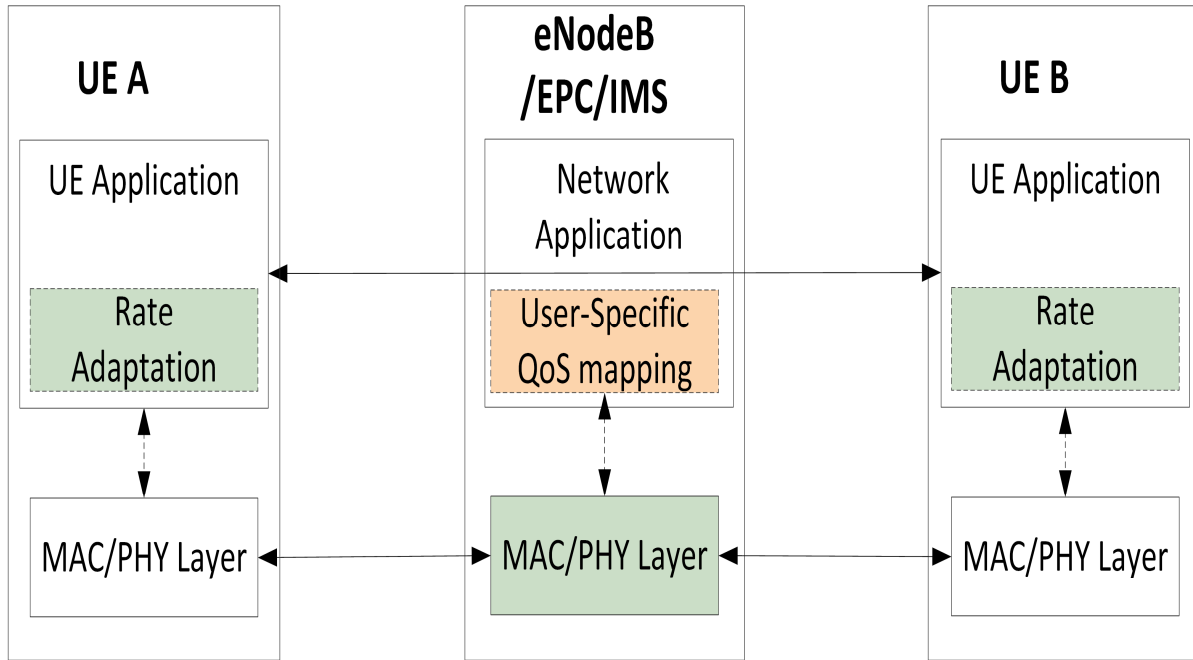
Figure 5.5 System architecture
