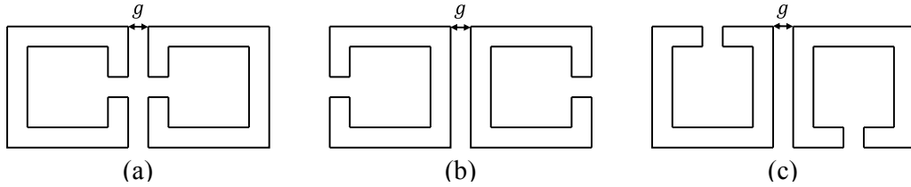
Figure 3.5 Electric coupling (a), magnetic coupling (b), and mixed coupling (c) modes for square open loop resonators.
