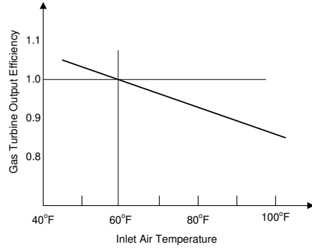
Figure 1: Cooler Inlet Air Yields Higher Turbine Output ([76])
