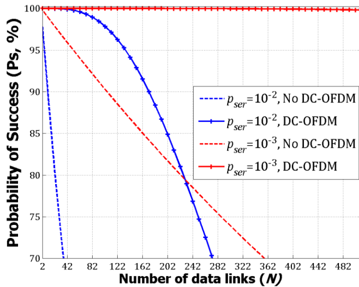
Figure 8.5 Performance of 3 – for – N DC – OFDM system for an OFDM-QPSK
