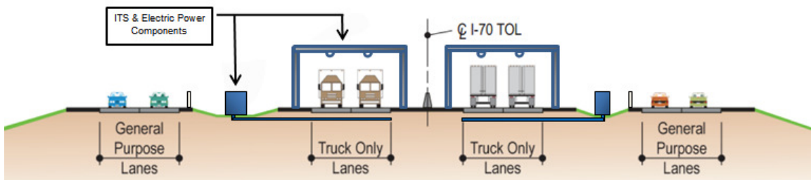
Figure 3-3 Proposed Cross-Section for AEHS. Adapted from MODOT, 2009
