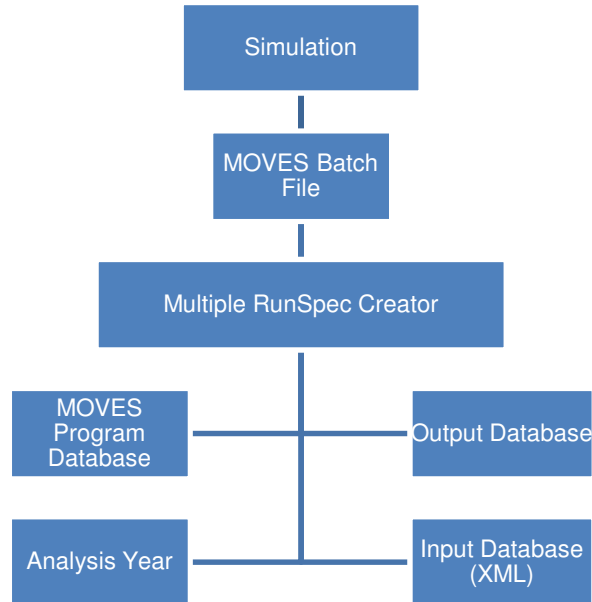
Figure 4-3 MOVES Multiple RunSpec Simulation Hierarchy
