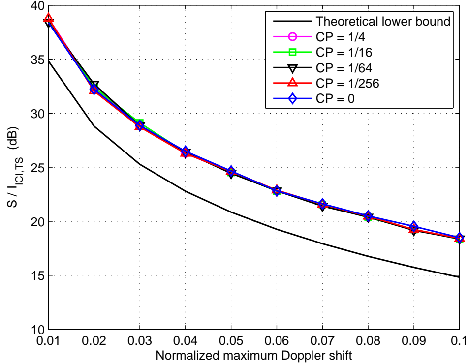
Figure 3.9 Estimated and theoretical S/I_{CI,TS} with both multipath channel with different Doppler spreads.
