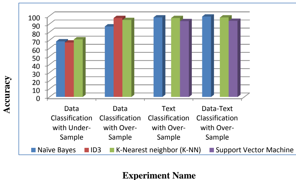
Figure 5.2: Accuracy for All our Experiments.
