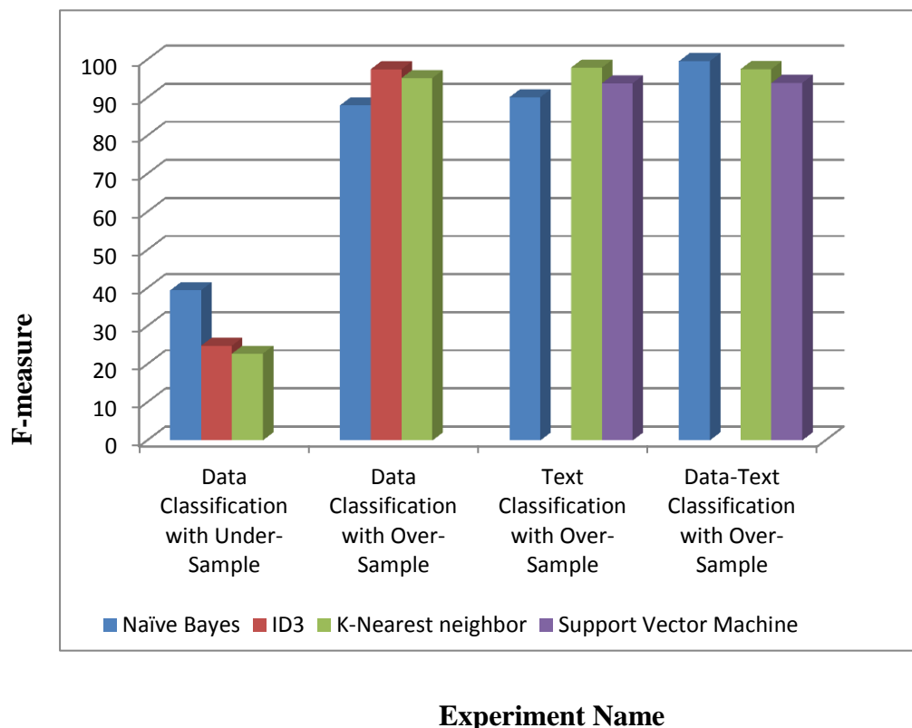
Figure 5.3: F-measure for All our Experiments.
