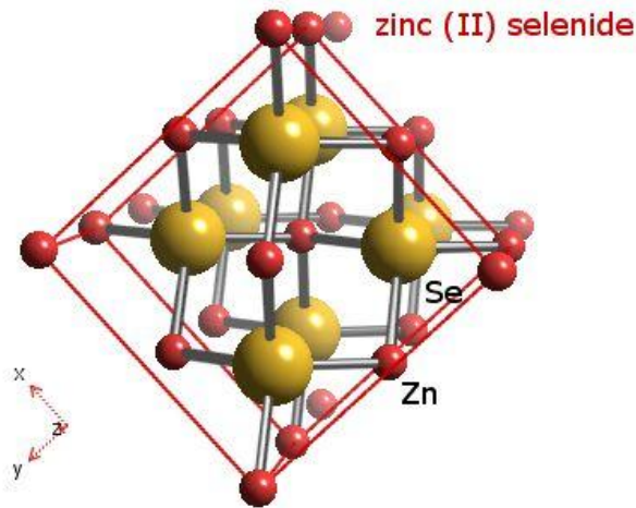
Fig. 2.16. ZnSe structure. [22]
