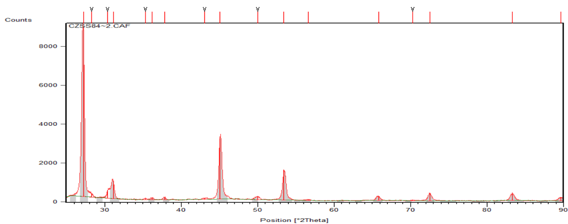
Fig. 4.7. XRD plot for CZSS 84 done at 350°C.
