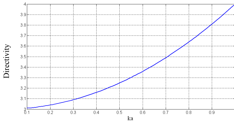
Figure 2.4: The Maximum Antenna Directivity
