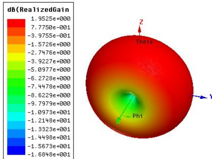
Figure 4.19: The Simulated 3D Pattern for the Meandered Dipole Antenna Design
