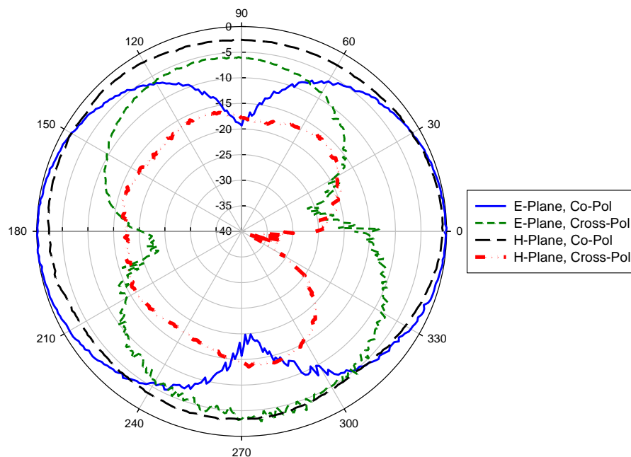
Figure 4.25: The Measured Radiation Patterns for the 3D Dipole Antenna Design
