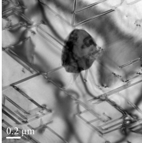
Figure 2.7 Micro-twinned crystal defect observed with plan-view TEM (PV-TEM). Data courtesy of C. Buongiorno, IMM-CNR, Catania, IT.
