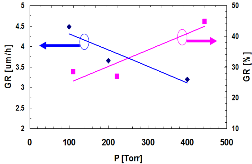
Figure 2.16 The impact of reactor pressure on the growth rate (GR [ \mu\text{m}/\text{h} ]) and (111)3C-SiC film thickness gradient (GR[%]). 50mm (111)Si wafer substrate. Reduced pressure improves thickness uniformity and increases deposition rate as expected (See Section 2.1). The trend lines are to aid the eye only and do not infer linear relationships.
