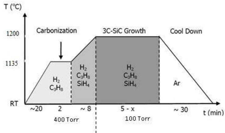
Figure 3.4 Initial baseline low temperature CVD growth process schedule.
