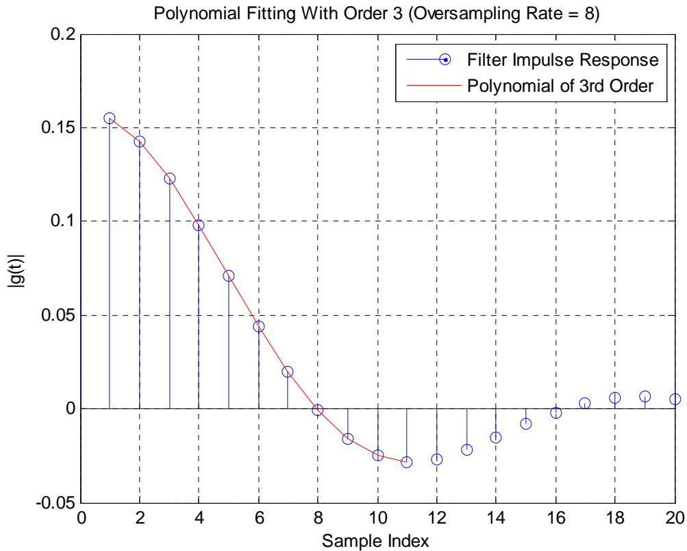
Figure 7: Representation of Polynomial Fitting
