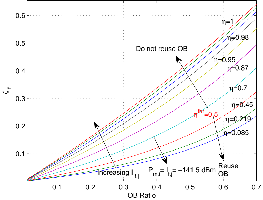
Figure 3.7 Femtocell capacity loss ratio ( \zeta_f ) vs. overlapped band (OB) ratio ( P_{m,i} = -141.5 dBm and I_{f,j} = \{-111.5, -116.5, \dots, -156.5\} dBm).
