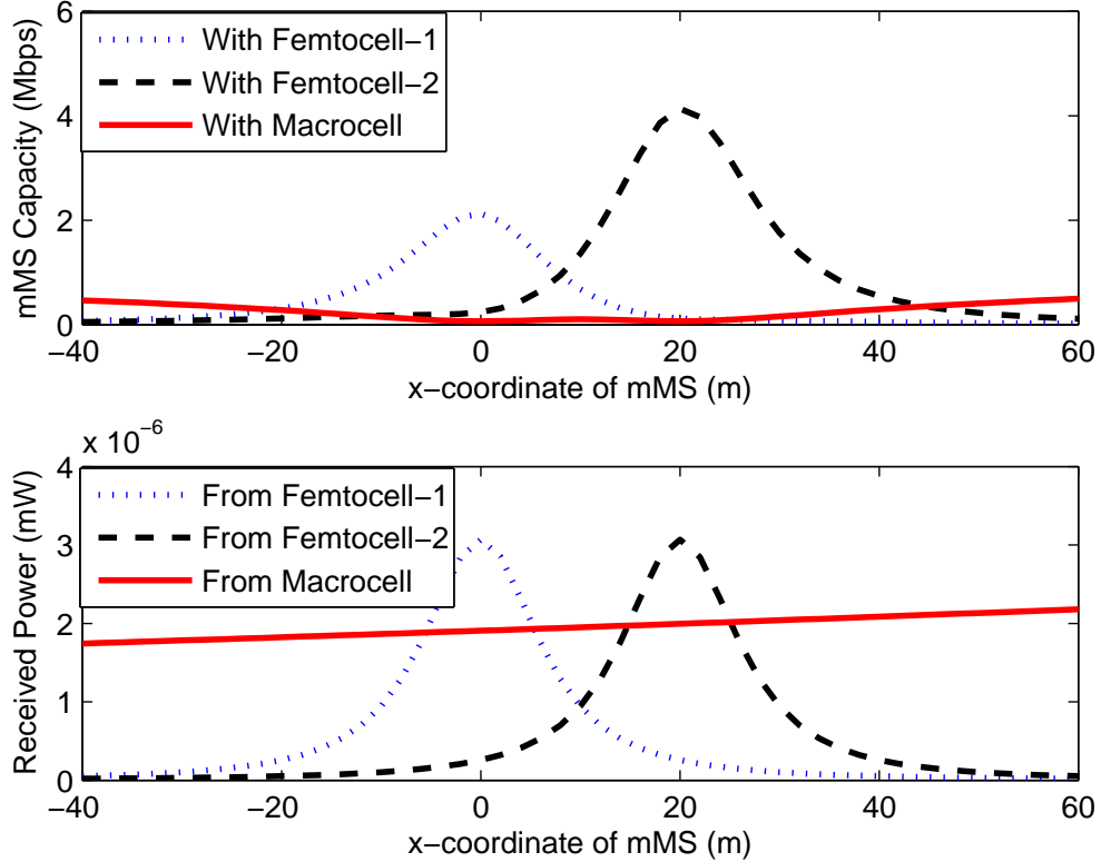
Figure 4.6 Capacity and RSS of mMS for associations with different cells ( d_{\text{mBS}} = 800 m).
