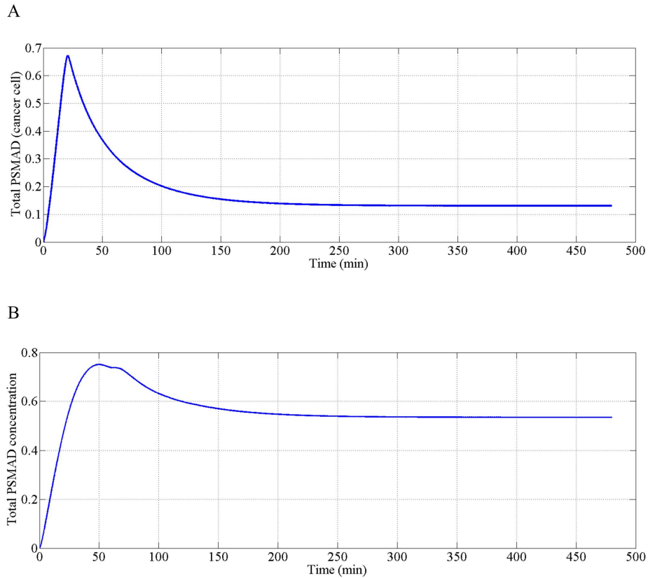
Figure 4.7: Total PSMAD time course for a certain TGF- \beta concentration. A) simulation results for low membrane receptor concentration condition (or so called early-stage tumors) B) simulation results for high membrane receptor concentration condition (or so called late-stage tumors). These conditions were simulated via altering the receptor production rate on the membrane.
