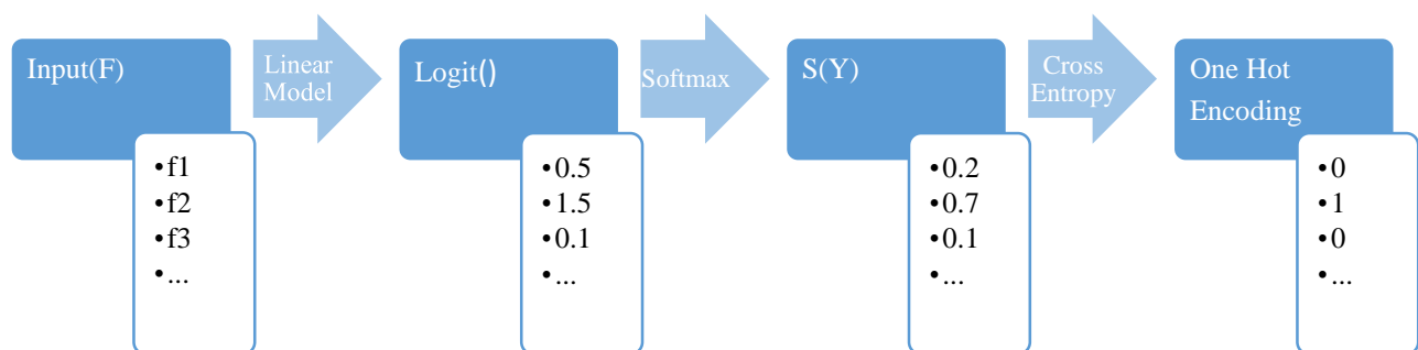
Figure (2.2): Multinomial LR Steps (Polamuri, 2017)
