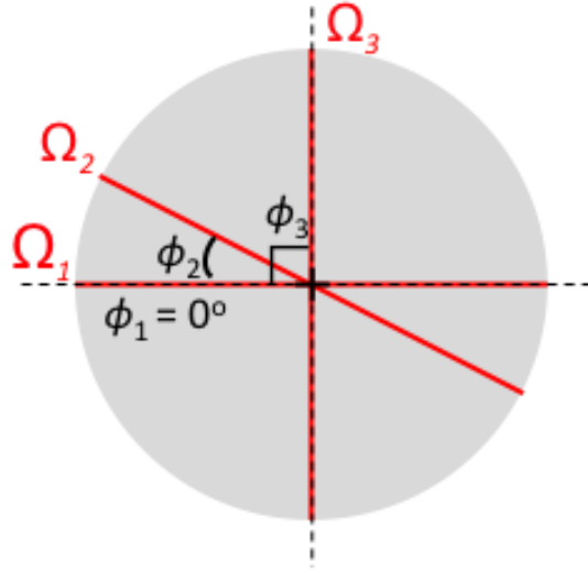
Figure 2.12: Spatial frequency representation with circles (repeated from Chp. 2).
