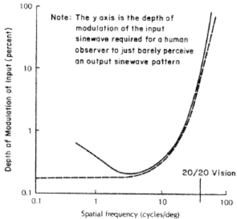
Figure 1.14: Modulation Transfer Function (MTF) of human visual system. Image from Ref. [23].
