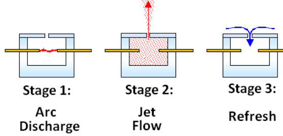
Figure 2.1: Basic schematic of the three stages of SparkJet operation.
