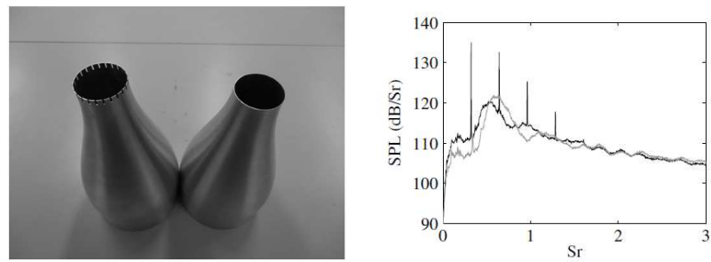
(a) Clean vs. Notched Nozzle Exit. (b) Sound pressure levels associated with a clean nozzle and a notched nozzle.
