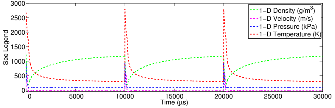
Figure 3.14: Simulation of the time dependent variation in cavity pressure, temperature, and density and the velocity through the orifice for three SparkJet cycles at 100 Hz.
