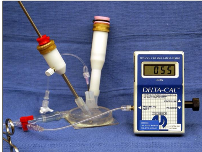
Figure 32 – Benchtop leak test setup
