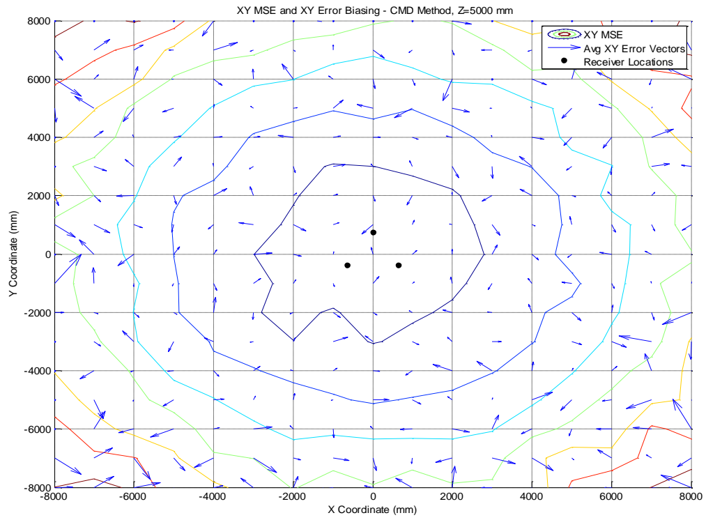
Figure 2.23: XY Error, Z = 5000mm
