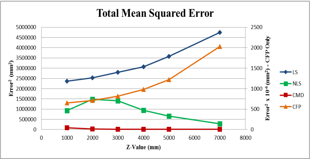
Figure 2.27: Total mean squared error
