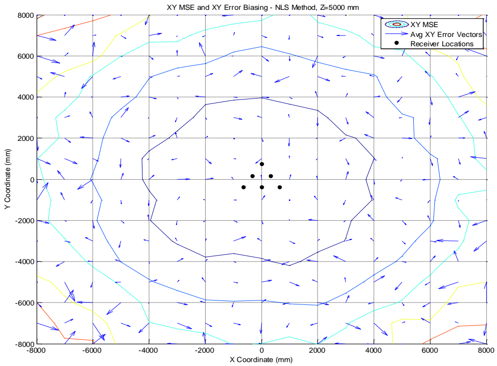
Figure 2.22: XY Error, Z = 5000mm
