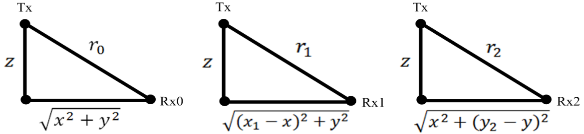
Figure 2.3: Geometric representation for each range measurement, r_i
