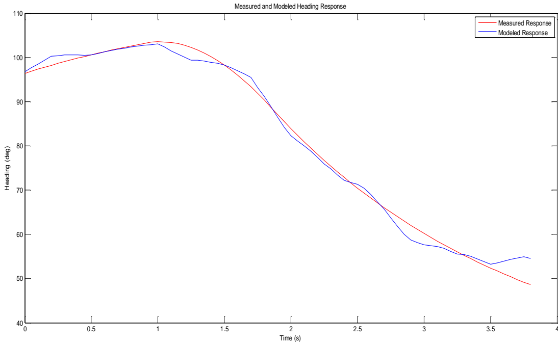
Figure 3.20: Measured and modeled heading response
