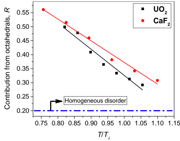
Figure 3.11 Temperature dependence of the role of octahedra in accommodating disorder, as seen from simulations. The lower values at temperatures close to T_\lambda indicate the dynamical nature of disorder in superionics.
