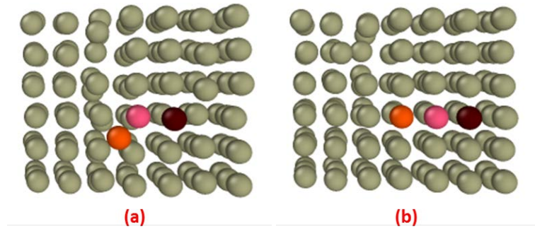
Figure 7.8 An example of cooperative motion among oxygen ions during cascade simulations of UO 2 – (a) and (b) represent snapshots of the system at two successive time intervals. Both the octahedral interstitial and the vacancy, which are three steps apart, get annihilated by means of string-like correlated jumps. The configurations are shown using OVITO [134].
