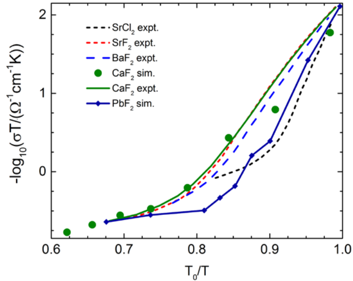
Figure 1.3 Variation of ionic resistivity, or inverse of ionic conductivity ( \sigma ), with temperature. T_0 has been chosen as the temperature at which the ionic conductivity has a value of 10^{-2.2} \Omega^{-1} \cdot \text{cm}^{-1} . The behavior of the plot changes little when T_\lambda is chosen for T_0 . The plot is digitized from [11].
