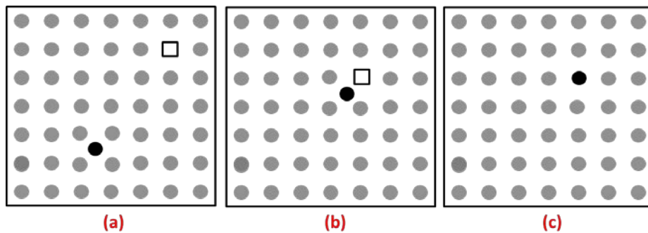
Figure 7.7 A vacancy-interstitial recombination. (a) A well-separated vacancy and an interstitial. (b) Vacancy and interstitial moving closer to each other. (c) Vacancy-interstitial annihilation.
