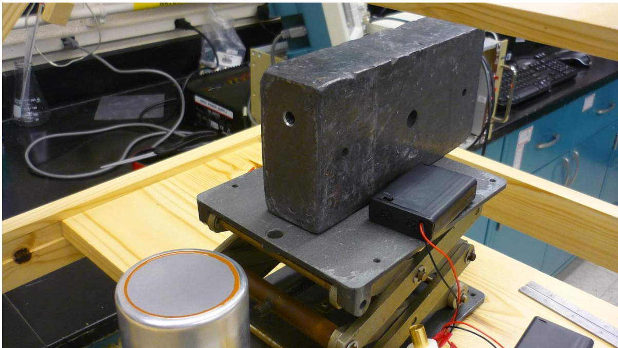
Figure 11 – Perspective view of lead collimator
