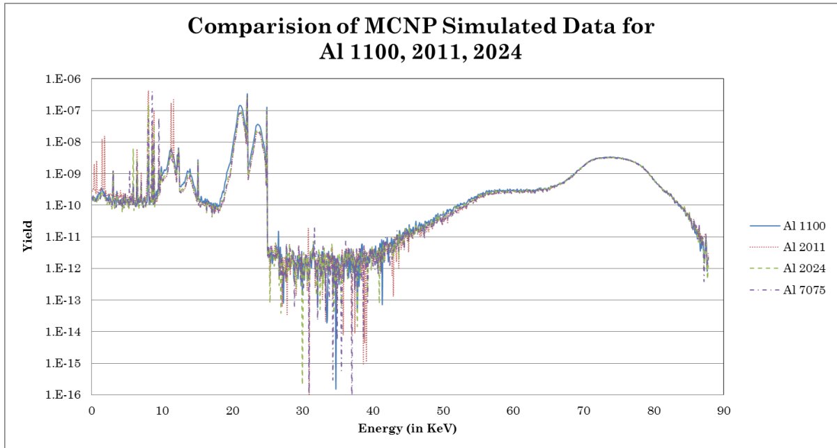
Figure 20 – MCNP Data for Al-1100, Al-2011, Al-2024, and Al-7075
