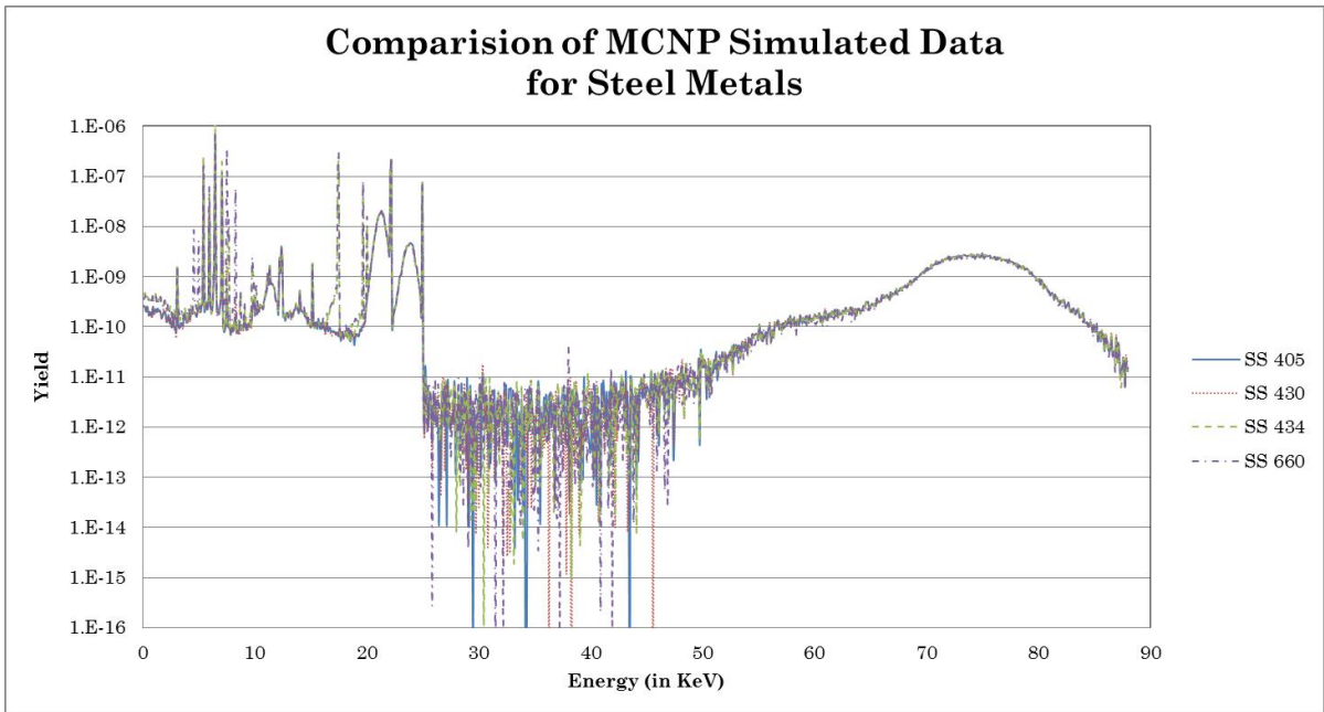
Figure 29 – MCNP Data for Stainless Steel 405, 430, 434, and 660
