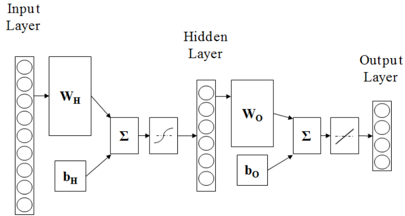
Figure 3 – Structure of Neural Net used in this study and its transformation functions.
