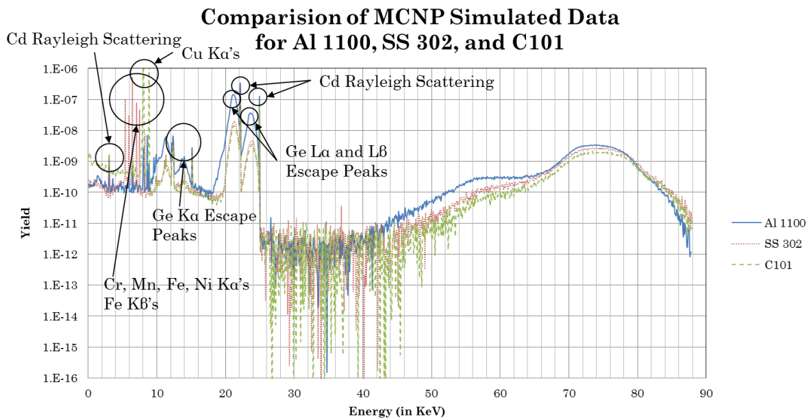
Figure 16 – MCNP Simulated Data
