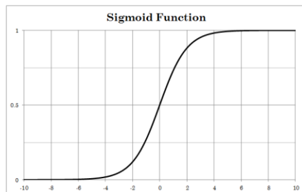
Figure 5 – Sigmoid function
