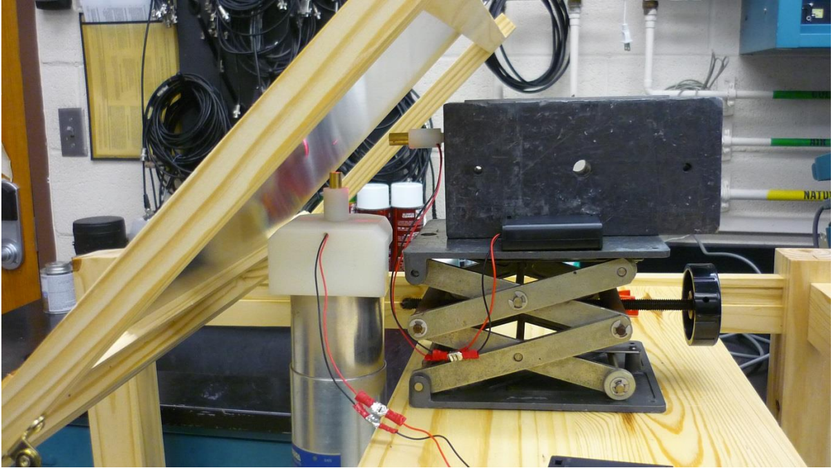
Figure 13 – View of Experimental setup with lasers mounted
