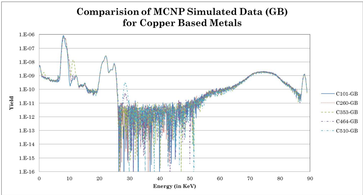
Figure 27 – Gaussian broadened MCNP Data for C101, C260, C260, C353, C464, and C510
