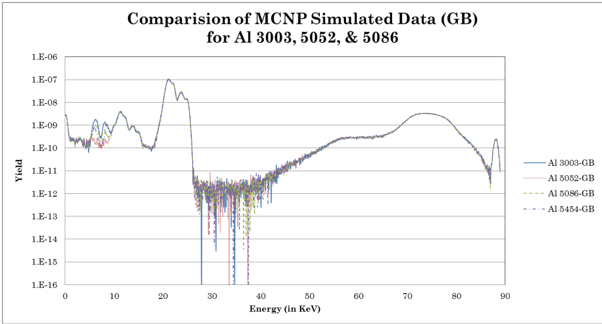
Figure 24 – Gaussian Broadened MCNP Data for Al-3003, Al-5052, Al-5086, and Al-5454
