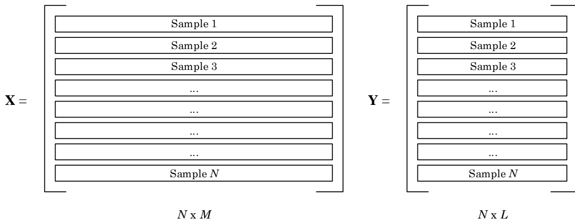
Figure 4 – X and Y data block structure
