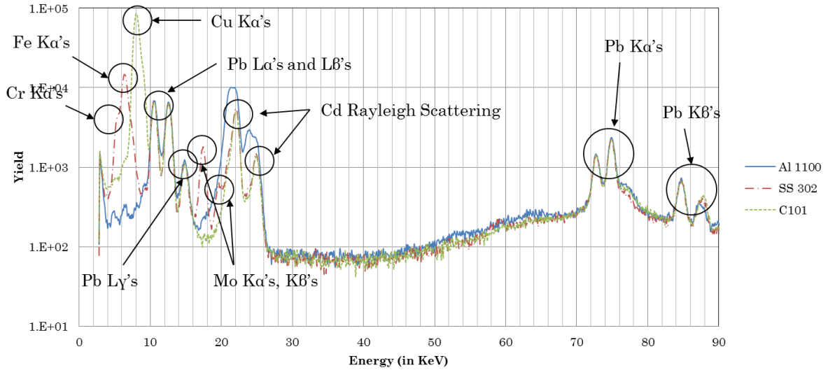
Figure 18 – Experimental Data with relevant peaks identified
