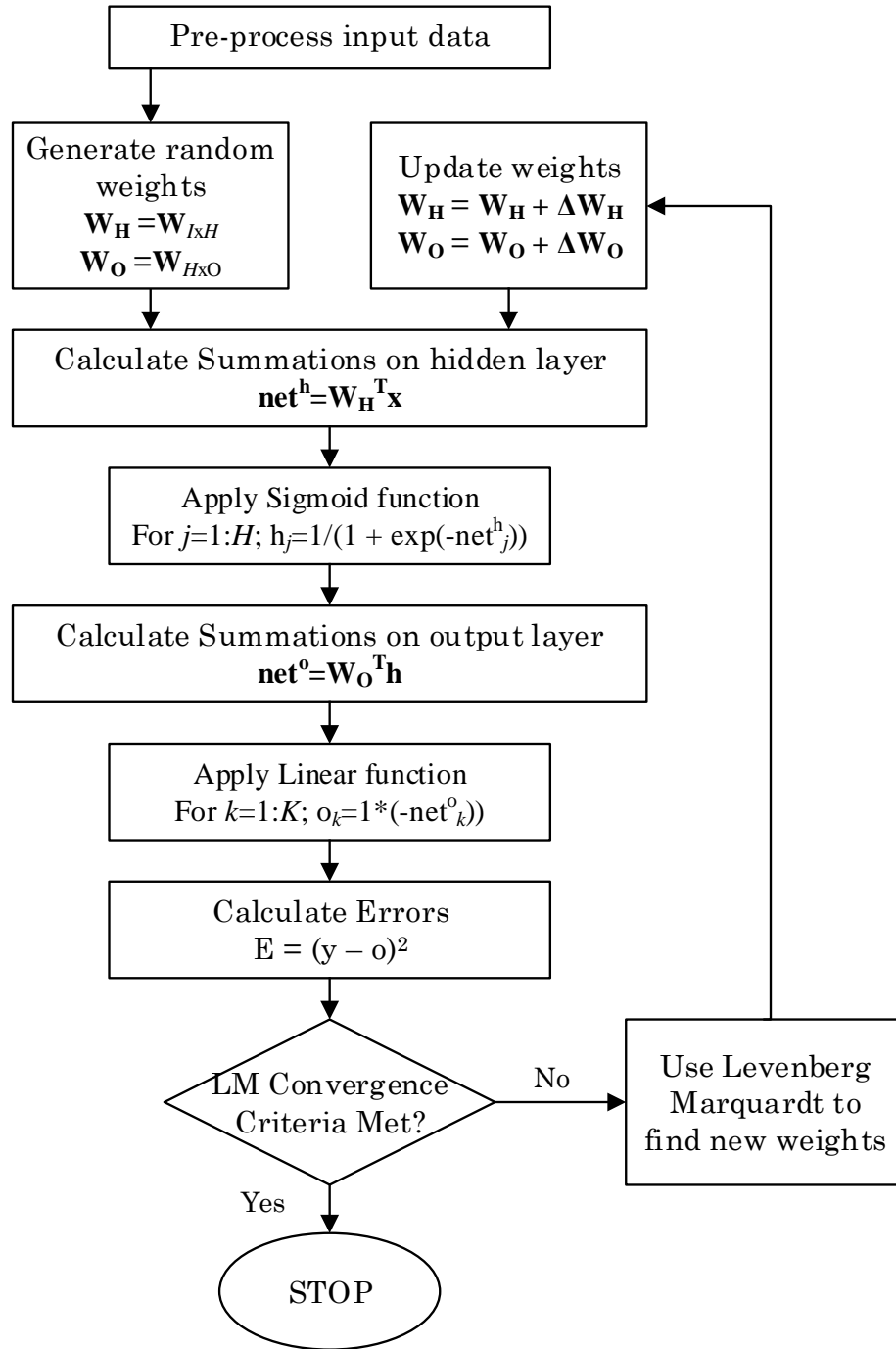
Figure 7 – Flow Diagram of the ANN Algorithm
