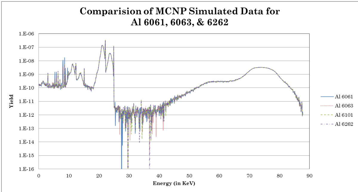
Figure 22 – MCNP Data for Al-6061, Al-6063, Al-6101, and Al-6262
