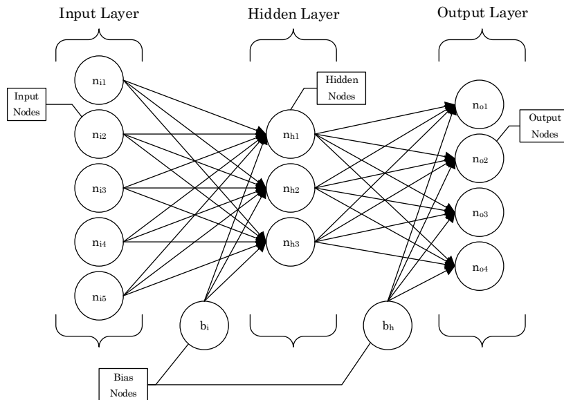
Figure 2 – Typical Structure of a Feed-Forward Neural Network
