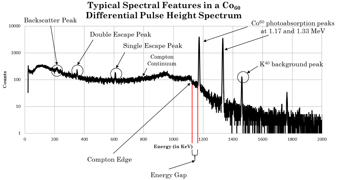
Figure 1 – Typical Features seen in a Gamma Spectra of Co-60
