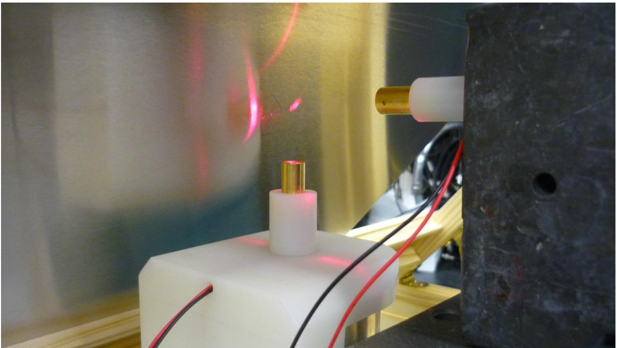
Figure 14 – Experimental setup with laser dots aligned on the metal surface
