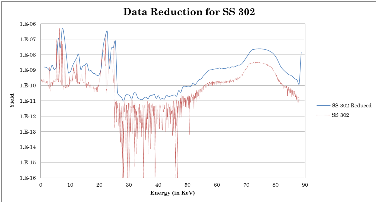
Figure 19 – Reduction of SS 302 data from 1024 channels to 128 channels
