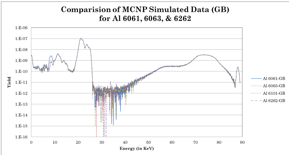
Figure 25 – MCNP Data for Al-6061, Al-6063, Al-6101, and Al-6262
