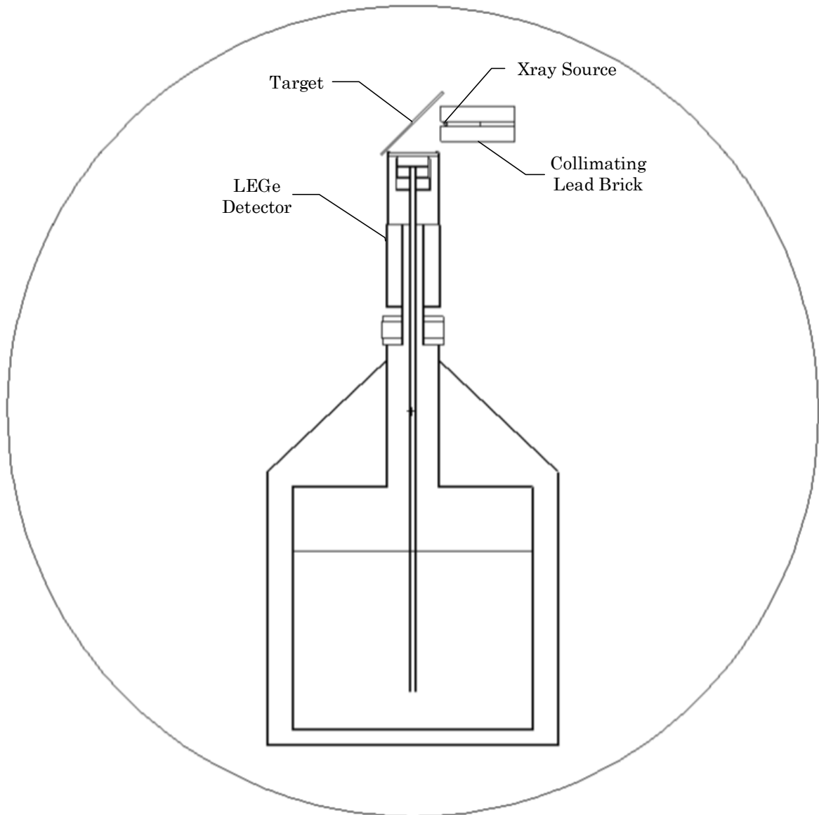
Figure 8 – MCNP Model of a LEGe Detector, Metal Target, Cd-109 X-ray Source, and Lead Collimator
