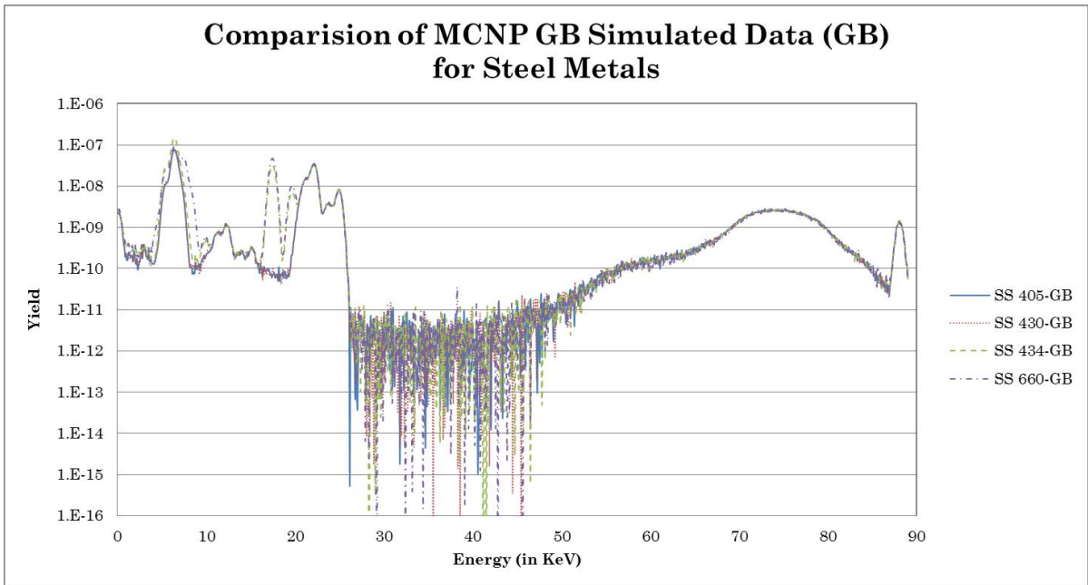
Figure 31 – Gaussian broadened MCNP Data for Stainless Steel 405, 430, 434, and 660
