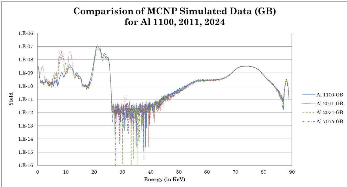
Figure 23 – Gaussian Broadened MCNP Data for Al-1100, Al-2011, Al-2024, and Al-7075
