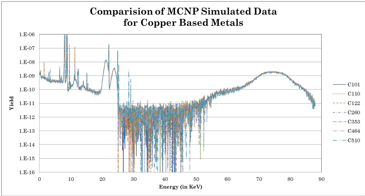
Figure 26 – MCNP Data for C101, C110, C122, C260, C260, C353, C464, C510
