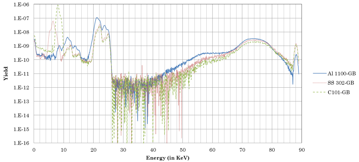
Figure 17 – MCNP Simulated Data (Gaussian Broadened)
