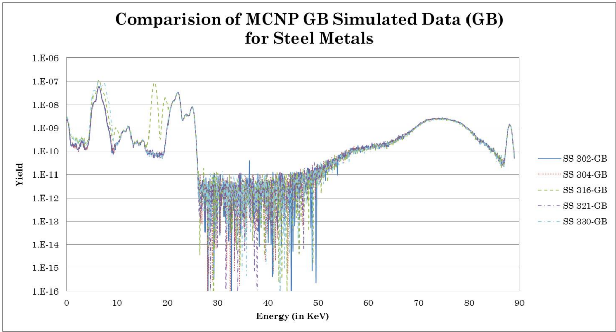
Figure 30 – Gaussian broadened MCNP Data for Stainless Steel 302, 304, 316, 321, and 330
