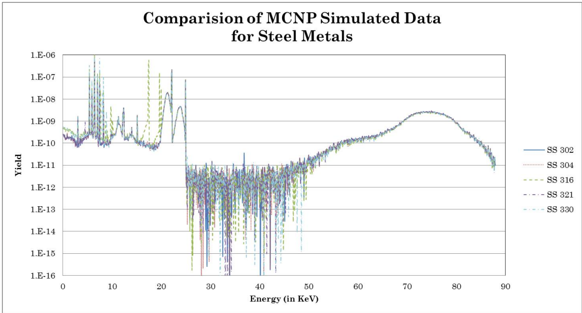
Figure 28 – MCNP Data for Stainless Steel 302, 304, 316, 321, and 330
