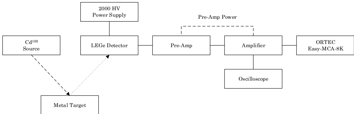
Figure 10 – Block Diagram of the Experimental Setup
