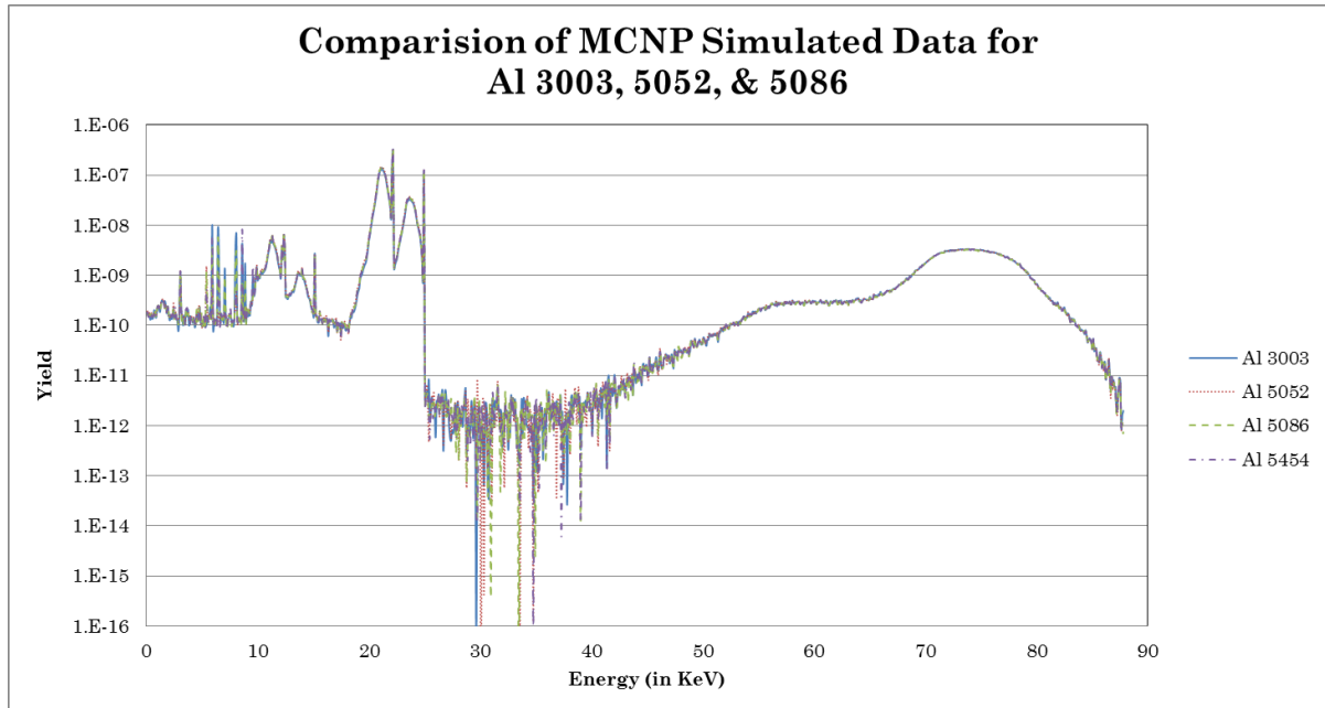
Figure 21 – MCNP Data for Al-3003, Al-5052, Al-5086, and Al-5454
