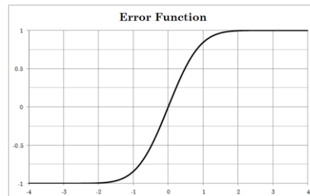
Figure 6 – Error Function
