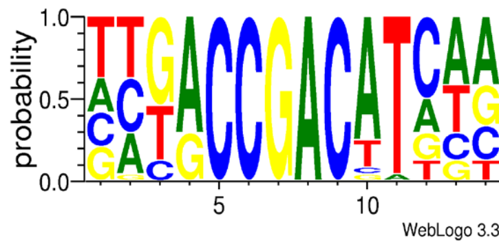
Figure 2: Consensus sequence that contains the C-Repeat/Drought Response Element (CRT/DRE) CCGAC motif was found using the RSAT promoter motif program.
