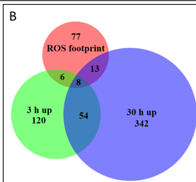
Fig. 4-14: (A) List of genes that act as reactive oxygen species (ROS) scavengers identified in the RNA-Seq data of differentially expressed genes in response to low K + after 3 h and 30 h. Log 2 fc identified with P -value <0.05. List of scavenging genes from Mittler et al. (2004). (B) Output from BioVenn online tool (Hulsen et al. , 2008) used to identify common genes between genes upregulated in response to 3 h or 30 h K + starvation (RNA-Seq data) and genes identified as a ROS transcriptomic footprint (Gadjev et al. , 2006). Gene list (Appendix V).
