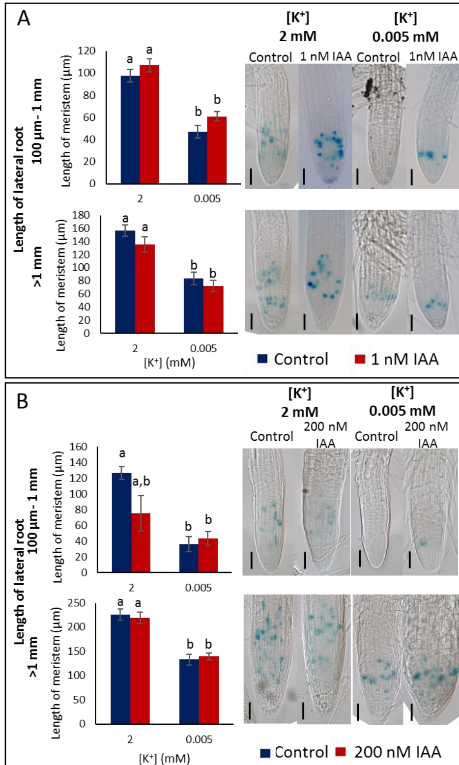
Fig. 5-6: Typical GUS staining pattern of CYCB1;2:GUS ; the staining shows a reduced area of cell division in low [K^+] . Scale bars = 50 \mu M. Average length of meristem measured as the length of area with dividing cells (stained blue in CYCB1;2:GUS line). Media supplemented with either 1 nM IAA (A), or 200 nM IAA (B) for 8 d. Analysis carried out on seedlings 12 d after germination (DAG). Values in histograms are averages of measurements taken from at least 6 individual seedlings per treatment \pm SE, Letters indicate significance with a Tukey Pairwise comparison P < 0.05 .
