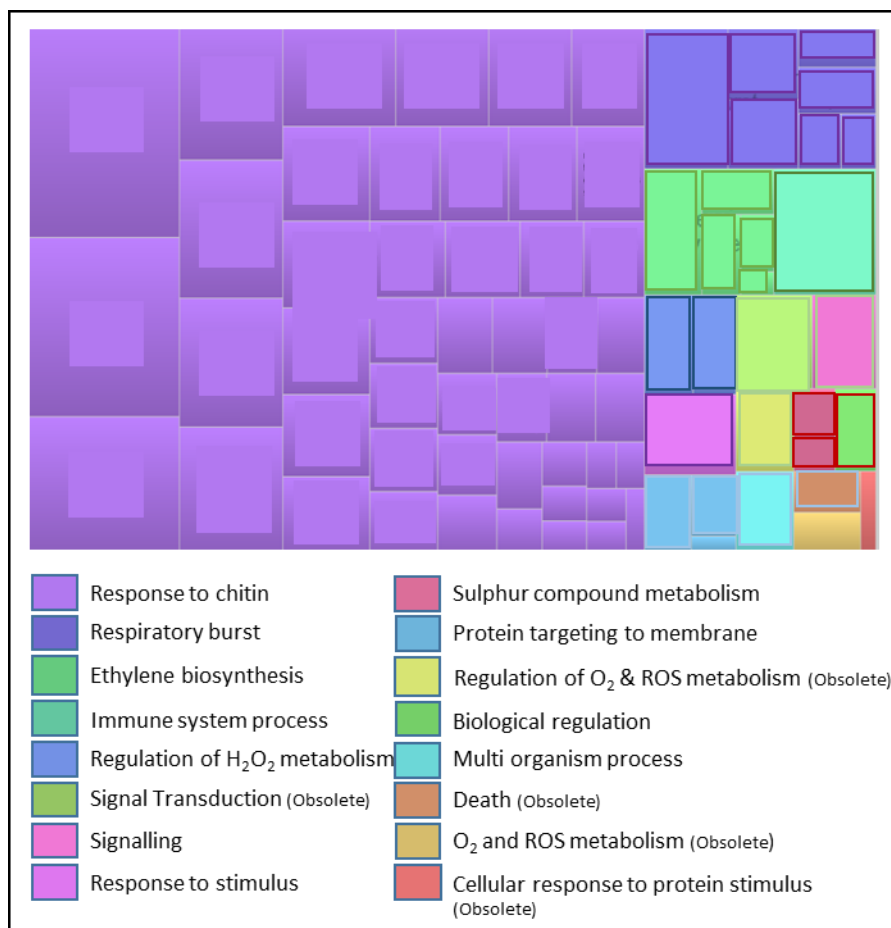
Fig. 4-3: Treemap output from REVIGO (Supek et al. , 2011) of the genes identified as significantly upregulated after 3 h K + starvation, following RNA-Seq experiment. P -value \leq 0.5 and a log 2 fold change (log 2 fc) \geq 0.5 . Each rectangle represents a gene ontology (GO) term cluster and each colour represents a supercluster of related clusters. The superclusters are listed in the key below the treemap. Obsolete terms represent misleadingly named or defined terms. Sizes of rectangles reflect the -\log_{10} P -value of each cluster.
