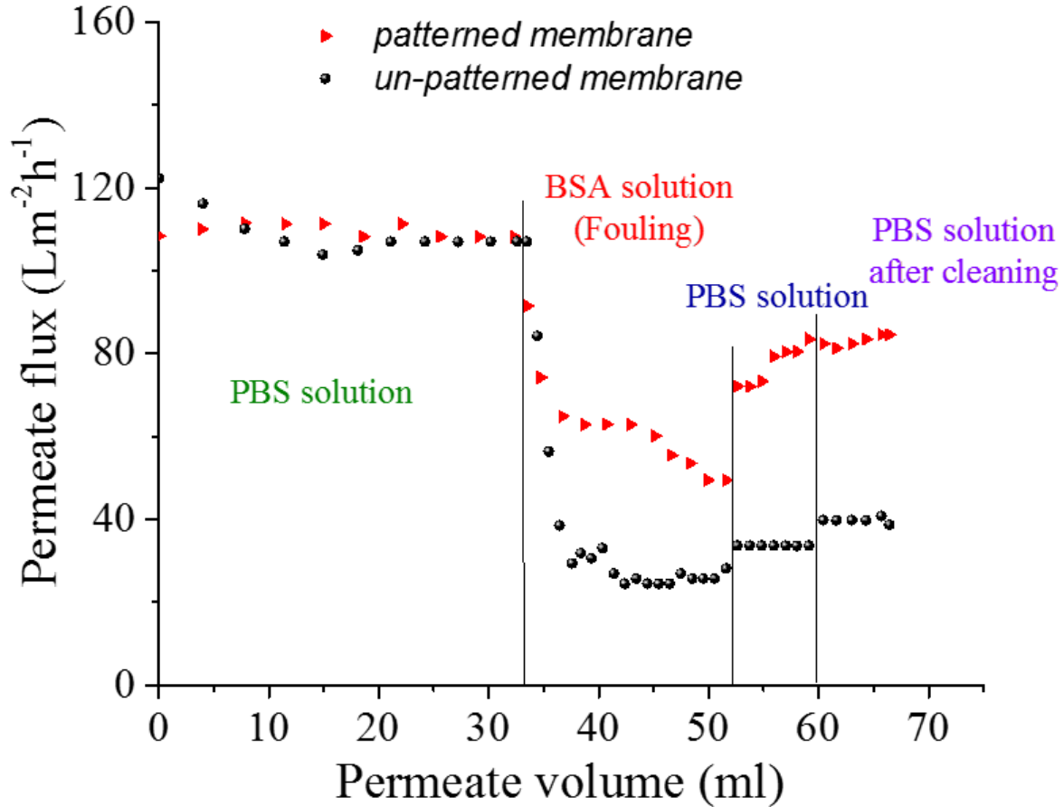
Figure 4.2: Permeate (PBS) flux ( \text{TMP}=276 \text{ kPa} ) versus permeate volume for both un-patterned (circles) and patterned (triangles) membranes during filtration stages 3–6 as specified in Fig. 4.1
