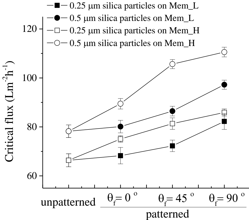
Figure 3.13: Critical flux for un-patterned and two patterned UF membranes at different flow configurations, for 0.25 \mu\text{m} and 0.5 \mu\text{m} aqueous silica suspensions (both at 5g/L). The cross-flow velocity is 0.03 \text{ms}^{-1} . Error bar represents the standard deviation from three replicate measurements.
