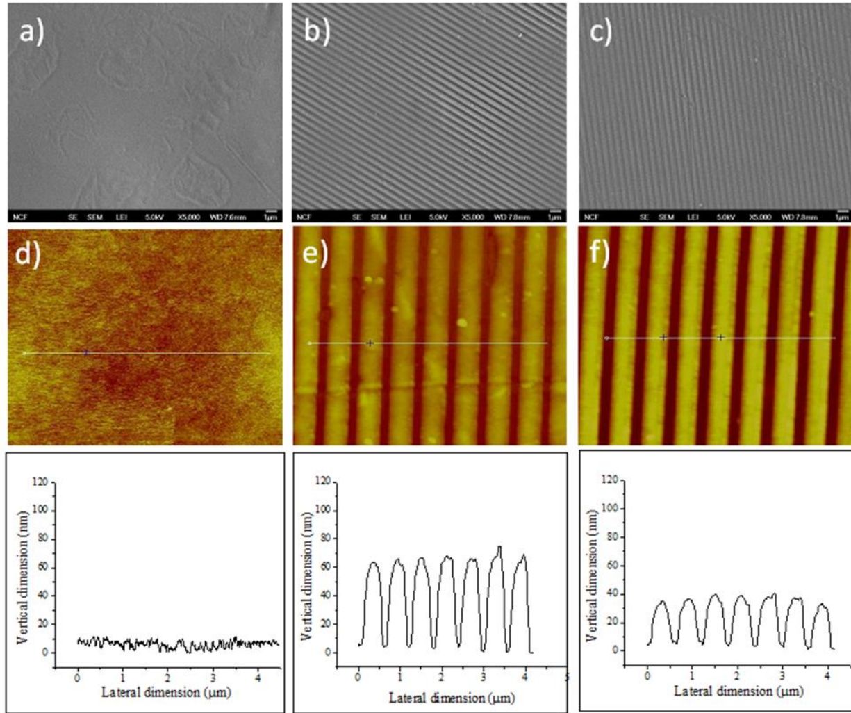
Figure 5.11: Morphological characterization of the un-patterned TFC, patterned UF and Patterned TFC membranes. Representative top-surface SEM images of (a) un-patterned membrane, (b) patterned UF support membrane, (c) patterned TFC membrane. Images (d), (e) and (f) are representative topographic AFM image of un-patterned UF, patterned UF and patterned TFC membranes obtained from AFM scans. The corresponding cross-sectional profiles of both patterned membranes are shown below the AFM images.
