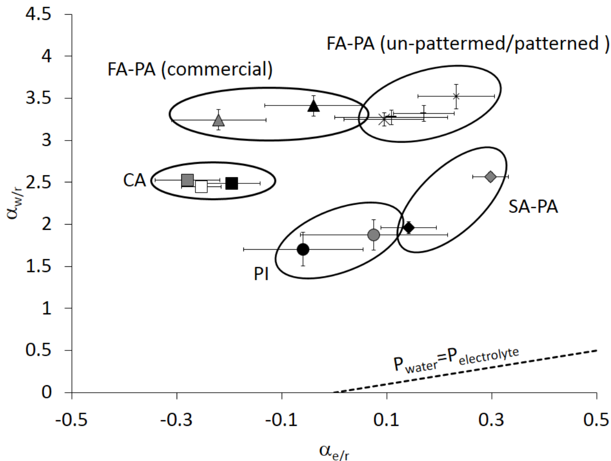
Figure 5.14: Separation factors between water ( w ), glycerol ( r ), and NaCl ( e ) for a variety of polymer material classes. Confidence bars are 90% confidence intervals for three membrane replicates. Adapted from [31]. CA (cellulose acetate), PI (polyimide), SA-PA (semi-aromatic polyamide), FA-PA (fully-aromatic polyamide)
