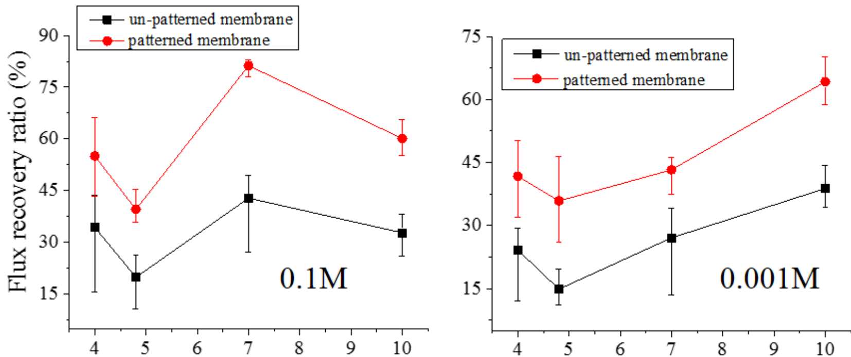
Figure 4.10: PBS flux recovery ratio of the un-patterned and patterned PES membranes as a function of the pH values of the BSA/PBS feed solutions at an ionic strength of (a) 0.1 M and (b) 0.001 M. The error bars represent standard deviations from three replicate measurements.
