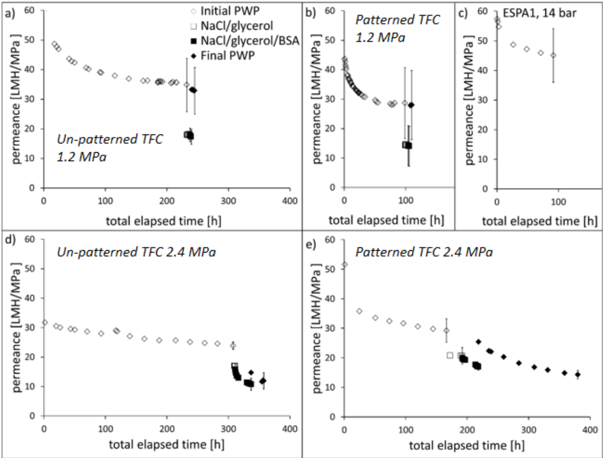
Figure 5.13: Pressure-normalized volumetric flux during un-patterned TFC and patterned TFC experiments at 1.2 and 2.4 MPa. Initial pure water permeance of ESPA1 (a commercial membrane) is also included to compare compaction behavior. Confidence bars are 90% confidence intervals for three membrane replicates. Only confidence intervals for the last marker in each series to reduce clutter was included.
