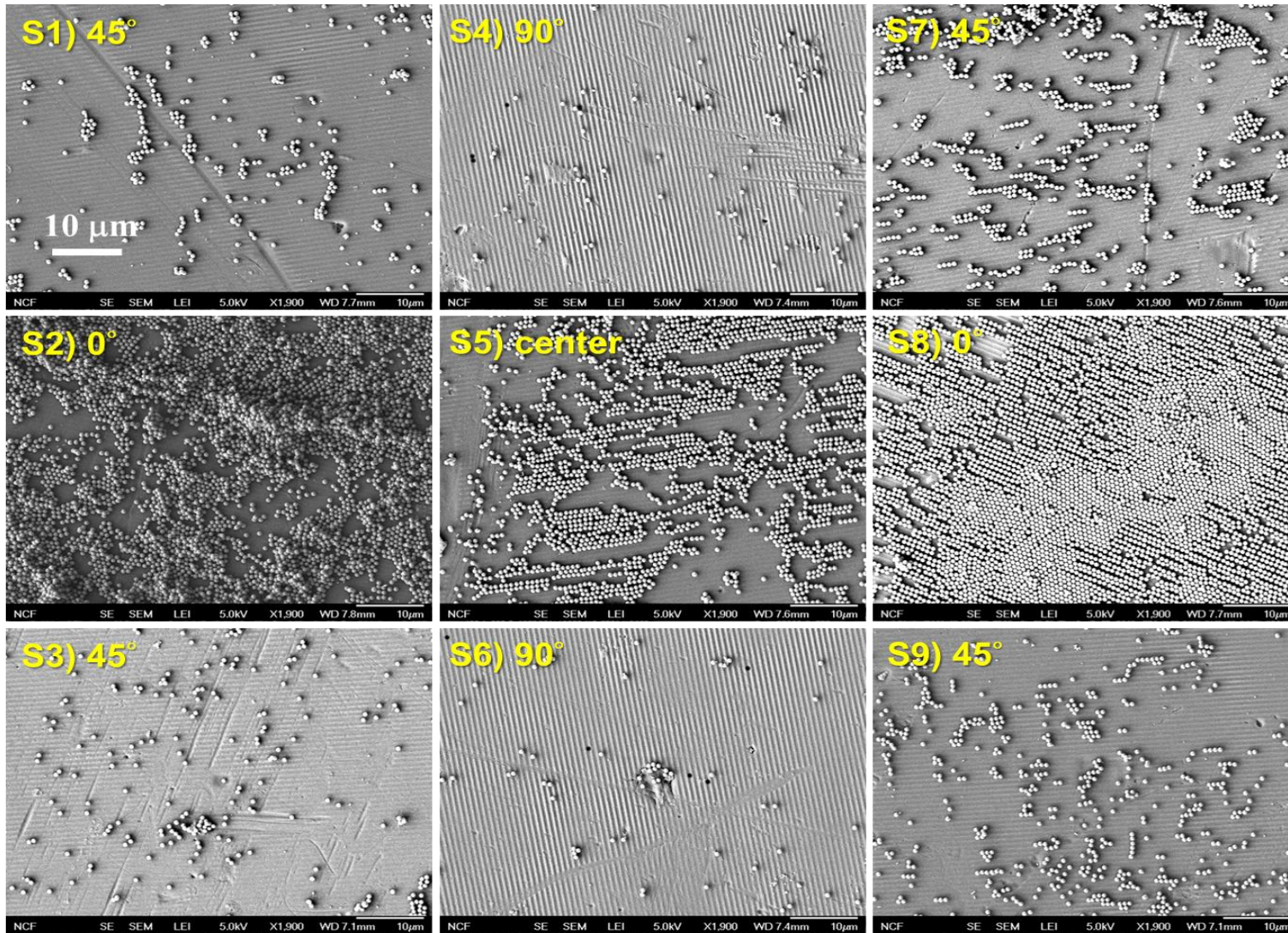
Figure 3.10: SEM images of the fouled patterned membrane at all nine segments of the fouled membrane surface; the average orientation angle of the segment is labeled on each image. The scale bar represents a length of 10 μm.
