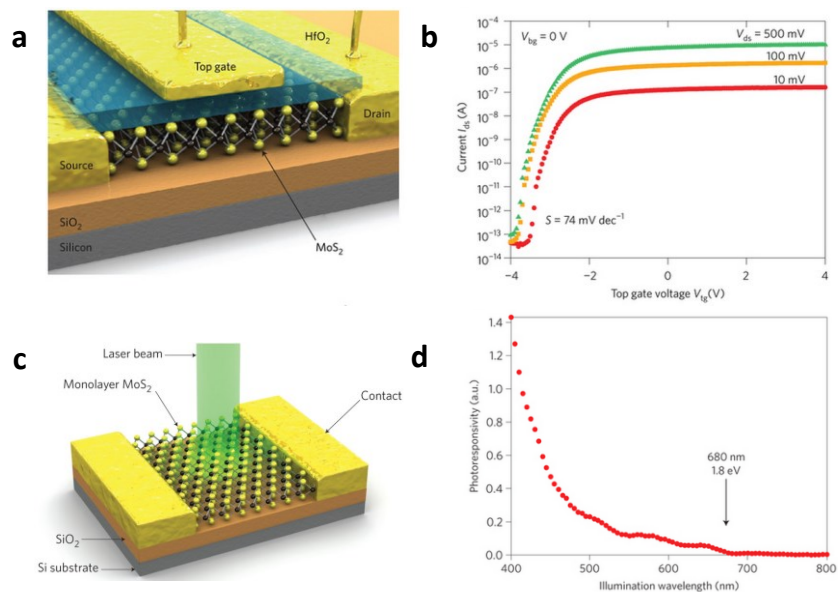
Figure 2.5 a) Schematic of a MoS 2 top gate field effect transistor. b) I_{ds} vs V_g . [44] c) Schematic of a MoS 2 photodetector. d) Photoresponsivity over illumination wavelength. [45]
