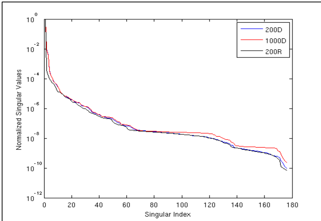
Figure 32: Flux singular values for steady-state and depletion due to cross-section perturbations.
