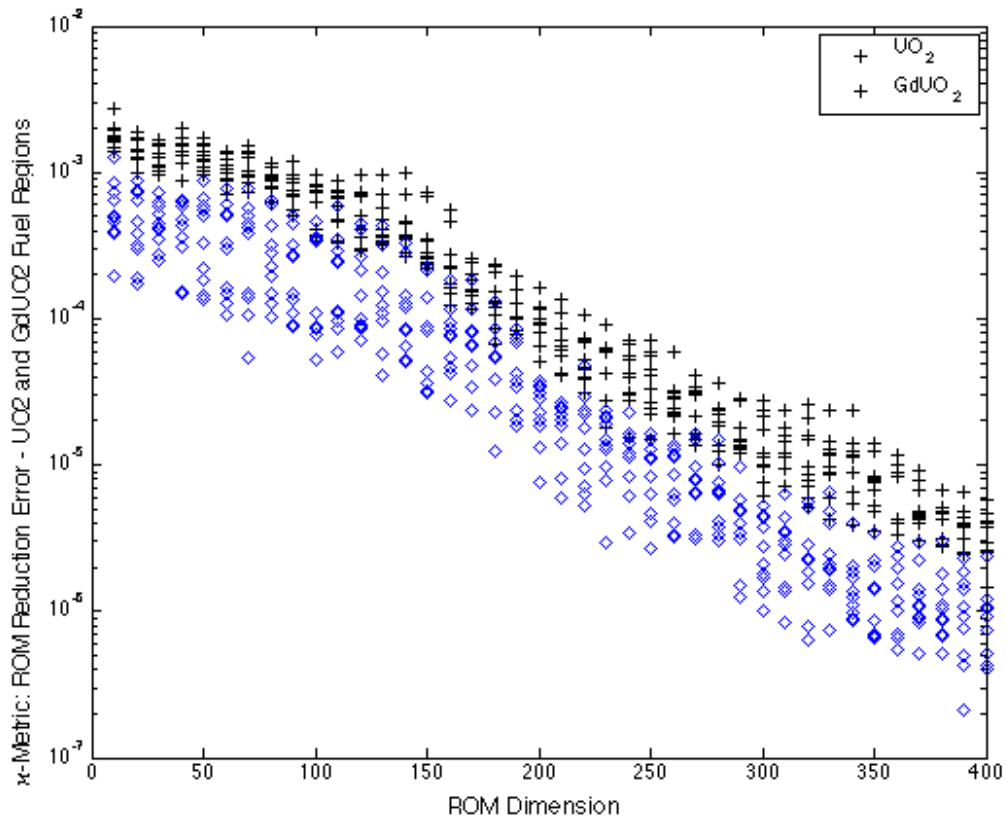
Figure 107: \kappa -Metric of both fuel types (UO 2 and GdUO 2 ) vs. increasing ROM dimension.
