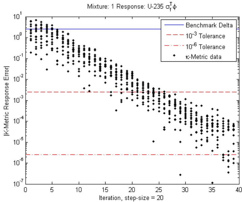
Figure 59: \kappa -metric plot for ^{235}\text{U} fission reaction density in mixture 1.
