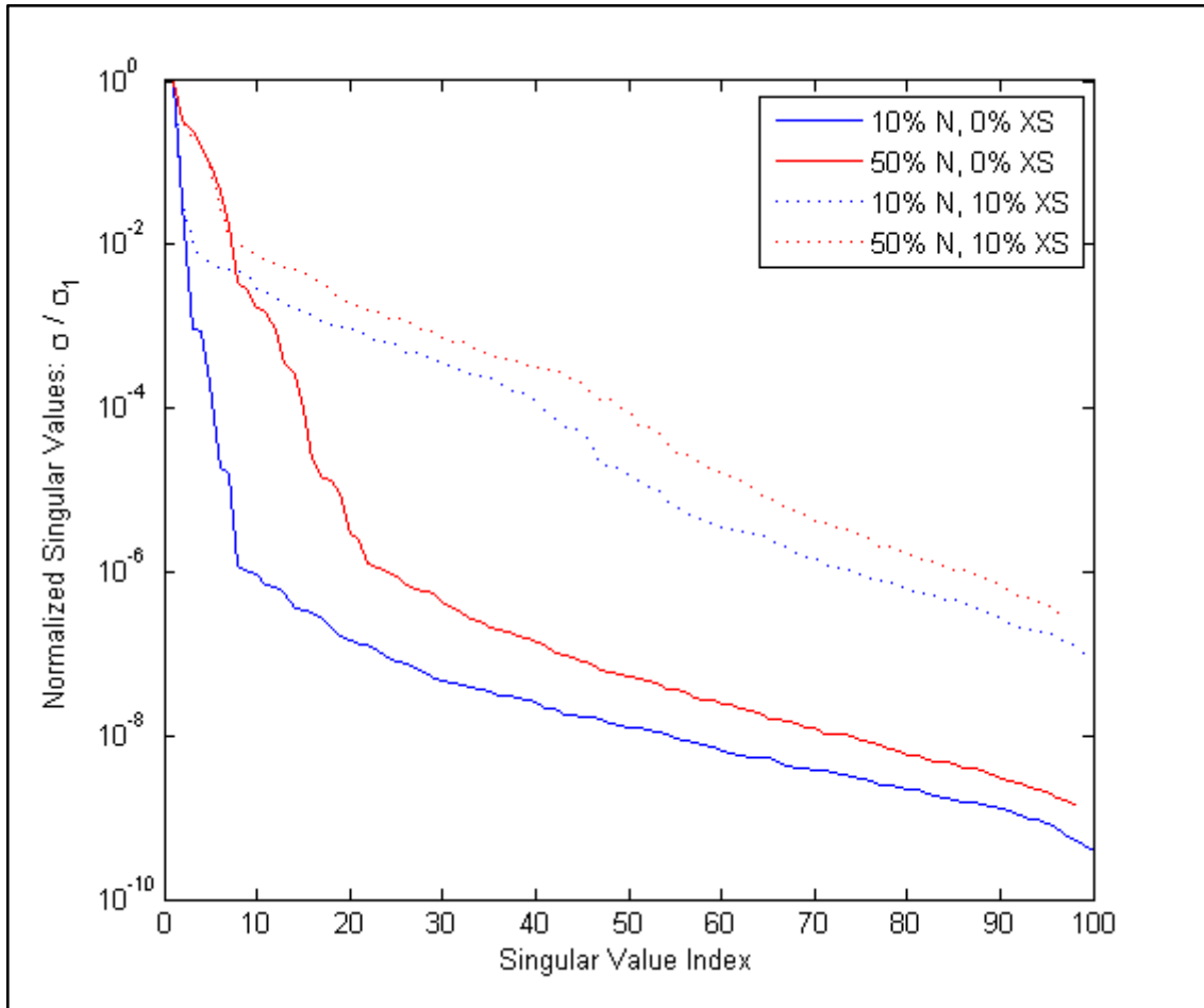
Figure 36: Singular values of sensitivity profiles for nuclide density (N) and cross-section (XS) perturbations of a ^{235}\text{U} enriched fuel pin modeled in TSUNAMI-2D.
