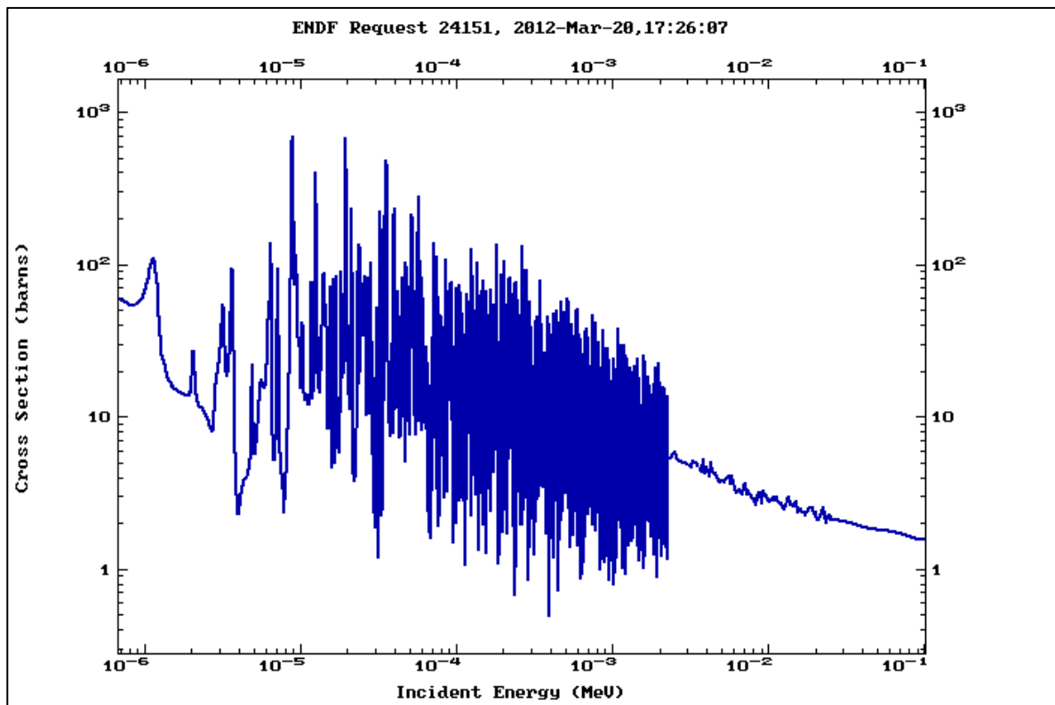
Figure 2: Uranium-235 fission cross-section at 293 o K.
