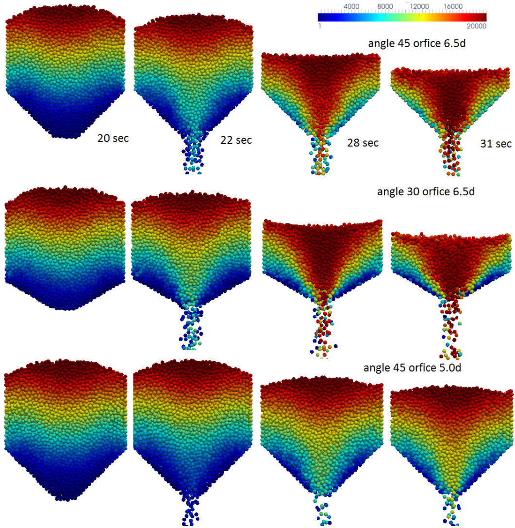
Figure 4.20: Configurations of final particle position distribution at 20 sec and the discharge of the different geometry conditions with the color scale indicating the particle order number
