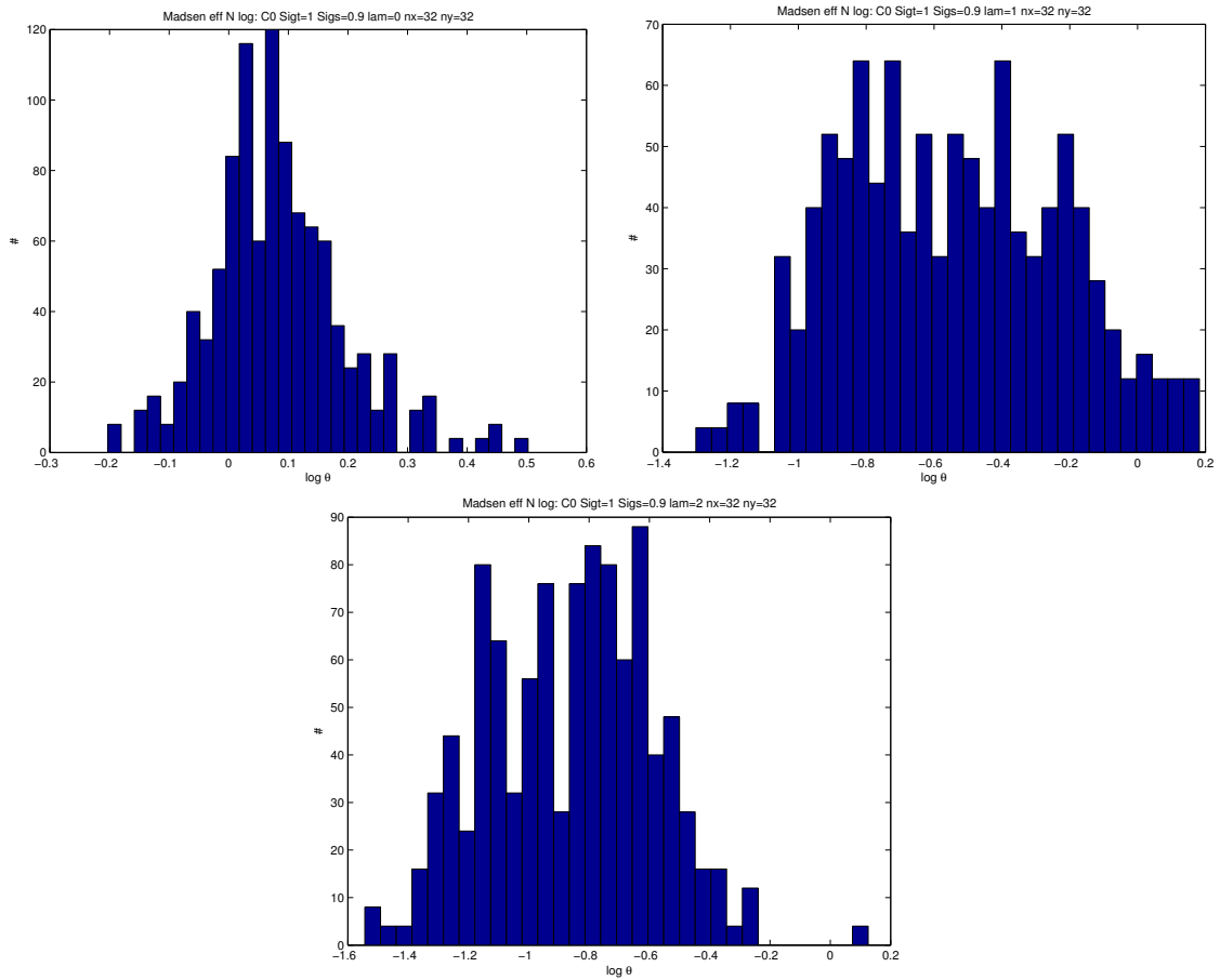
Figure 6.9: Madsen normalized effectivity index: log scale for \text{nx,ny}=32 \sigma_t = 1.0 , C0 and c = 0.1 . Left: \Lambda = 0 , Right: \Lambda = 1 , Bottom: \Lambda = 2 .
