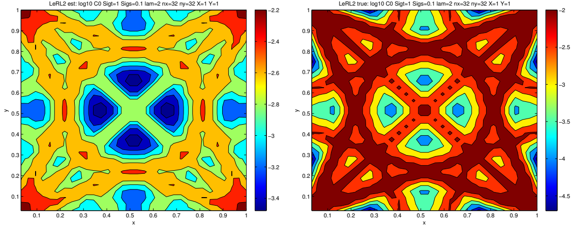
Figure 6.1: Le=R errors: \text{Log}_{10} scale of C0 , \sigma_t = 1 , c = 0.1 and \Lambda = 2 . Left: estimator Right: true error.
