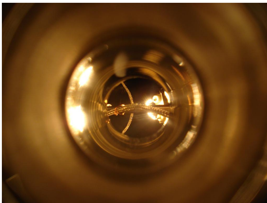
Fig. 4.14. Image displaying filament with 1 A of applied current while the remoderator is within the beamline.
