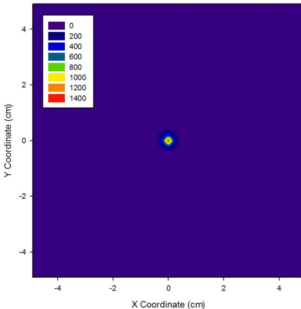
Fig. 6.9. Simulated beam profile of slow positrons emitted from a remoderator foil into a magnetic funnel. The FWHM of the profile is 3.2 mm.
