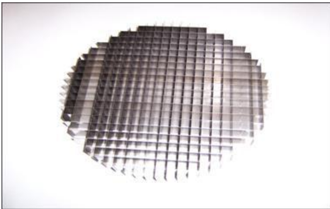
Fig. 2.20. Image of an assembled tungsten vane moderator.
