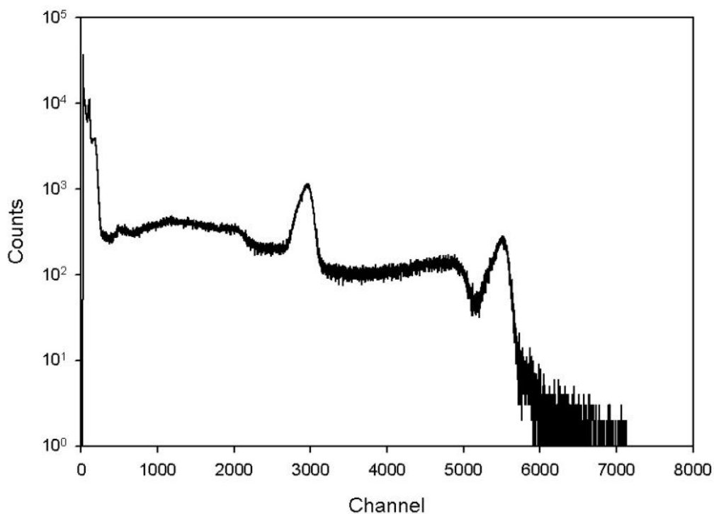
Fig. 5.4. Energy spectrum for Sodium-22 source placed in the sample holder within the target chamber using a \text{LaBr}_3 detector.
