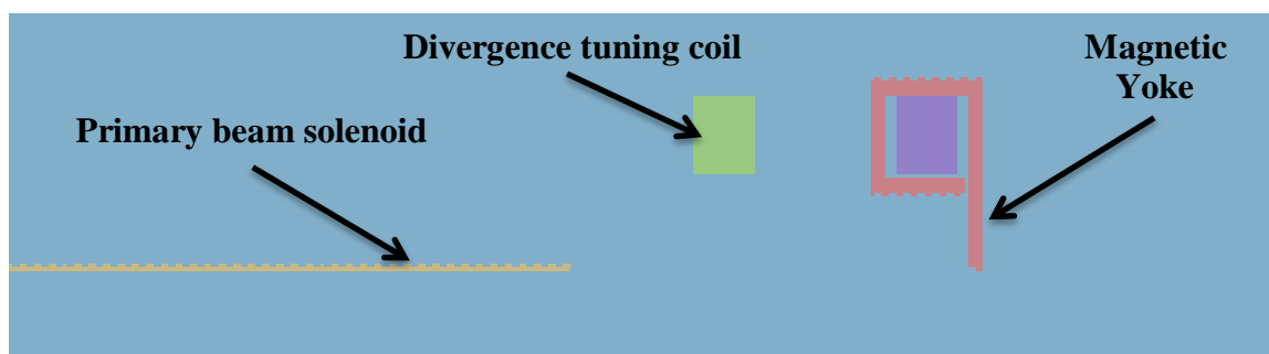
Fig. 6.4. A Tricom model of a 4” ID solenoid followed by a magnetic lens.
