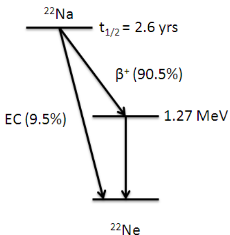
Fig. 5.3. Decay scheme for Na-22.
