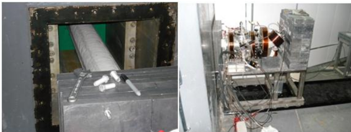
Fig. 3.9. Images of the Second Generation Intense Slow Positron Beam installed in beam tube 6 of the PULSTAR reactor.
