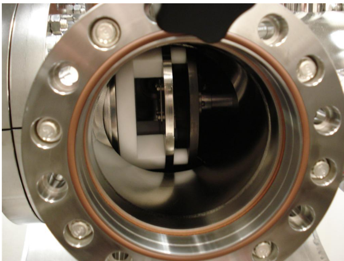
Fig. 4.23. Image of drift lens and sample holder installed in the pulsed positron beam.
