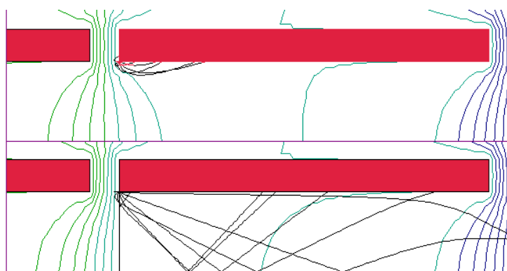
Fig. 2.9. Simulation displaying the effectiveness of grids behind the moderator bank. The top simulation contains no grid. The bottom simulation has a grid at the same potential as the moderator on the right. The first bank is on the left and second (closest to the extraction optics) is on the right.
