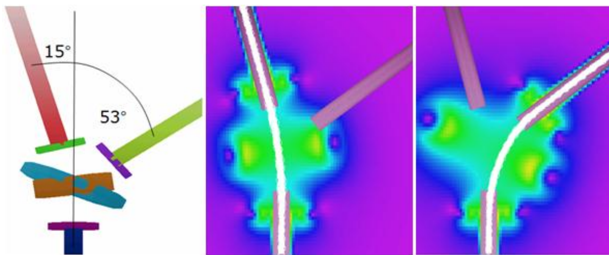
Fig. 2.17. A Schematic of the coil placement for a concept first beam switchyard. This is capable of compensating for particle drifts.
