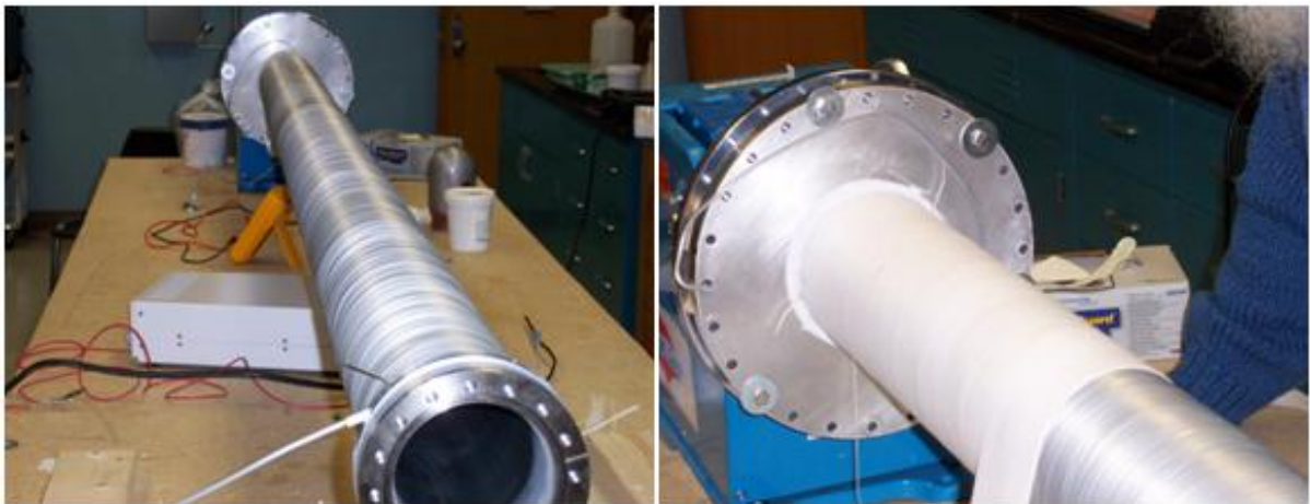
Fig. 2.28. Images taken during the winding of the main solenoid of the slow positron beam.
