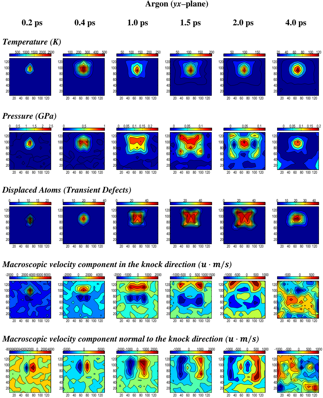
Figure 5.19 The temporal evolution of the spatial fields for Ar in the yx plane. The radiation impact is along the x direction at the center of the plane. E_{PKA} = 100 eV.
