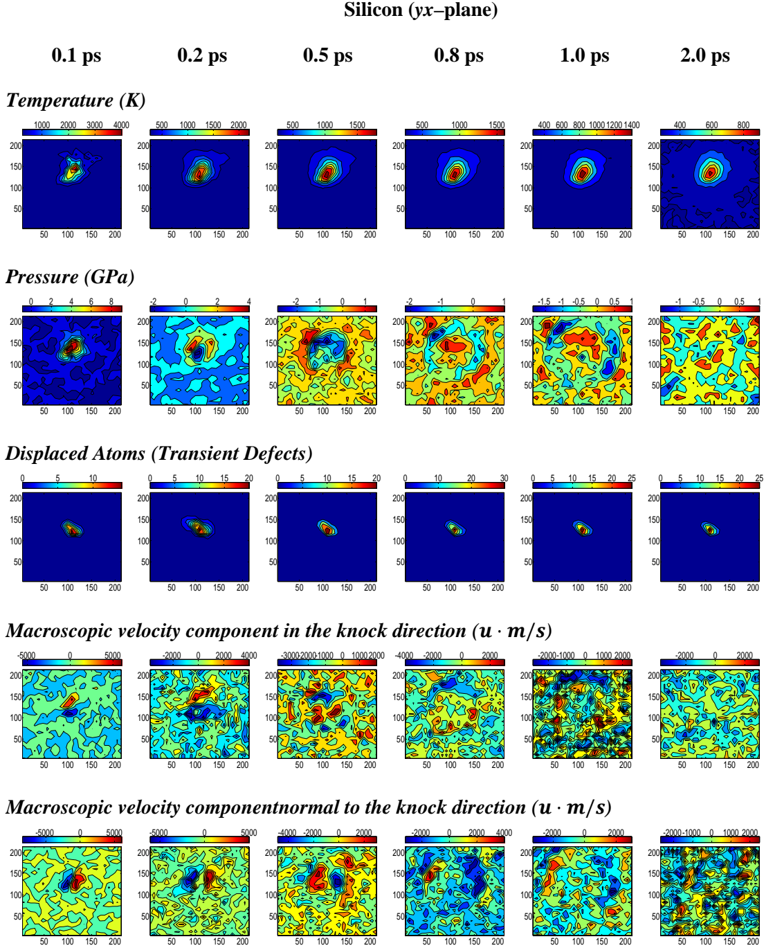
Figure 5.16 The temporal evolution of the spatial fields for Si in the yx plane. The radiation impact is along the x direction at the center of the plane. E_{\text{PKA}} = 3 \text{ keV} .
