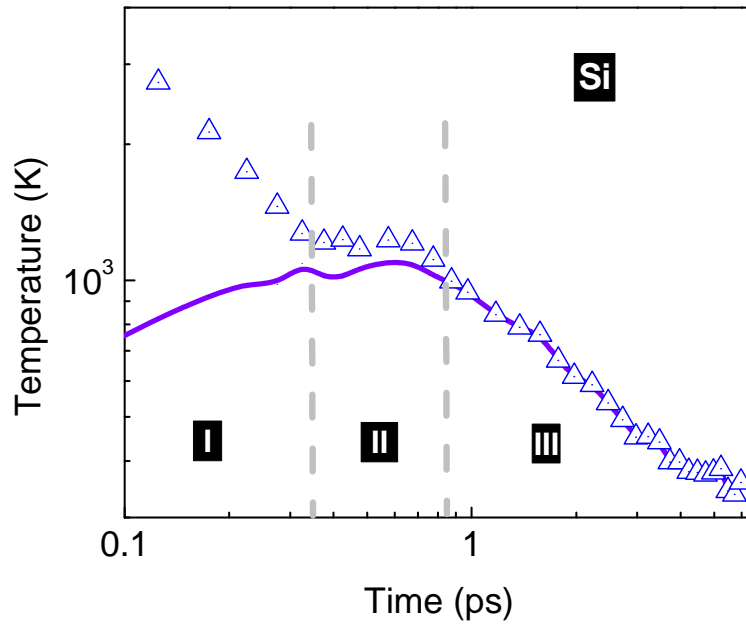
Figure 5.8 Bi-modal temperature variation for Si ( T – line, \Theta – symbol). E_{PKA} = 3 keV.
