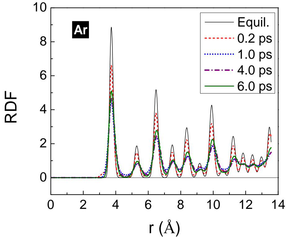
Figure 5.13 RDF of Ar following radiation. E_{\text{PKA}} = 100 eV.
