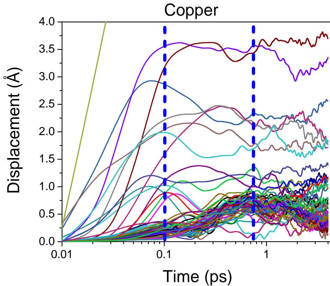
Figure 5.3 Mean displacements of PKA neighbors in copper. E_{\text{PKA}} = 3 \text{ keV} .
