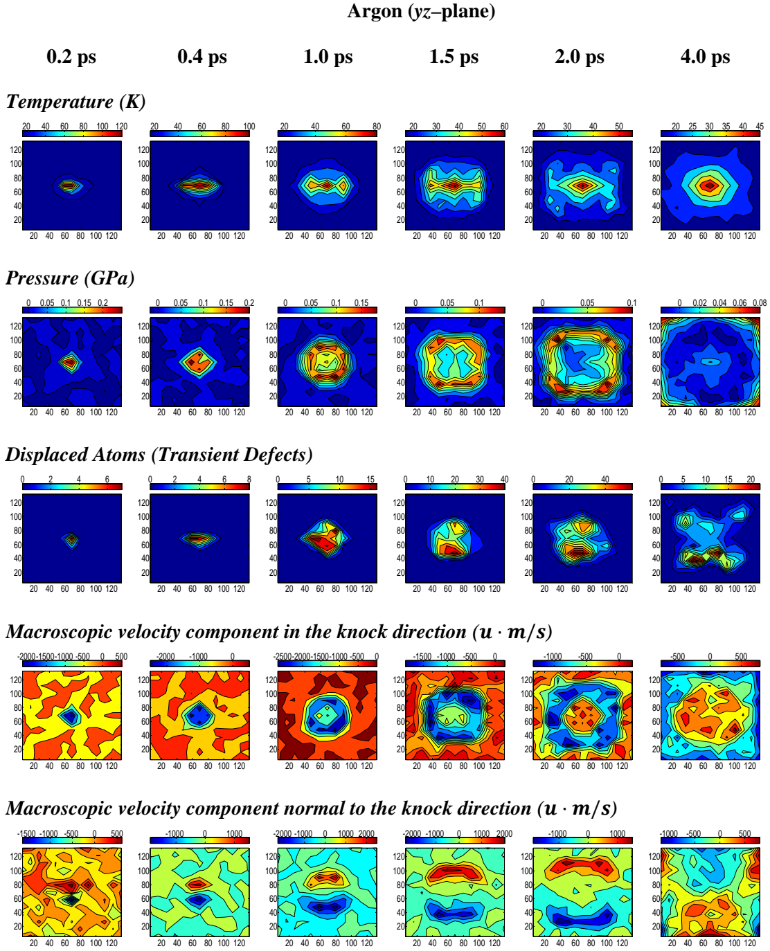
Figure 5.20 The evolution of spatial fields in the yz plane (normal to the knock) for Ar. E_{\text{PKA}} = 100 eV.
