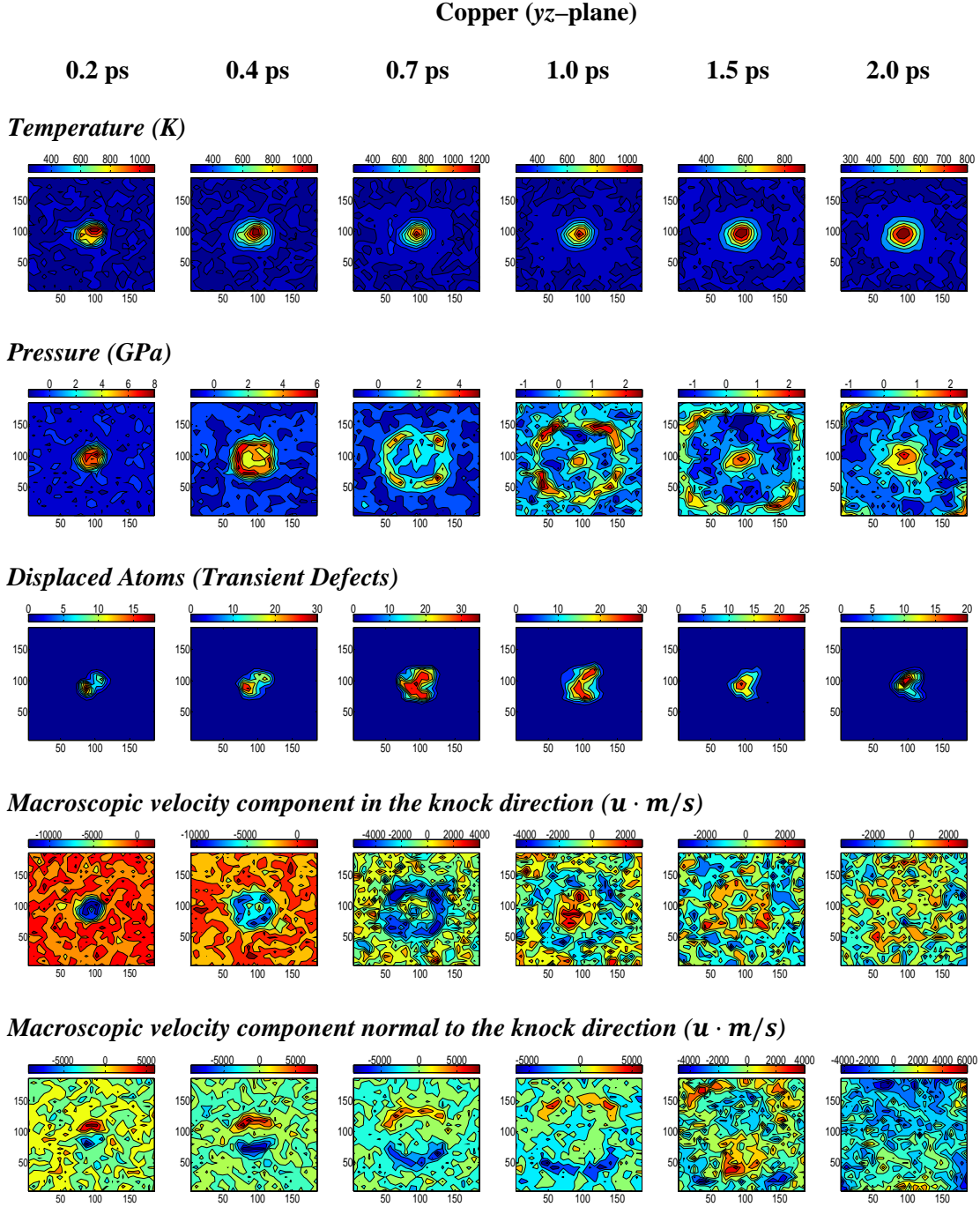
Figure 5.15 The evolution of spatial fields in the yz plane (normal to the knock) for Cu. E_{\text{PKA}} = 3 \text{ keV} .
