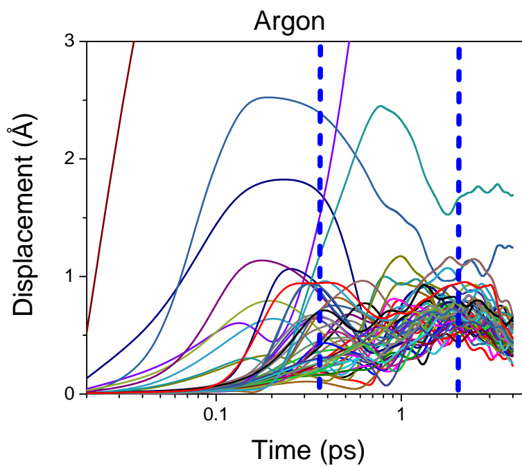
Figure 5.5 Mean displacements of PKA neighbors in argon. E_{\text{PKA}} = 100 \text{ eV} .
