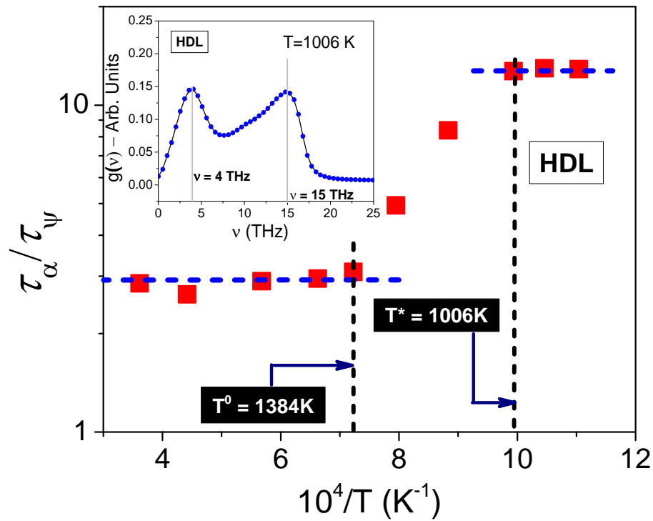
Figure 4.5 The ratio of structural relaxation time with a wavevector of 0.34 \text{ \AA}^{-1} to the viscous relaxation time ( \tau_\alpha/\tau_\psi ) for HDL. (Inset) VDOS for HDL at 1006K showing two prominent frequencies, 4 THz and 15 THz.
