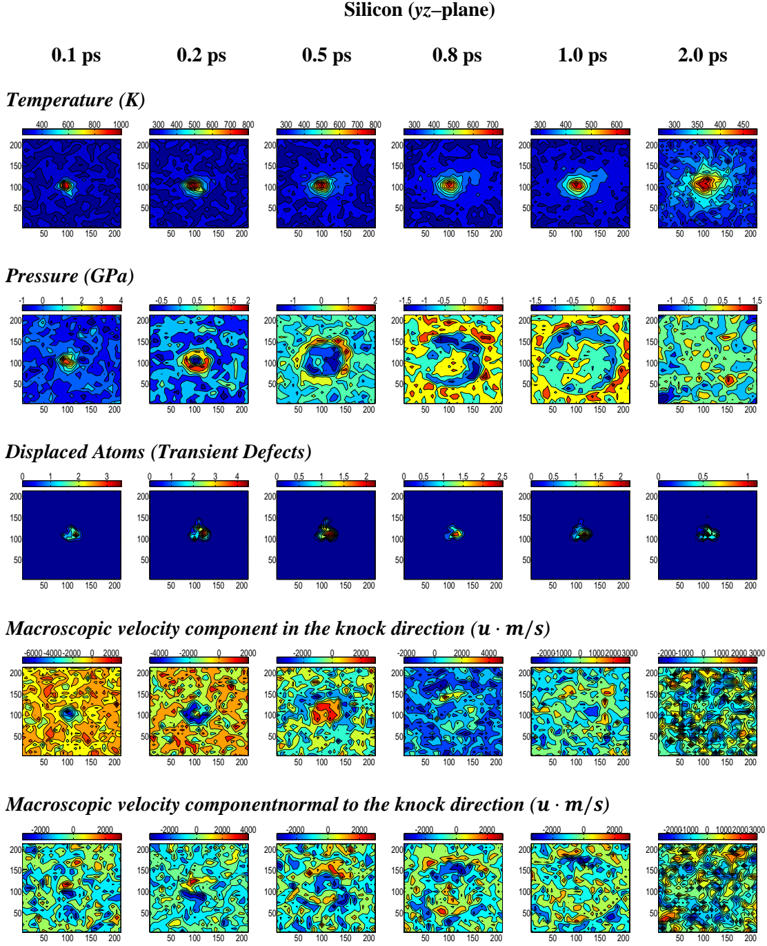
Figure 5.17 The evolution of spatial fields in the yz plane (normal to the knock) for Si. E_{PKA} = 3 keV.
