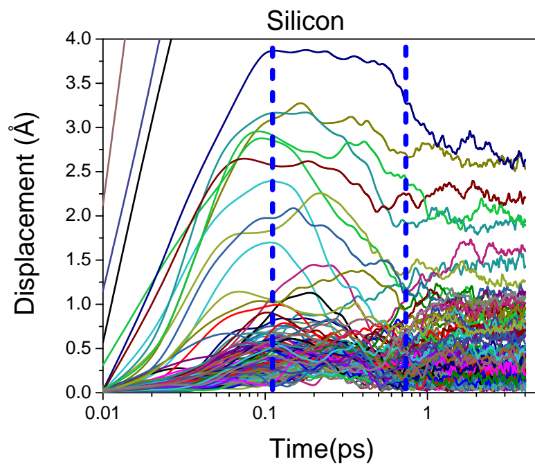
Figure 5.4 Mean displacements of PKA neighbors in silicon. E_{\text{PKA}} = 3 \text{ keV}
