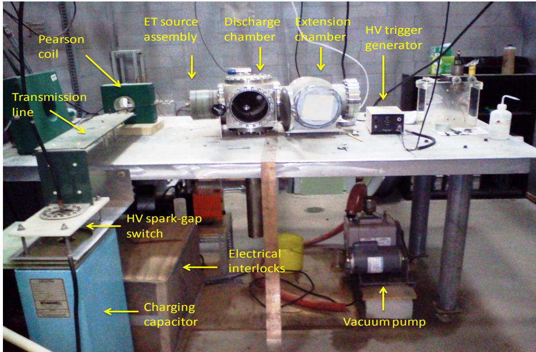
Figure 1.4: A photograph of the PIPE facility.
