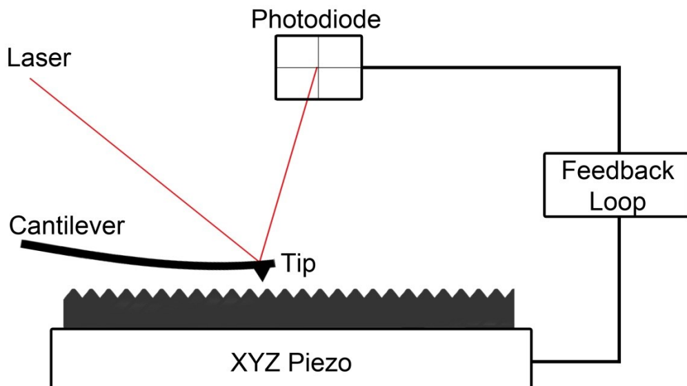
Figure 2.3: Schematic diagram showing the key components of an atomic force microscope.
