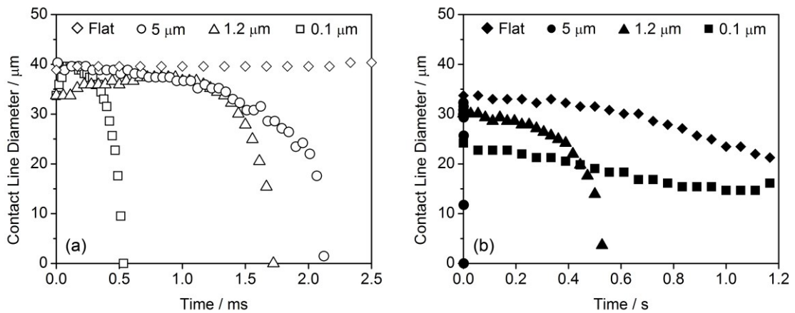
Figure 7.2: Evolution of picolitre droplet (30 \mu\text{m} diameter in air) contact line diameter over time following impact upon: (a) untreated polyethersulfone surfaces (time in ms) and (b) \text{CF}_4 plasma fluorinated polyethersulfone surfaces (time in s).
