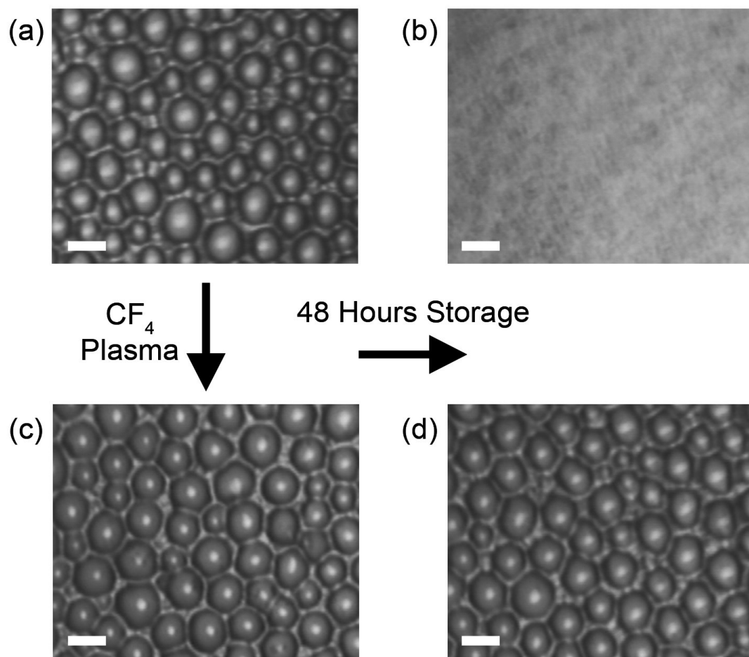
Figure 4.6: Optical microscope images of honeycomb polybutadiene surface: (a) solvent cast; (b) after storage for 48 h; (c) CF 4 plasma treatment of (a) (30 W, 60 s, downstream); and (d) following storage of (c) for 48 h. Scale bar = 50 \mu\text{m} .
