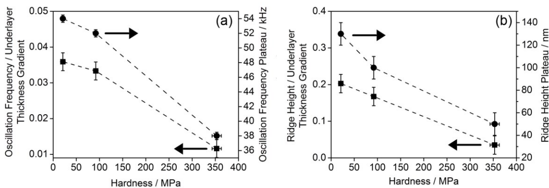
Figure 5.8: Effect of underlayer hardness upon: (a) drop oscillation frequency dependence on underlayer thickness and plateau and (b) surface deformation ridge height dependence on underlayer thickness and plateau after picolitre droplet impact upon 20 nm thick ATRP poly(perfluorooctyl acrylate)* brushes grown from initiator layers with varying underlayer hardness values. * Assuming similar polymer brush densities.
