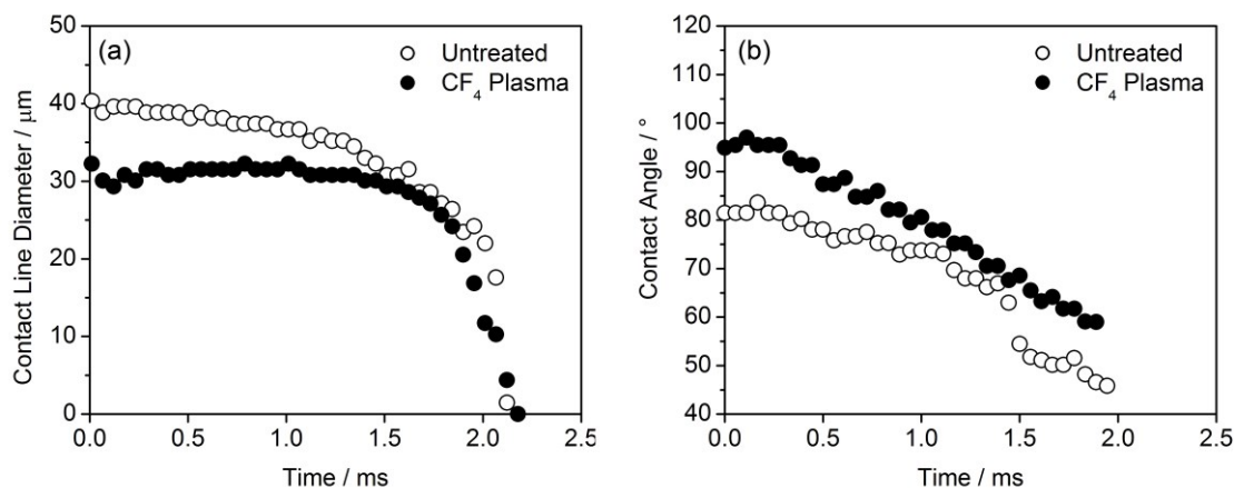
Figure 7.3: Evolution of picolitre droplet (30 μm diameter in air): (a) contact line diameter and (b) contact angle over time following impact upon untreated and CF 4 plasma fluorinated (30 W, 60 s) polyethersulfone membrane surfaces (5 μm pore size).
