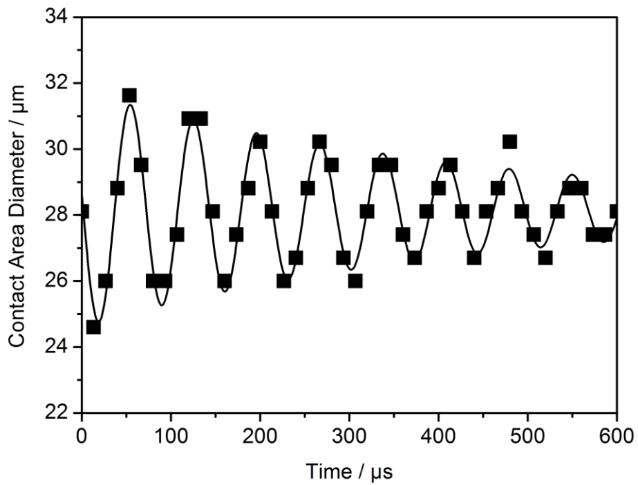
Figure 3.7: Typical damped oscillating curve (Equation 3.6) fitted to the experimental data for picolitre water droplet fluctuation following impact.
