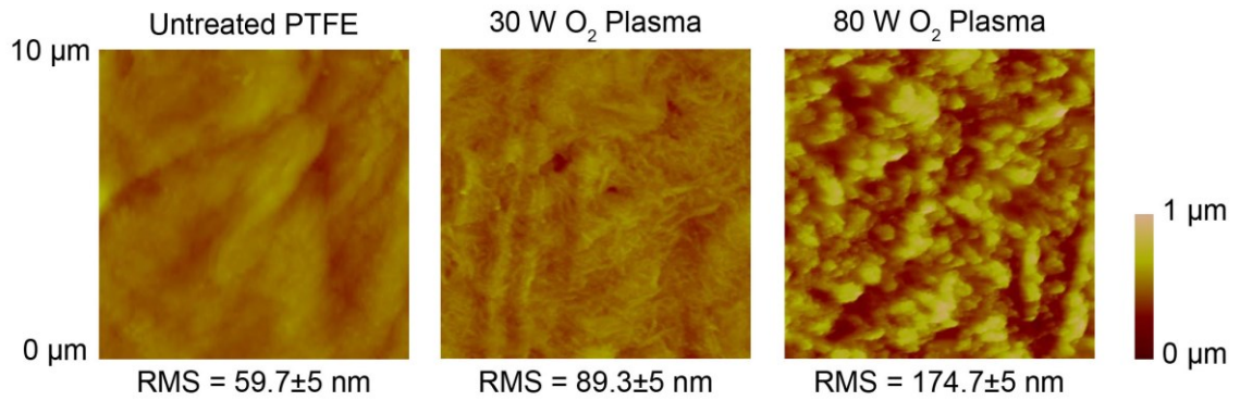
Figure 6.5: AFM images and RMS roughness values for untreated PTFE and O 2 plasma textured PTFE.
