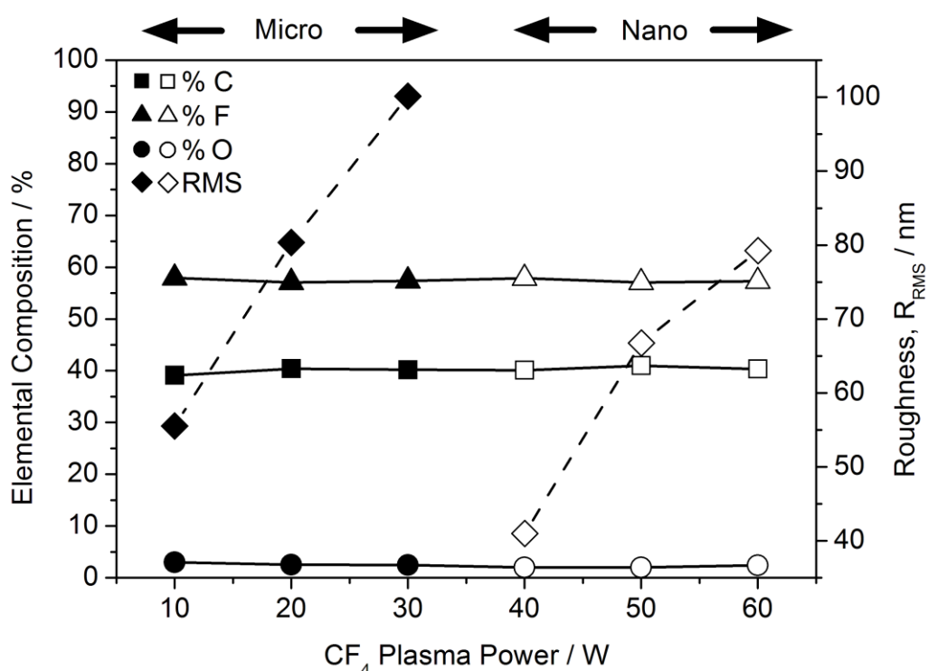
Figure 3.1: XPS and AFM RMS roughness analysis following 5 min \text{CF}_4 plasma fluorination of polybutadiene surfaces as a function of power. The lines are guides to the eye. Closed symbols denote microscale features, and open symbols denote nanoscale features. Error values: Elemental Composition = \pm 2\% ; Roughness, R_{\text{RMS}} = \pm 5 \text{ nm} .
