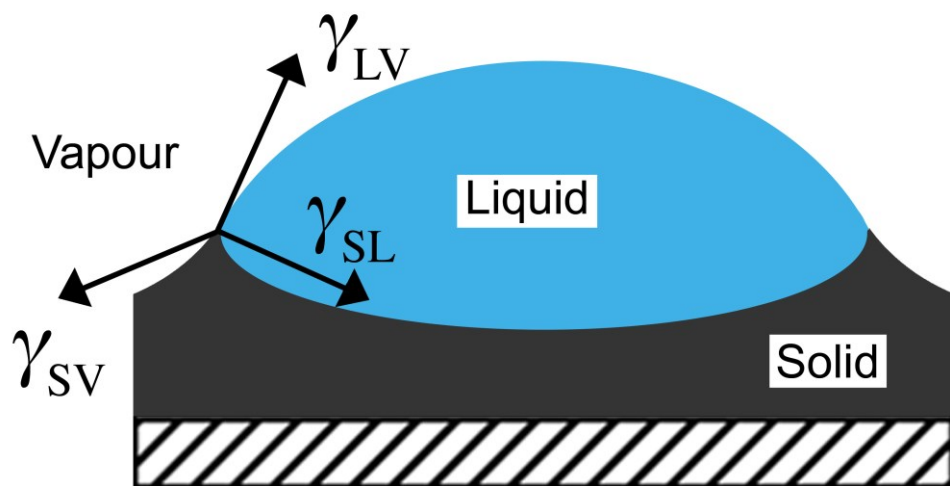
Scheme 5.1: Schematic diagram showing a wetting ridge formed on a soft surface due to the vertical component of the liquid-vapour surface tension, \gamma_{LV} .
