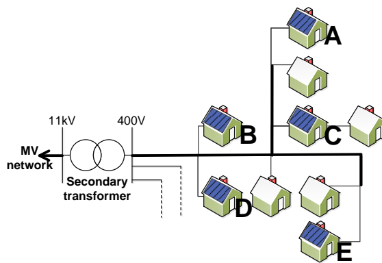
Figure 5-10: An LV network with five feasible locations for home energy storage (labelled A-E)
