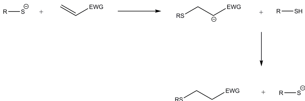
Scheme 1.8 Thiol-ene Michael addition.
