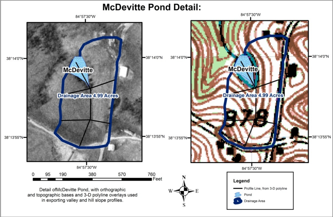
FIGURE 52 - Orthographic and topographic layout of McDevitte pond site.
