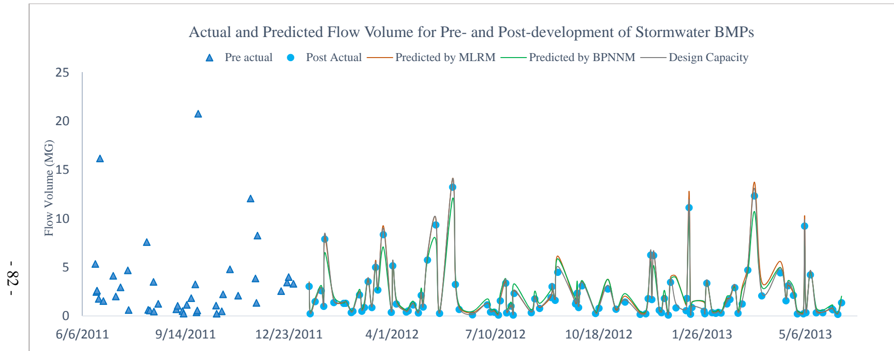
Figure 34 Actual and predicted flow volume for pre- and post-development of stormwater BMPs
