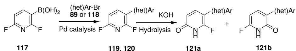
Scheme 74: Two-step synthesis of 3- and 5-((hetero)aryl)-6-fluoro-2-pyridones.
