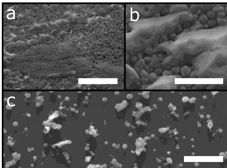
Figure 3.8 TOP : Top images: SEM images of the separated phase formed with the polyHIPE upon curing. Small microdroplets of cured polymer can clearly be seen, along with residue from the emulsion. Lower image: Image shows extracted microdroplets with the soluble residue removed. Scale bars: a ; 20 \mu\text{m} , b ; 5 \mu\text{m} , c ; 10 \mu\text{m}
