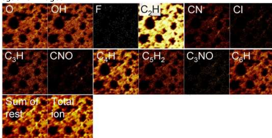
Figure 4.13 ToF-SIMS composite images and corresponding ion assignments for blank polyHIPE (LHS) TOP: positive images. BOTTOM: negative images
