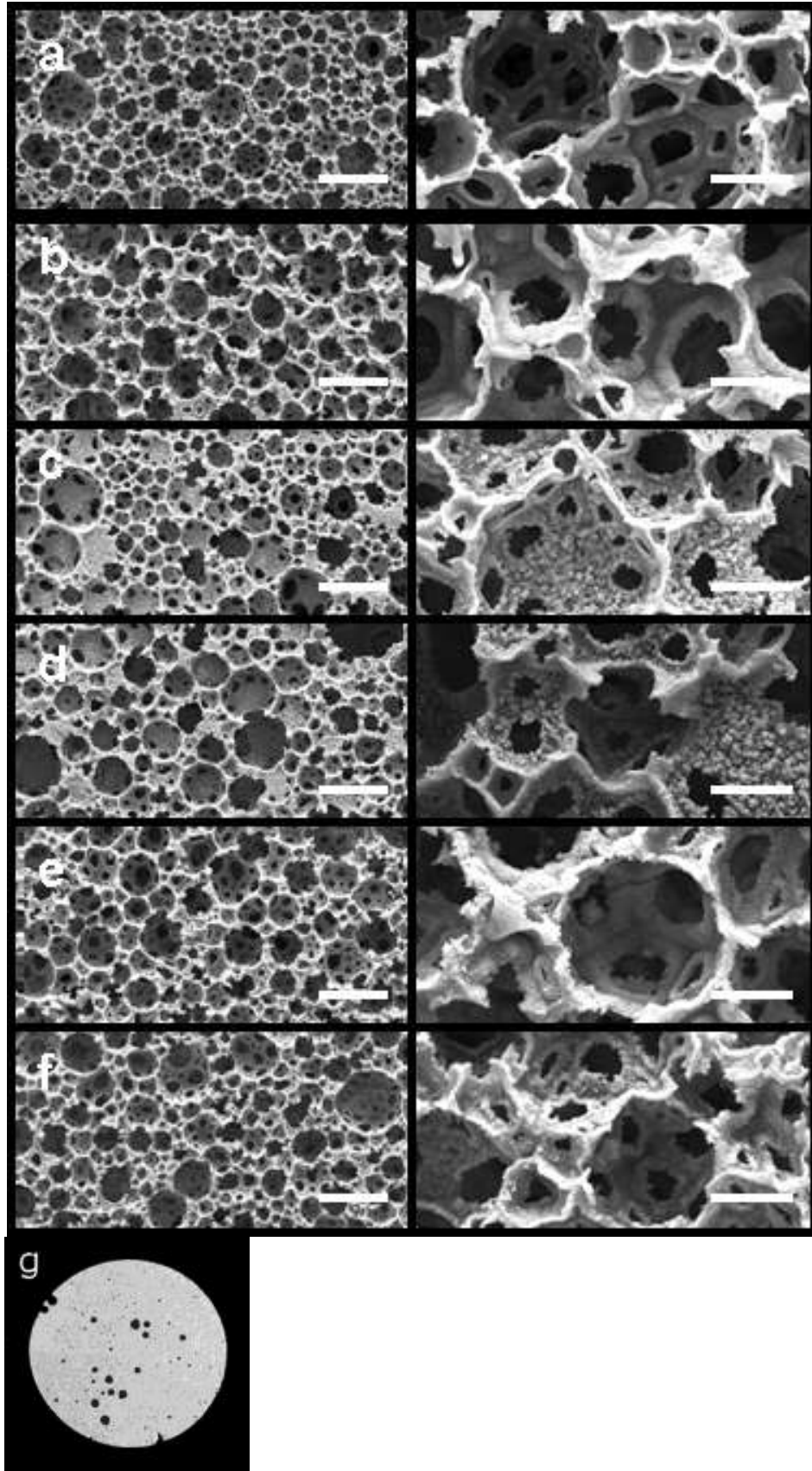
Figure 3.9 a-f: SEM images at 100 x and 500 x magnification. Scale bar LHS 200 \mu\text{m} , RHS, 50 \mu\text{m} . Each row shows the resulting monolith with the following subtleties; a: 10 day old styrene, b: aqueous phase with KPS present left at 80 ^{\circ}\text{C} for 1 hour, c: freshly filtered unrefrigerated monomers, d: inhibitors present (chemicals used as received), e: repeat of "standard conditons": refrigerated filtered monomers used within 24 hours of filtering, aqueous phase/KPS used with no delay f: second repeat as "e". g: photograph of large uneven holes formed through the polyHIPE slice
