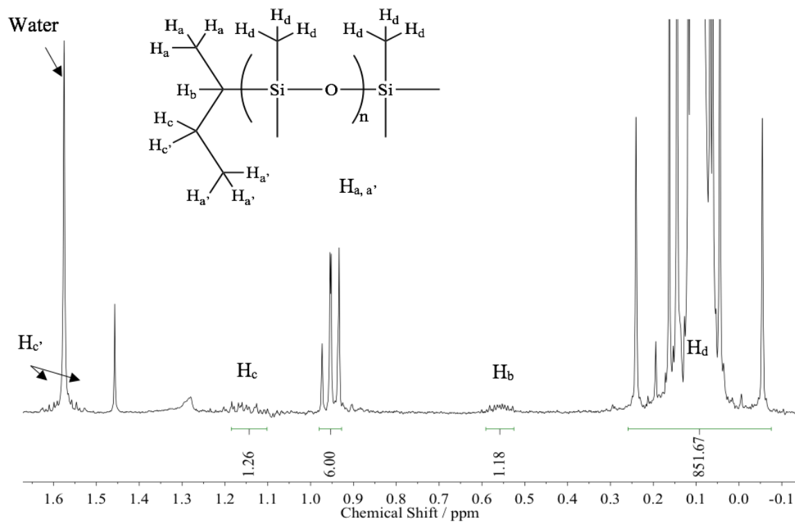
Figure 2.1: The 1 H NMR (CDCl 3 ) spectrum obtained from PDMS 1 after 24 hours.
