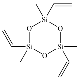
Figure 1.12: 1,3,5-Trivinyl-1,3,5-trimethylcyclotrisiloxane monomer.
